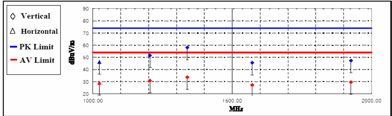
< Fig 6. Radiated emission result (1000MHz ~ 2000MHz)>
