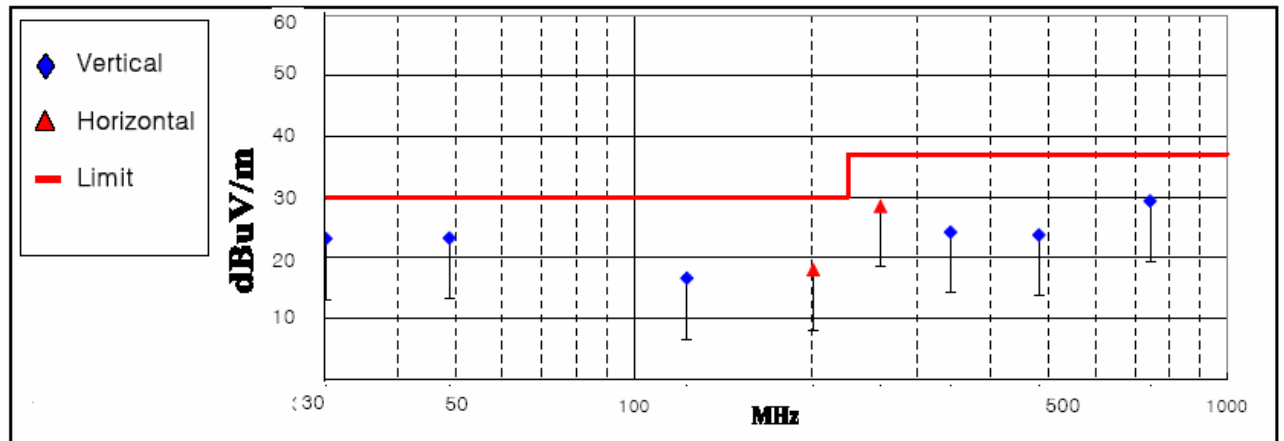
&lt; Fig 8. Radiated emission result (30MHz ~ 1000MHz)&gt;
