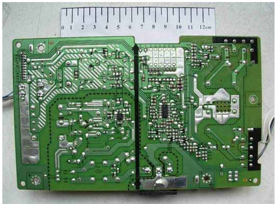
FIGURE 9 LCD MONITOR (M/N: W2340SV) POWER BOARD (SOLDERED SIDE)
