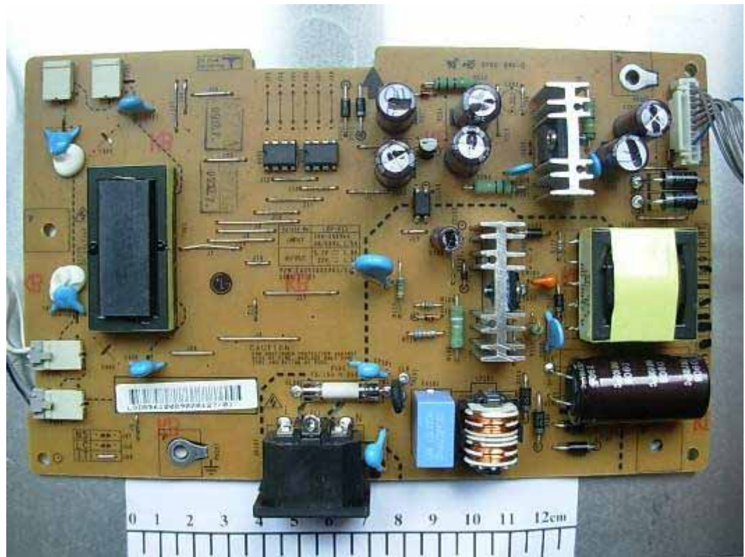
FIGURE 8 LCD MONITOR (M/N: W2340SV) POWER BOARD (COMPONENT SIDE)
