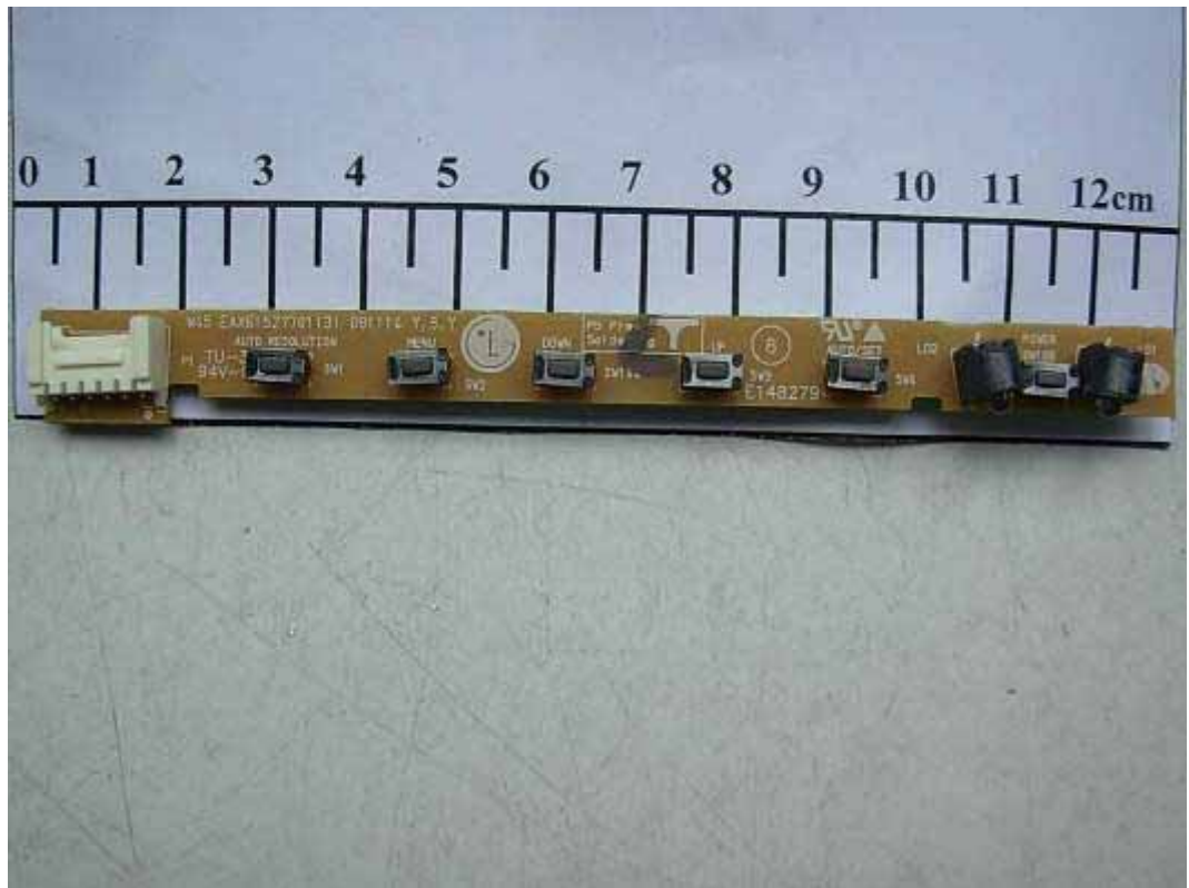
FIGURE 3 LCD MONITOR (M/N: W2340SV) KEYBOARD (COMPONENT SIDE)
