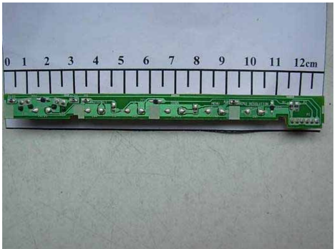
FIGURE 4 LCD MONITOR (M/N: W2340SV) KEYBOARD (SOLDERED SIDE)
