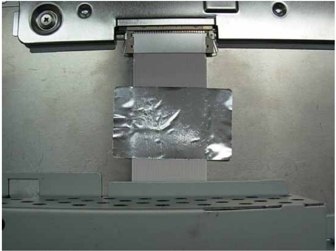
FIGURE 13 LCD MONITOR (M/N: W2340TV) DEBUG
