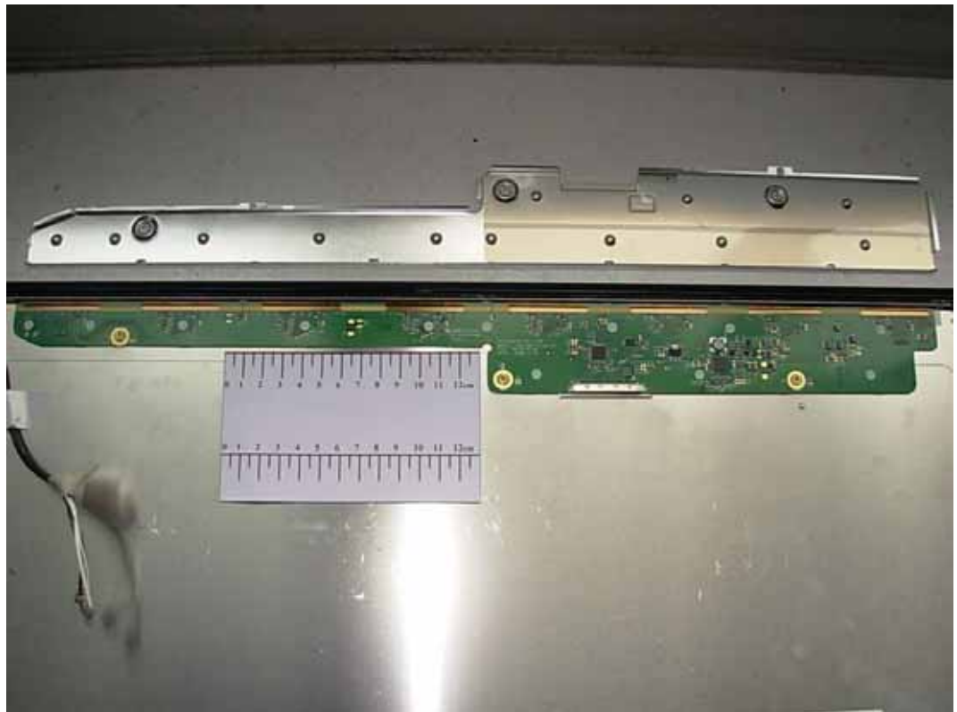
FIGURE 11 LCD MONITOR (M/N: W2340TV) LCD PANEL MAIN BOARD (COMPONENT SIDE)
