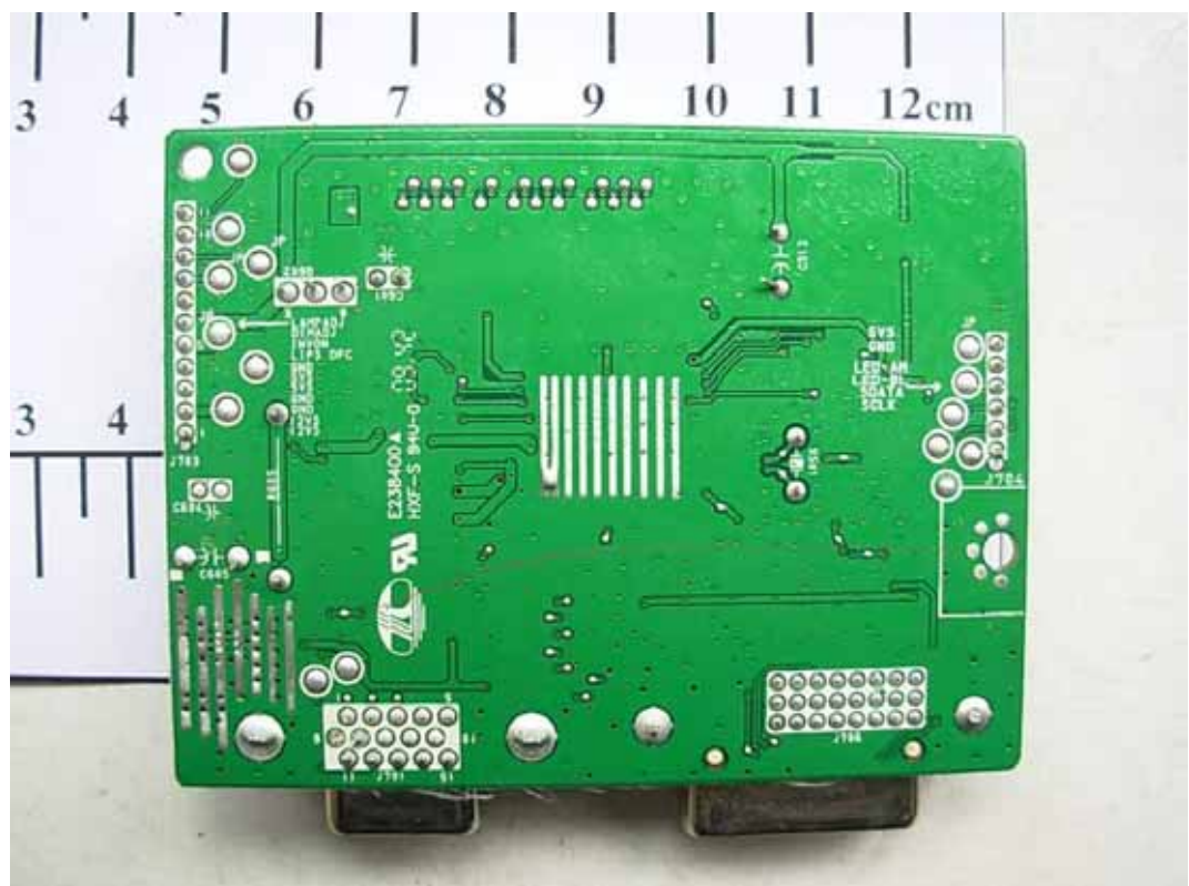
FIGURE 8 LCD MONITOR (M/N: W2340TV) MAIN BOARD (SOLDERED SIDE)
