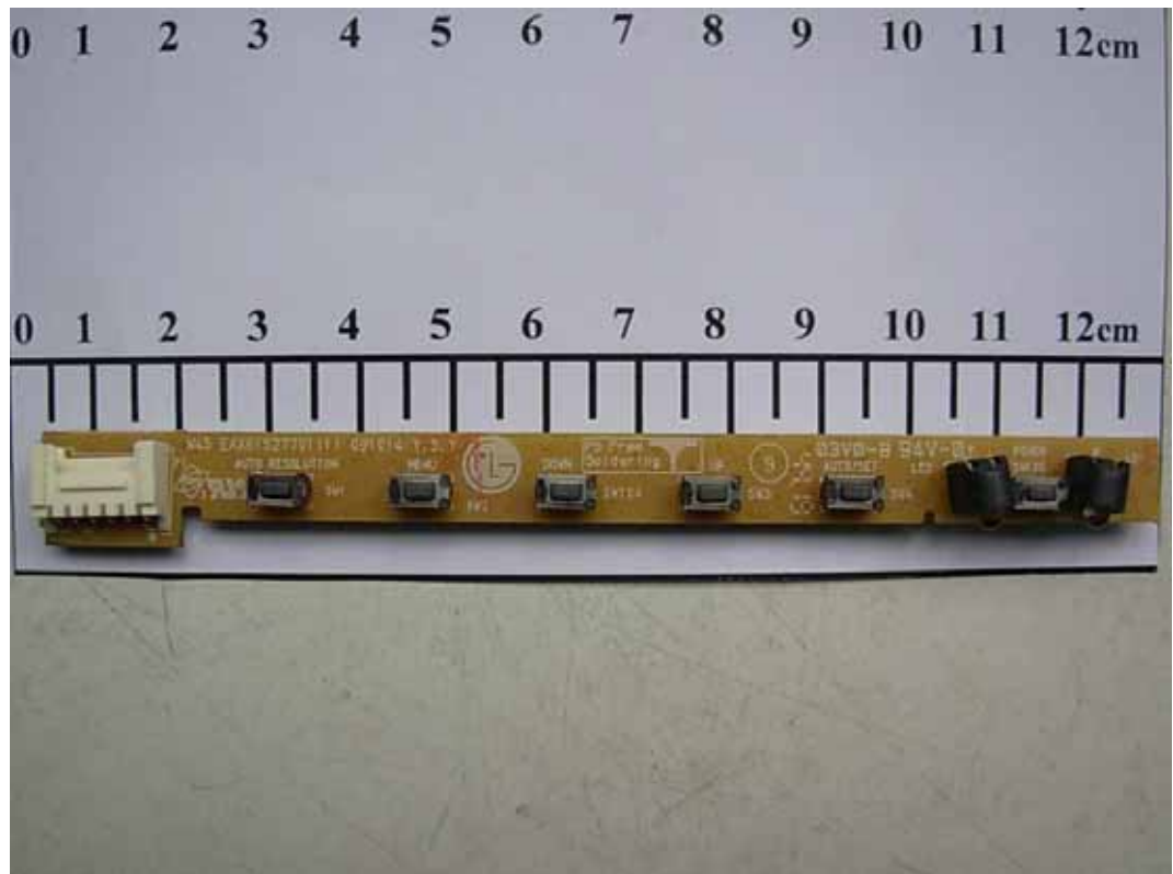
FIGURE 3 LCD MONITOR (M/N: W2340TV) KEY BOARD (COMPONENT SIDE)
