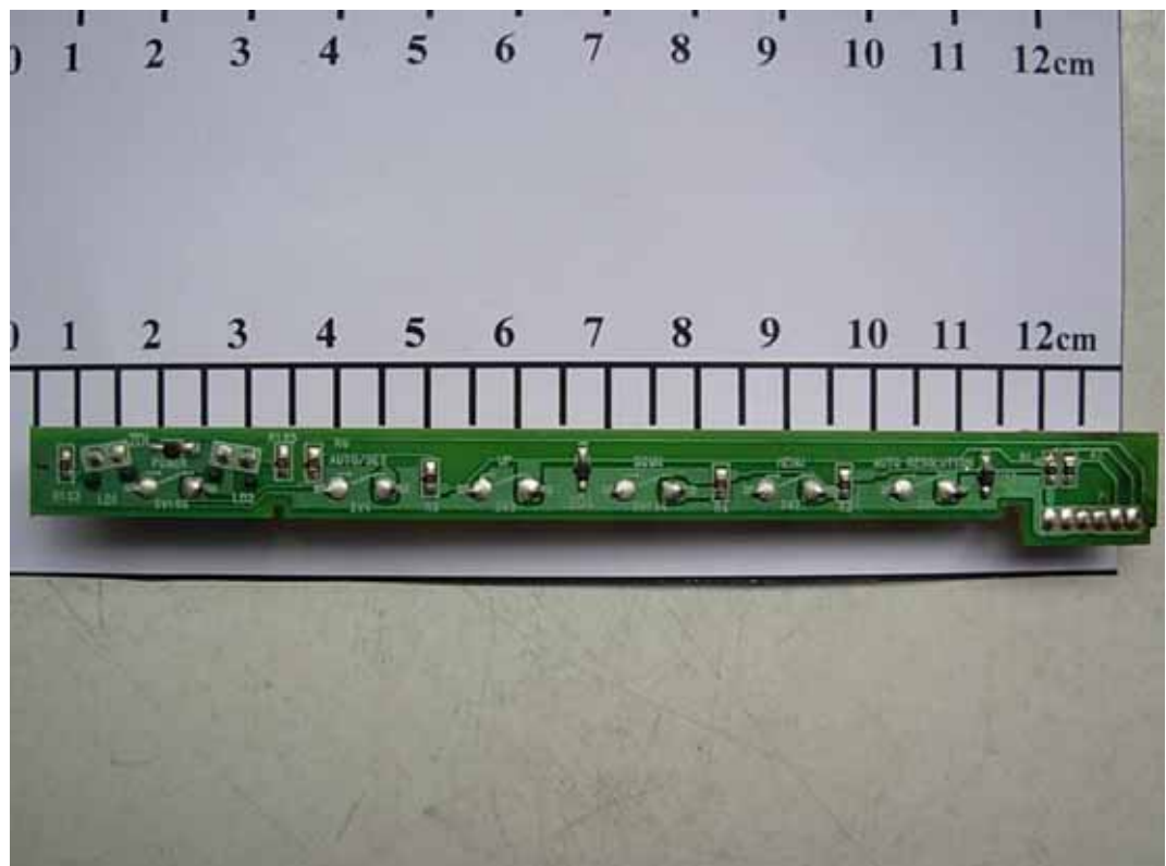
FIGURE 4 LCD MONITOR (M/N: W2340TV) KEY BOARD (SOLDERED SIDE)
