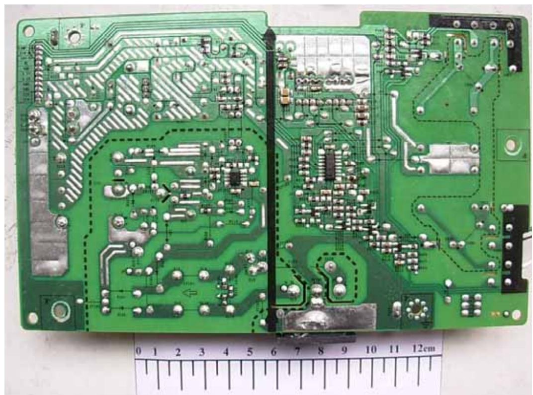
FIGURE 6 LCD MONITOR (M/N: W2340TV) POWER BOARD (SOLDERED SIDE)
