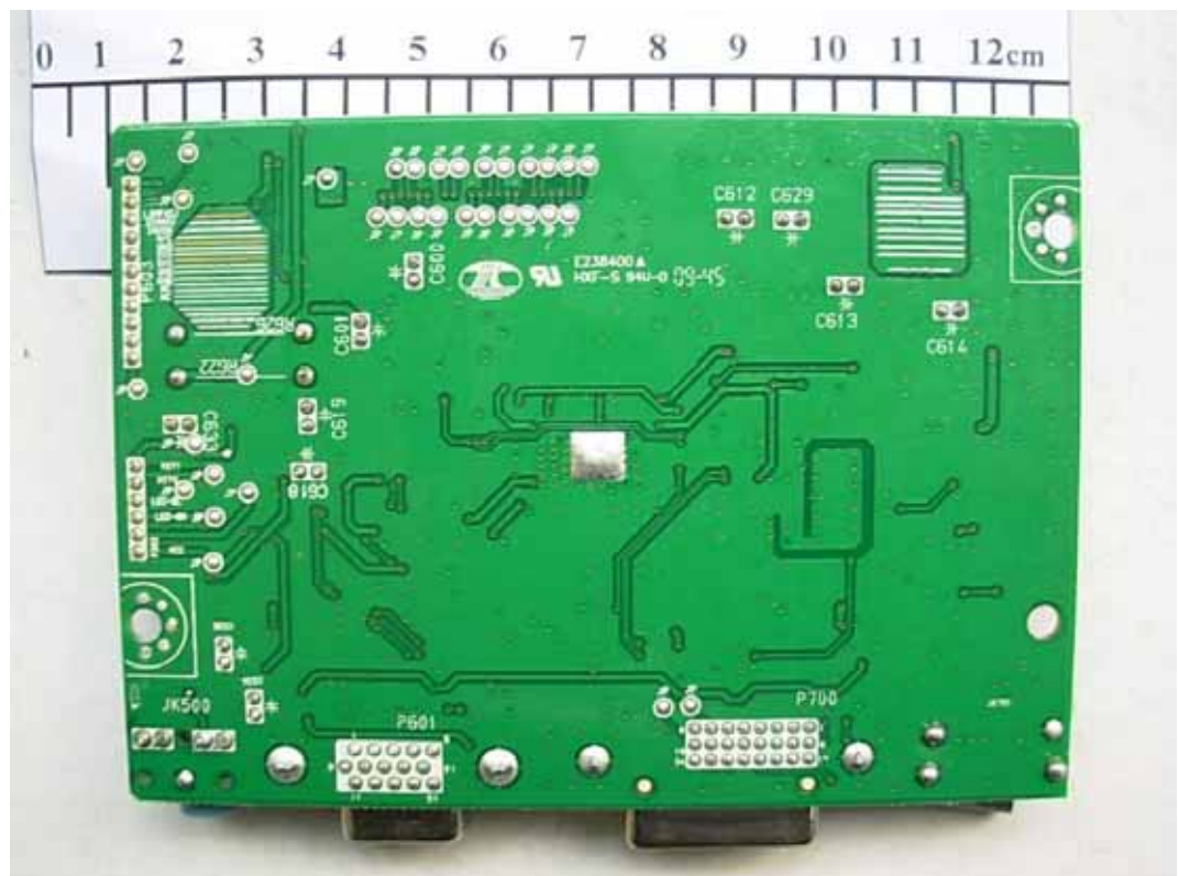
FIGURE 6 LCD MONITOR (M/N: W2340VV) MAIN BOARD (SOLDERED SIDE)
