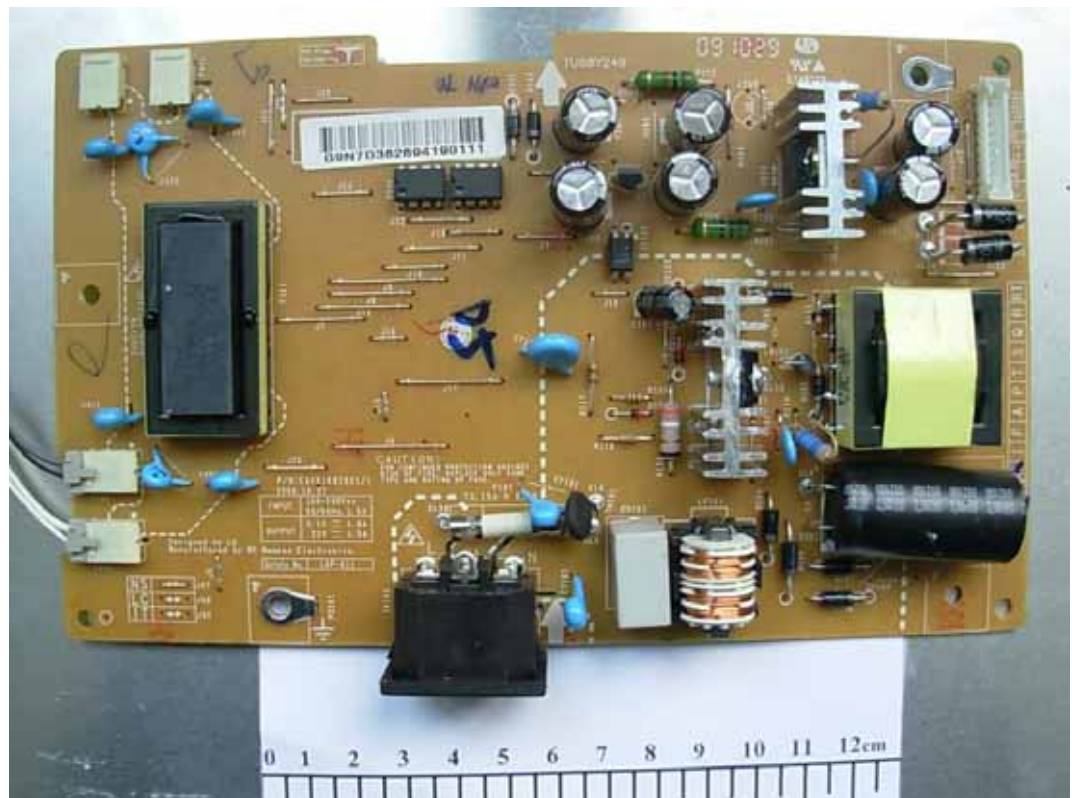
FIGURE 3 LCD MONITOR (M/N: W2340VV) POWER BOARD (COMPONENT SIDE)
