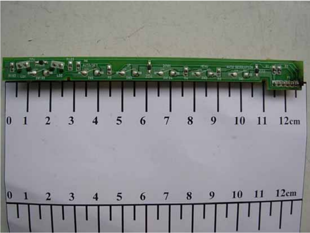
FIGURE 9 LCD MONITOR (M/N: W2340VV) KEY BOARD (SOLDERED SIDE)
