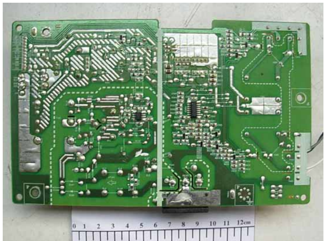
FIGURE 4 LCD MONITOR (M/N: W2340VV) POWER BOARD (SOLDERED SIDE)
