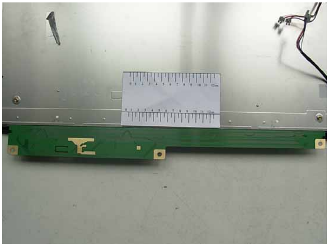
FIGURE 11 LCD MONITOR (M/N: W2353TQV) LCD PANEL MAIN BOARD (SOLDERED SIDE)
