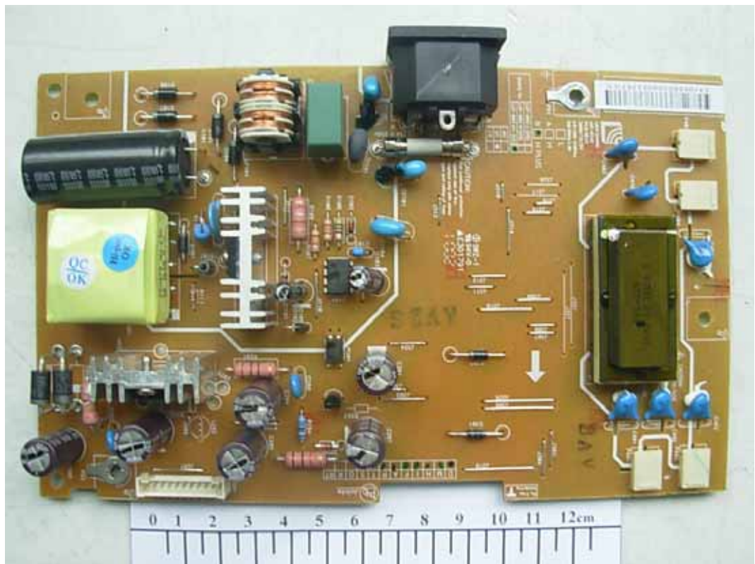
FIGURE 7 LCD MONITOR (M/N: W2353TQV) POWER BOARD (COMPONENT SIDE)
