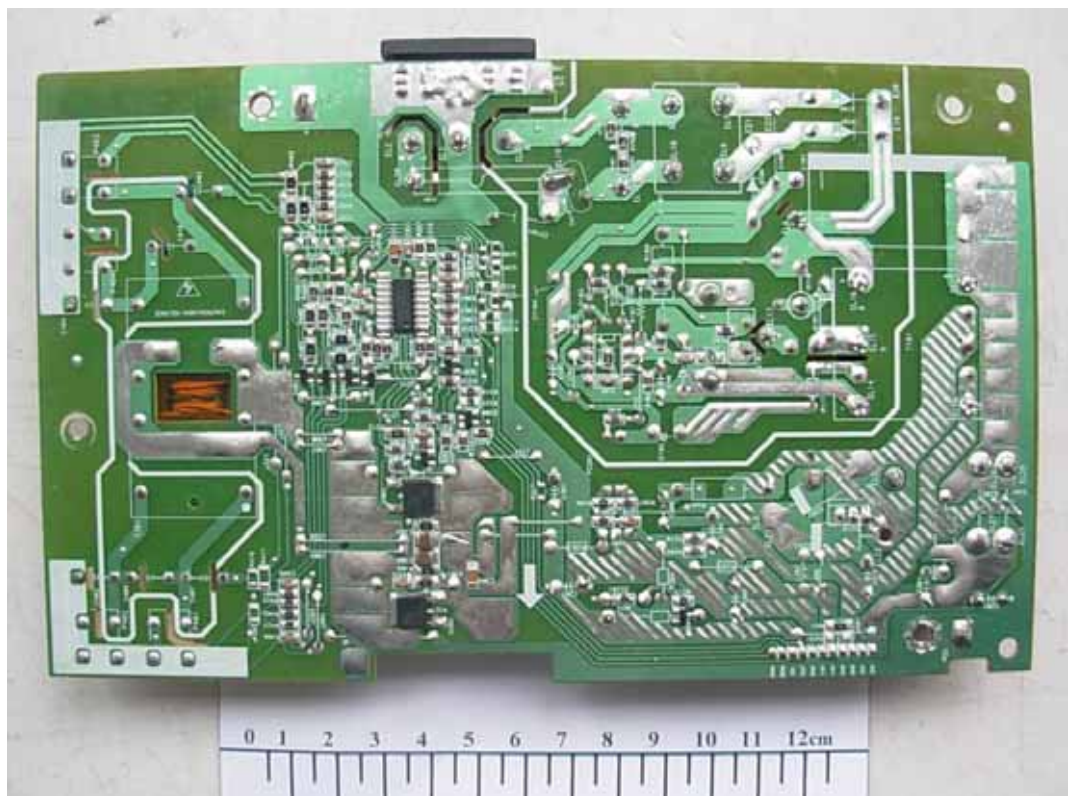
FIGURE 8 LCD MONITOR (M/N: W2353TQV) POWER BOARD (SOLDERED SIDE)
