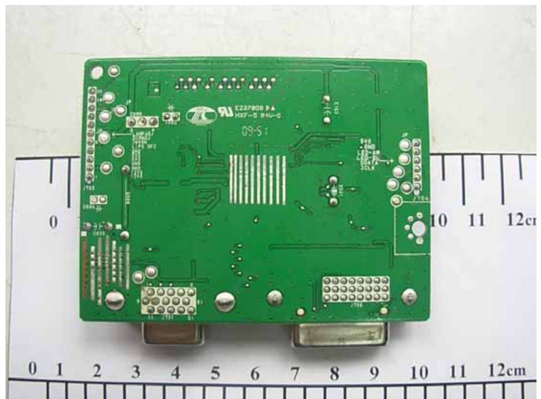
FIGURE 5 LCD MONITOR (M/N: W2353TQV) MAIN BOARD (SOLDERED SIDE)
