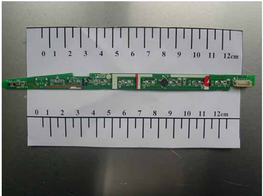
FIGURE 2 LCD MONITOR (M/N: W2353TQV) KEY BOARD (COMPONENT SIDE)
