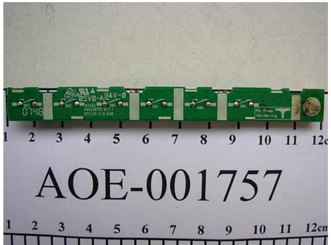
FIGURE 5 LCD MONITOR (M/N: W2452TQT) BUTTON BOARD (SOLDERED SIDE)
