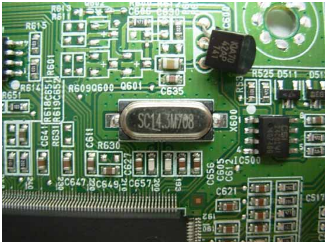
FIGURE 10 LCD MONITOR (M/N: W2452TQT) CRYSTAL ON MAIN BOARD
