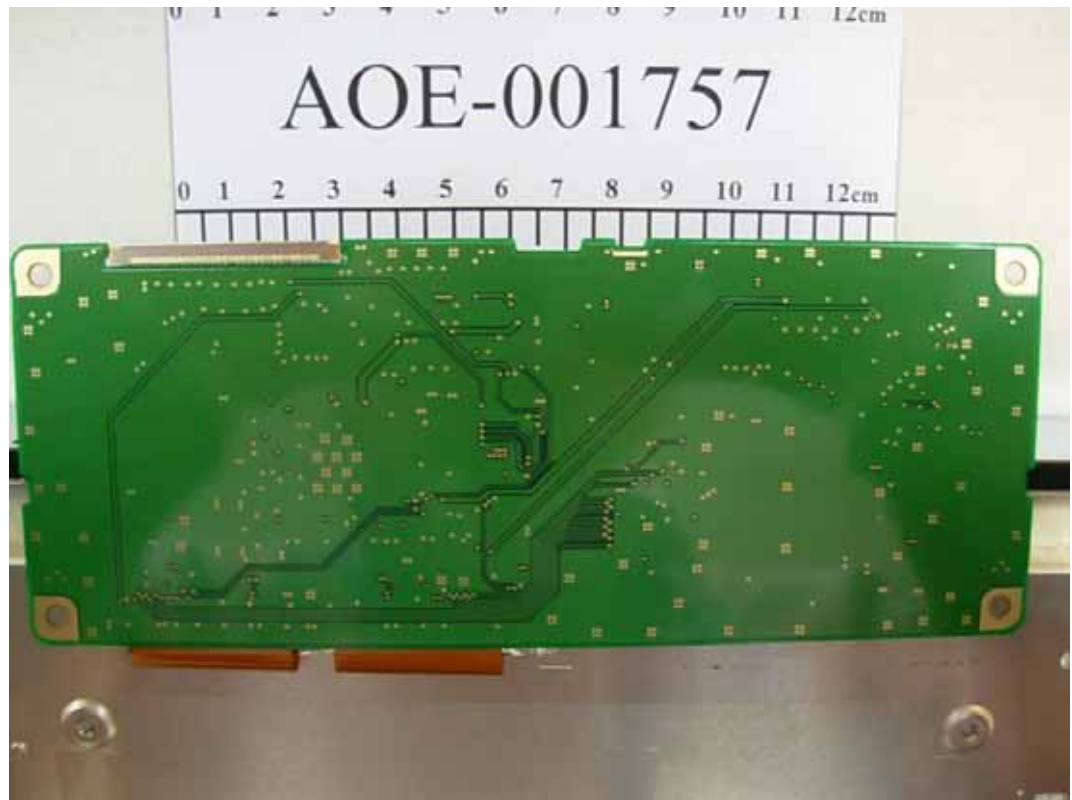
FIGURE 19 LCD MONITOR (M/N: W2452TQT) LCD PANEL MAIN BOARD (SOLDERED SIDE)
