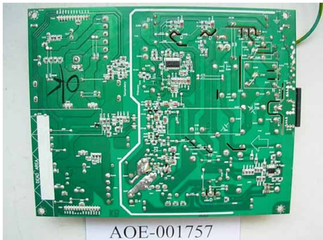
FIGURE 12 LCD MONITOR (M/N: W2452TQT) POWER BOARD (SOLDERED SIDE)
