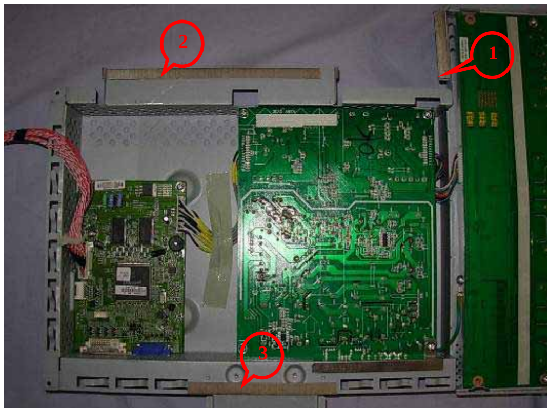
FIGURE 24 LCD MONITOR (M/N: W2452TQT) DEBUG 3
