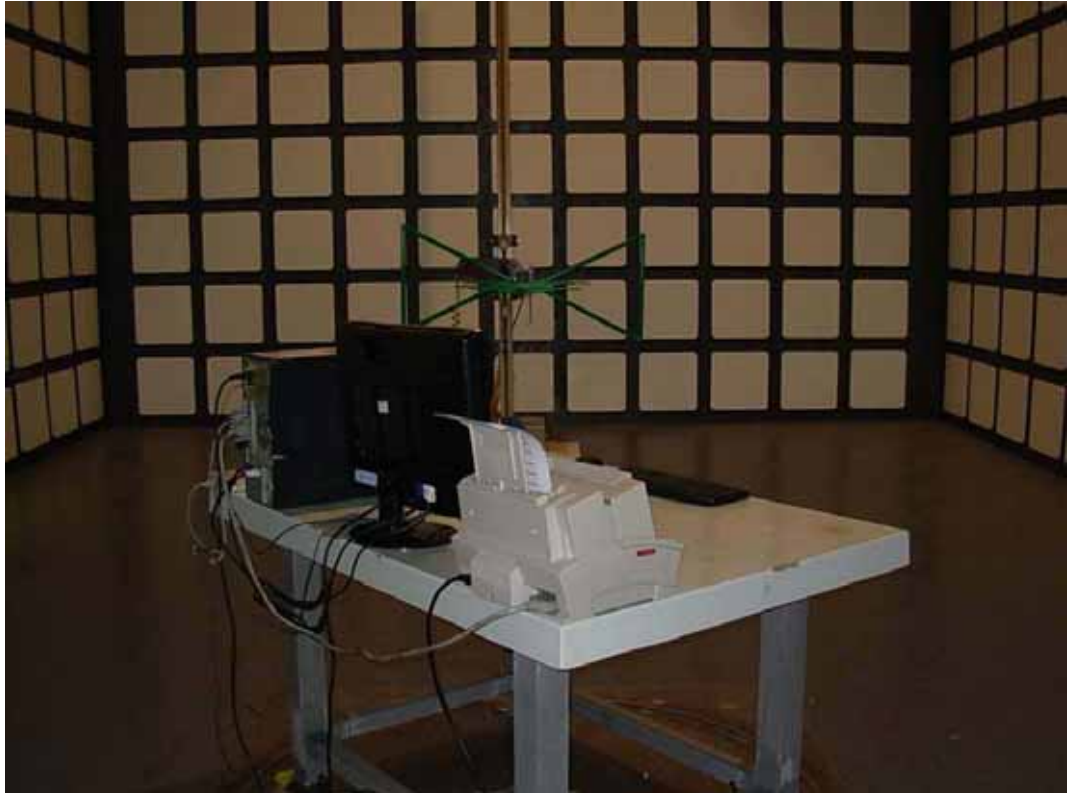
SETUP WITH MAXIMUM DETECTED EMISSION AT HORIZONTAL POLARIZATION (DVI 640*480@60Hz)
