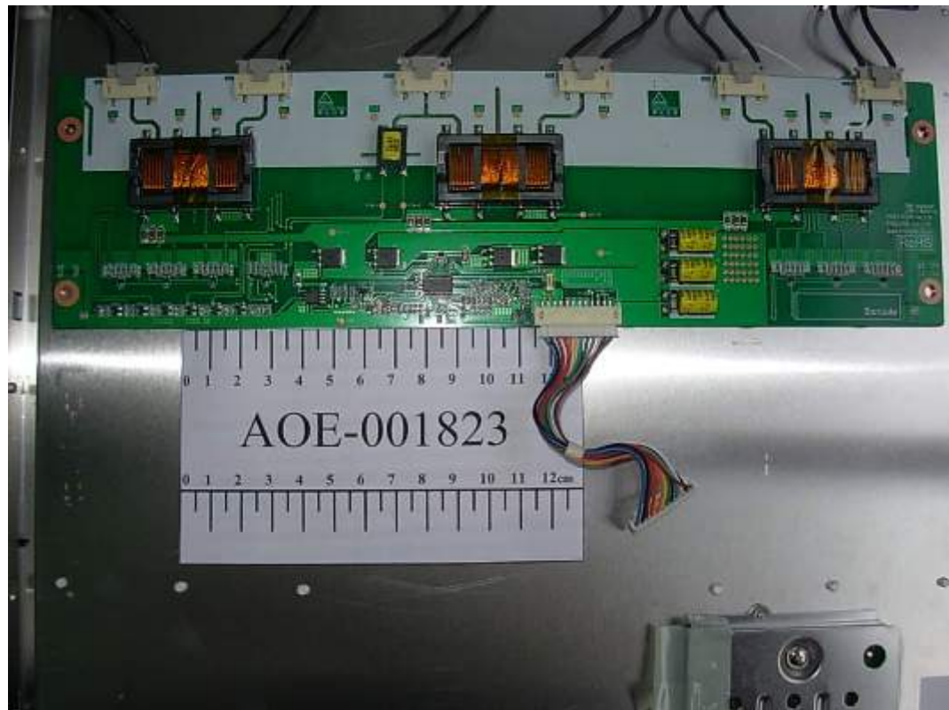
FIGURE 14 LCD MONITOR (M/N: W2452VQT) INVERTER BOARD (COMPONENT SIDE)
