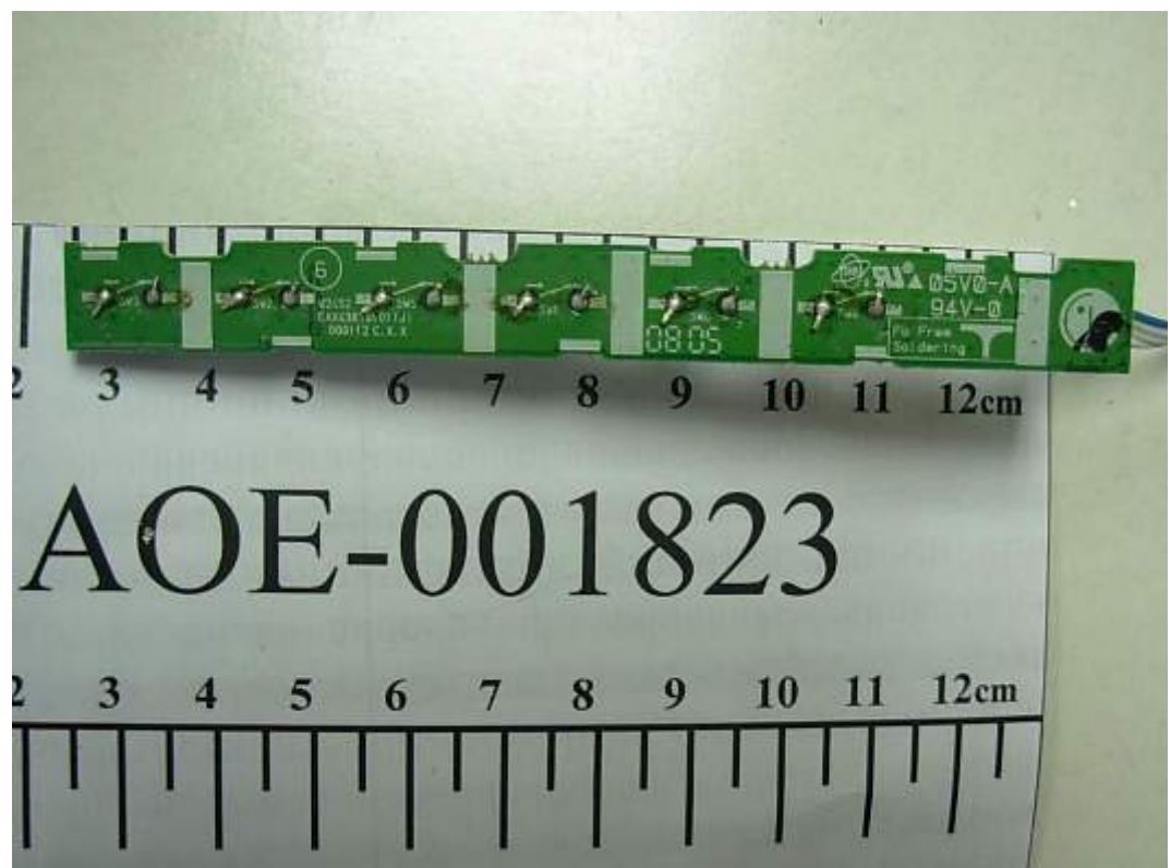
FIGURE 5 LCD MONITOR (M/N: W2452VQT) BUTTON BOARD (SOLDERED SIDE)
