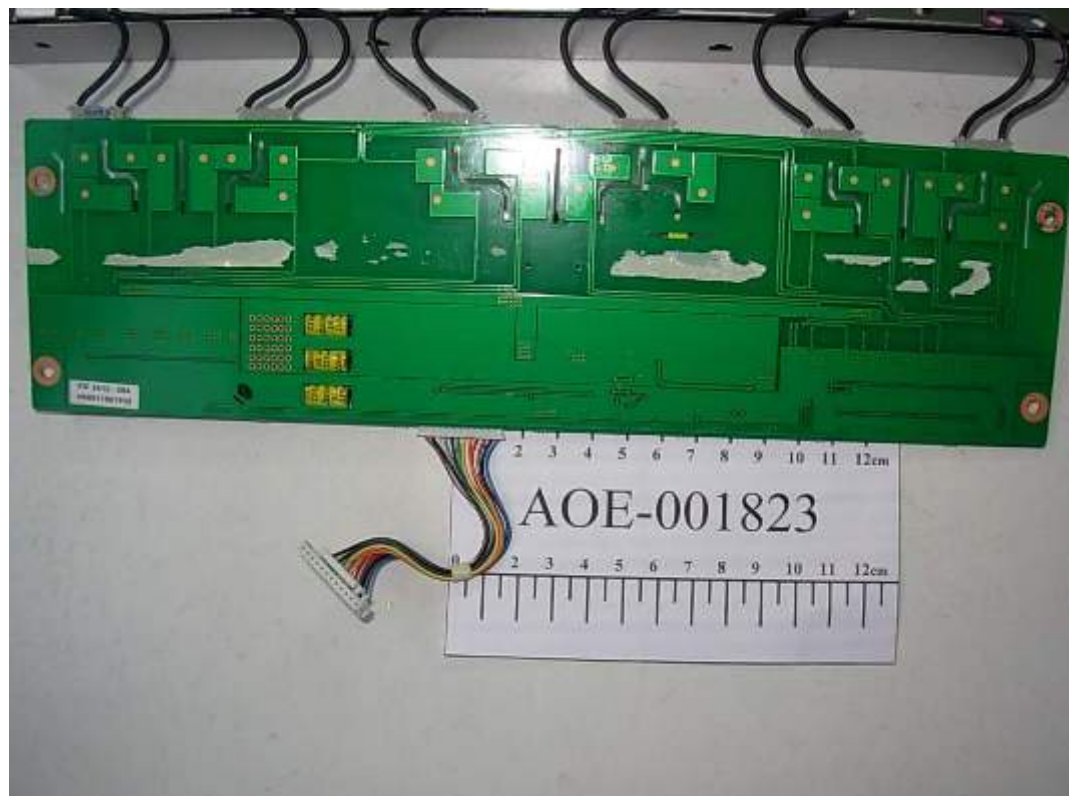
FIGURE 15 LCD MONITOR (M/N: W2452VQT) INVERTER BOARD (SOLDERED SIDE)
