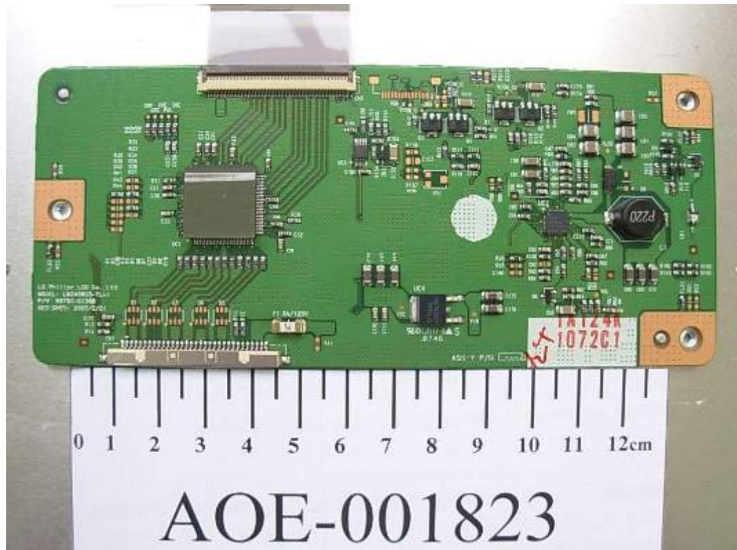
FIGURE 19 LCD MONITOR (M/N: W2452VQT) LCD PANEL MAIN BOARD (COMPONENT SIDE)
