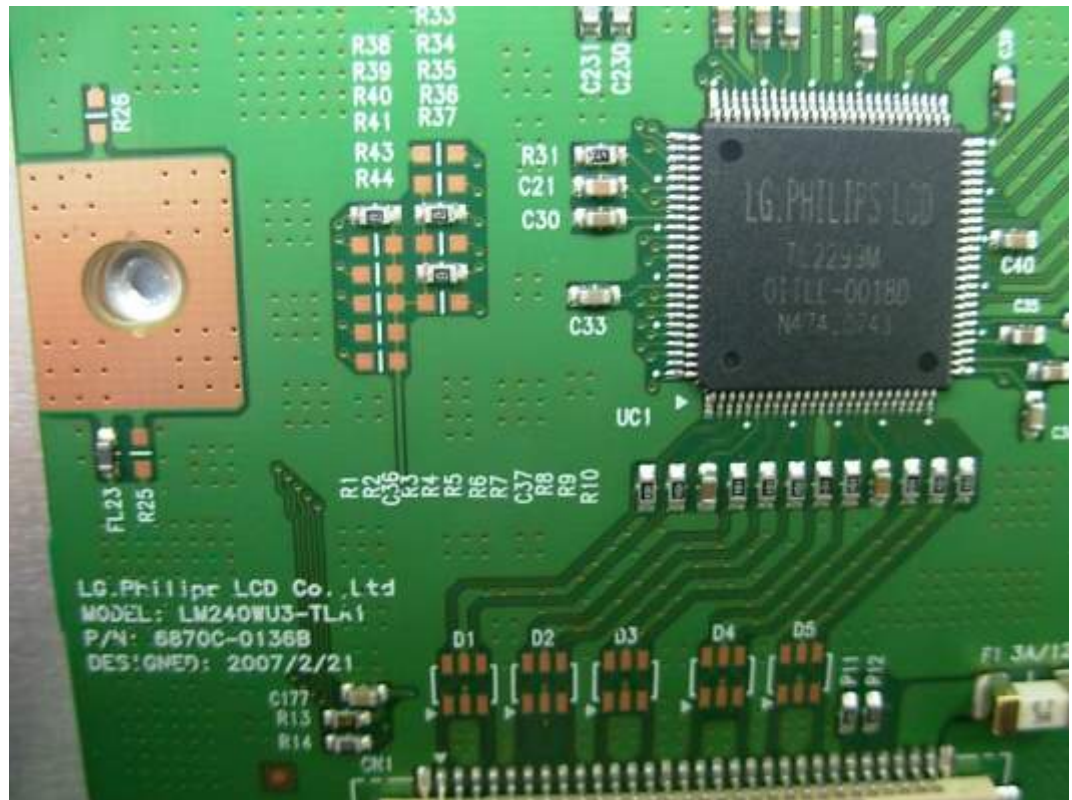
FIGURE 21 LCD MONITOR (M/N: W2452VQT) CHIP & LABEL ON LCD PANEL MAIN BOARD
