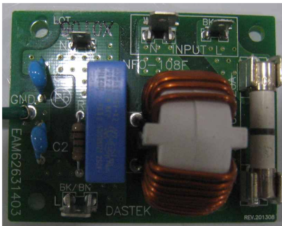
<Noise filter>
