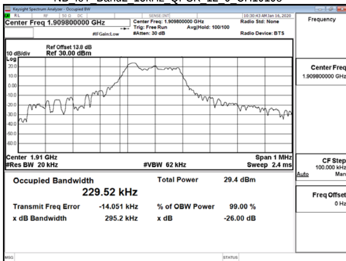
NB IoT Band2 15kHz QPSK 12 0 CH19198
