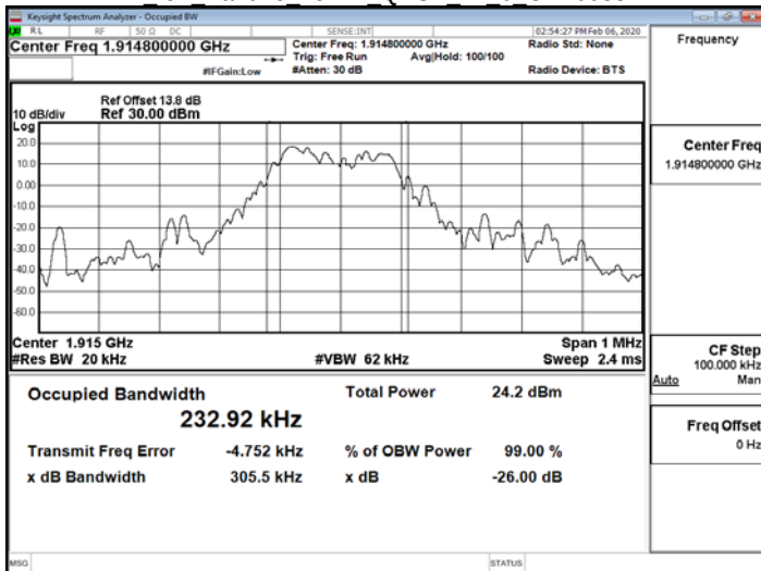
NB IoT Band25 15kHz QPSK 12 0 CH26688
