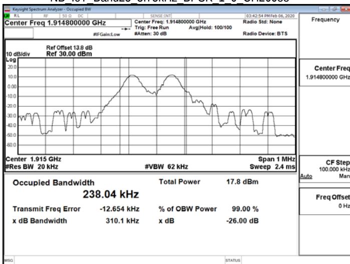
NB IoT Band25 3.75kHz BPSK 1 0 CH26688
