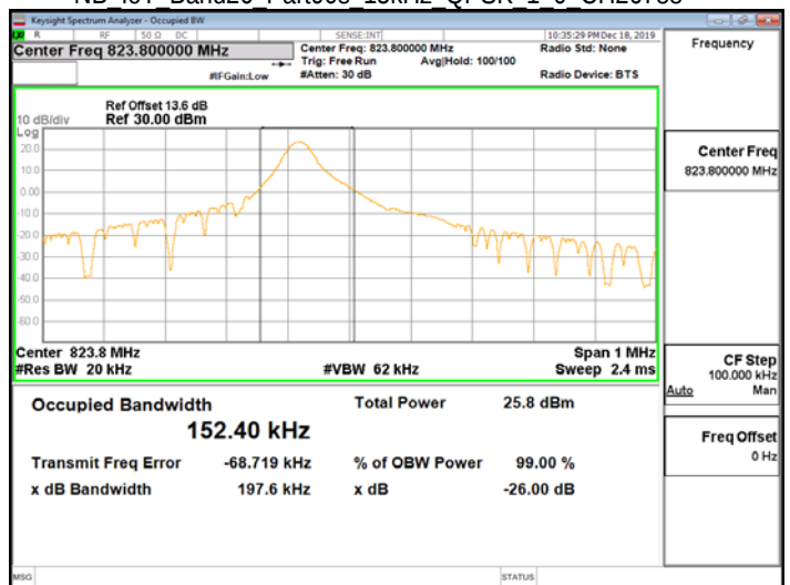
NB IoT Band26 Part90s 15kHz QPSK 1 0 CH26788
