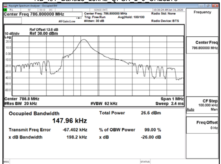
NB IoT Band13 15kHz QPSK 1 0 CH23278
