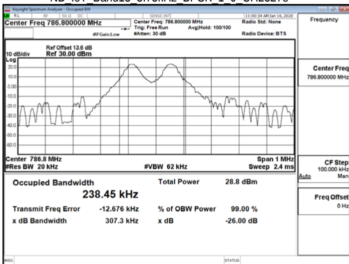
NB IoT Band13 3.75kHz BPSK 1 0 CH23278
