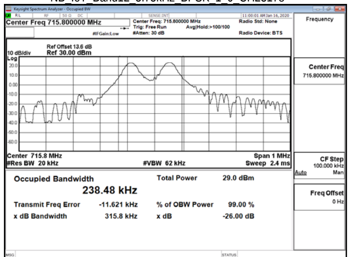
NB IoT Band12 3.75kHz BPSK 1 0 CH23178
