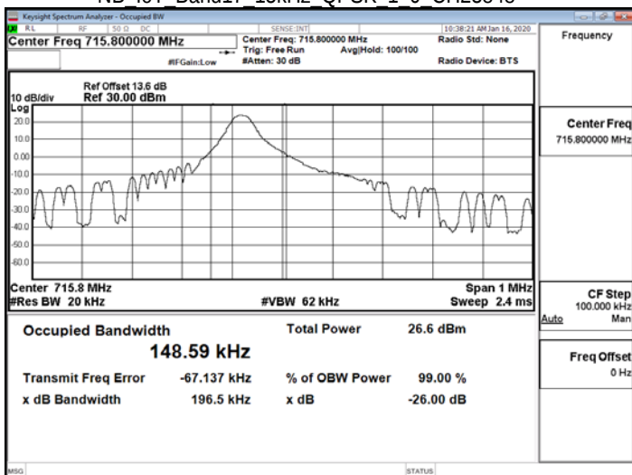
NB IoT Band17 15kHz QPSK 1 0 CH23848
