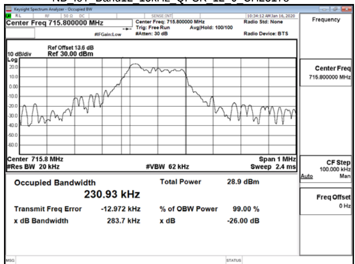
NB IoT Band12 15kHz QPSK 12 0 CH23178
