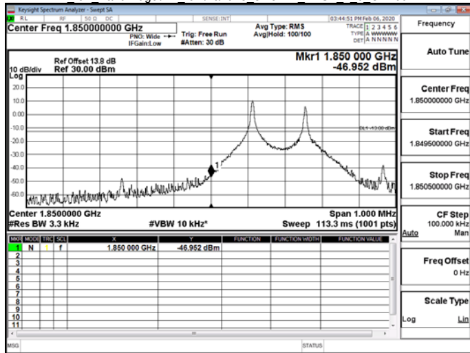
NB IoT_Band Edge\NB IoT\Band25 3.75kHz BPSK 1 47 CH26688
