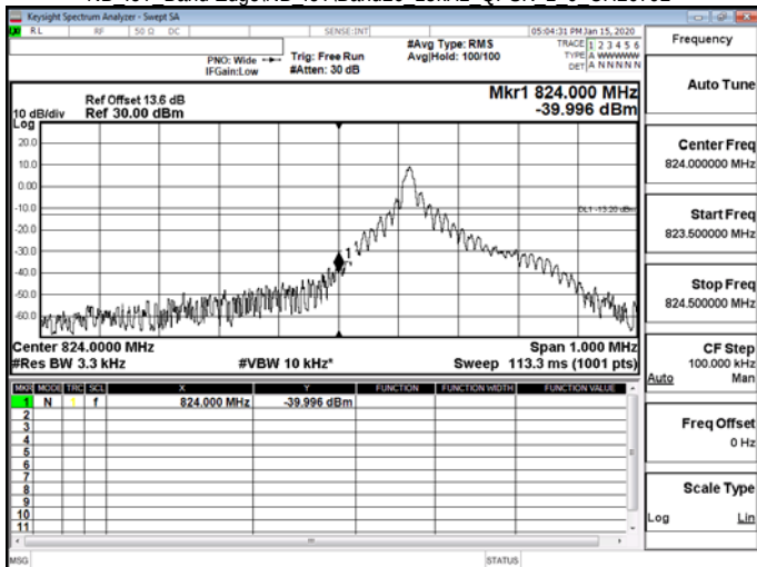
NB IoT Band Edge/NB IoT Band26 15kHz QPSK 1 0 CH26792
