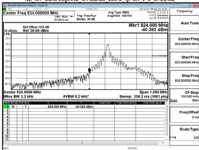
NB IoT_Band Edge\NB IoT\Band5 15kHz QPSK 1 0 CH20402
