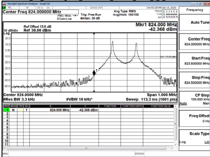
NB IoT Band Edge/NB IoT Band26 3.75kHz BPSK 1 47 CH27038
