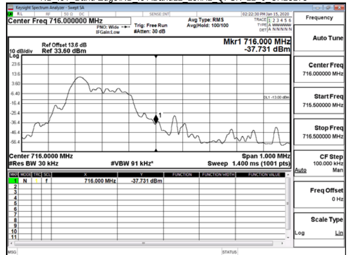
NB IoT_Band Edge\NB IoT\Band12 15kHz QPSK 12 0 CH23178
