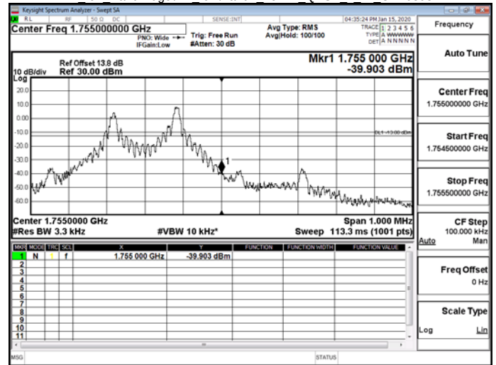
NB IoT_Band Edge\NB IoT\Band4 15kHz QPSK 12 0 CH19952
