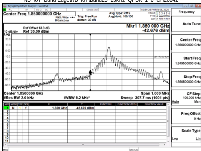
NB IoT_Band Edge\NB IoT\Band25 15kHz QPSK 1 0 CH26042
