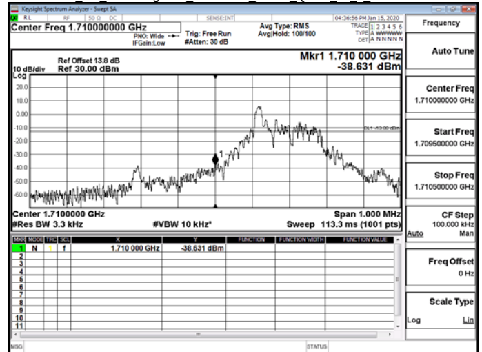
NB IoT_Band Edge\NB IoT\Band4 15kHz QPSK 12 0 CH20398
