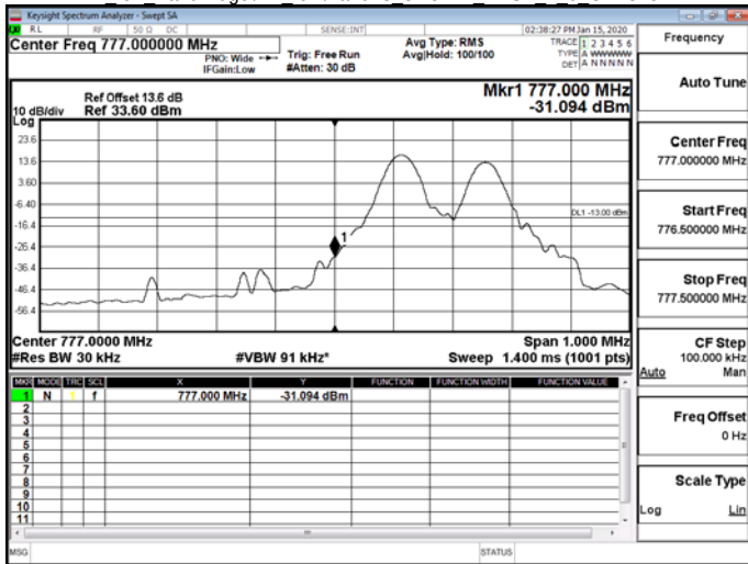
NB IoT_Band Edge\NB IoT\Band13 3.75kHz BPSK 1 47 CH23278
