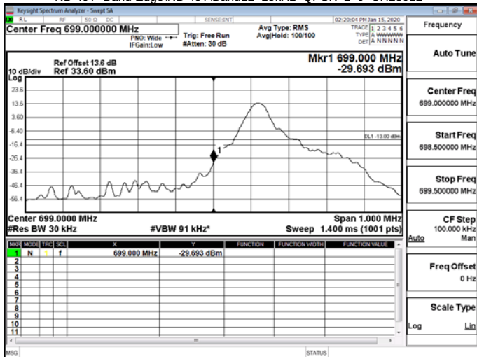
NB IoT_Band Edge\NB IoT\Band12 15kHz QPSK 1 0 CH23012
