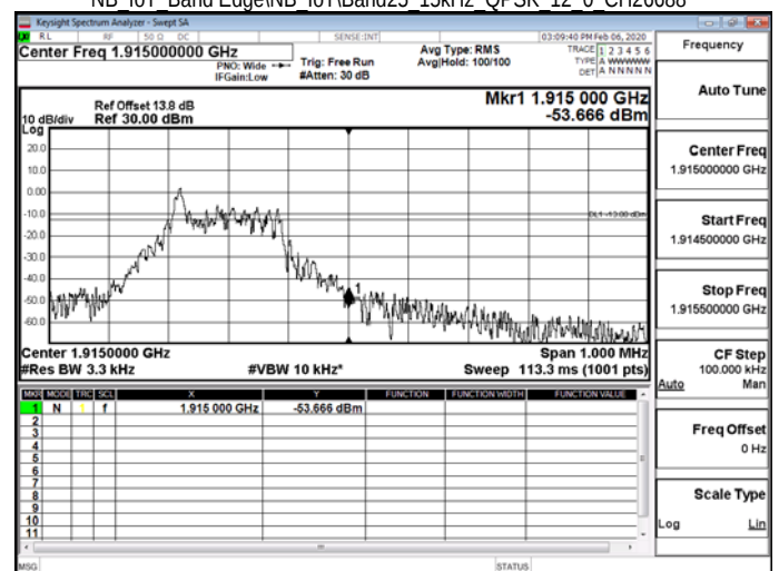
NB IoT_Band Edge\NB IoT\Band25 15kHz QPSK 12 0 CH26688
