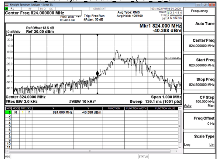
NB IoT_Band Edge\NB IoT\Band5 15kHz QPSK 12 0 CH20648
