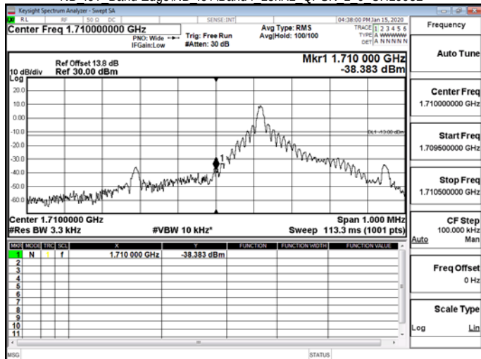
NB IoT_Band Edge\NB IoT\Band4 15kHz QPSK 1 0 CH19952
