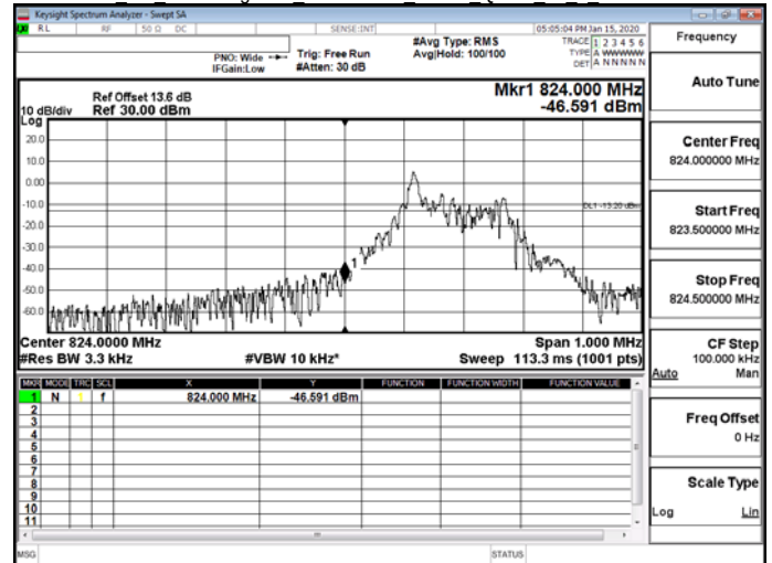
NB IoT Band Edge/NB IoT Band26 15kHz QPSK 12 0 CH27038
