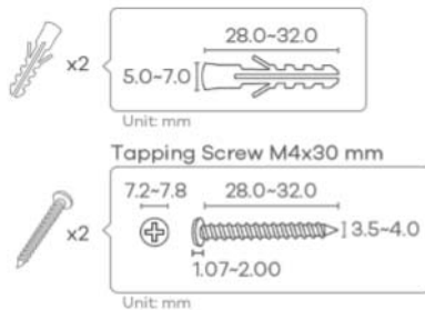
Figure 4 Screw Specifications
