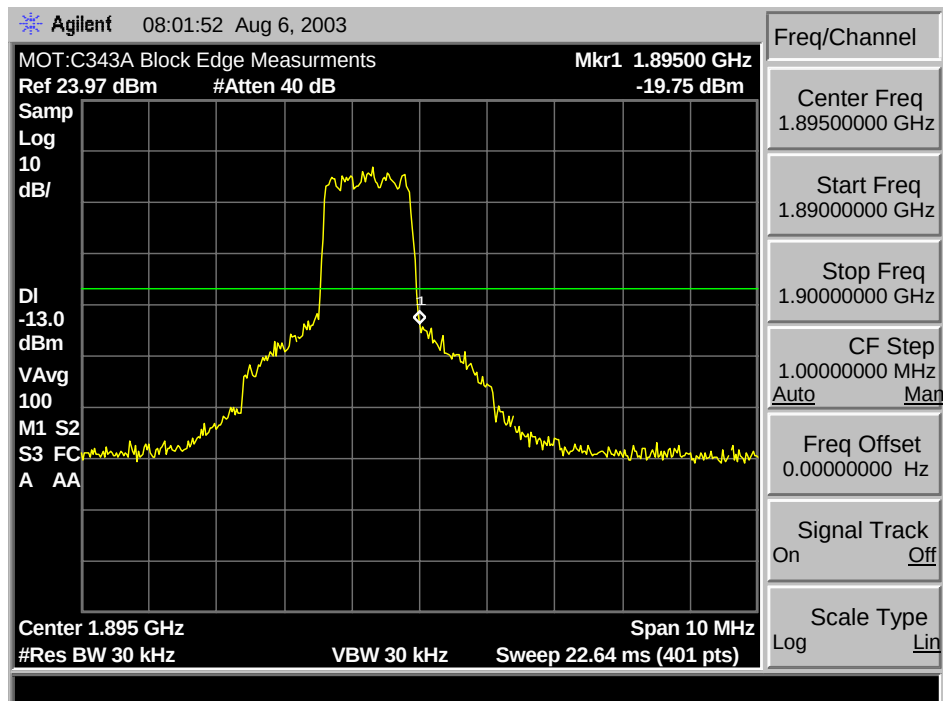
1900 CDMA F Max. Block Edge
