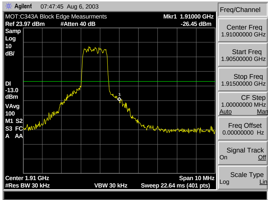
1900 CDMA C Max Block Edge
