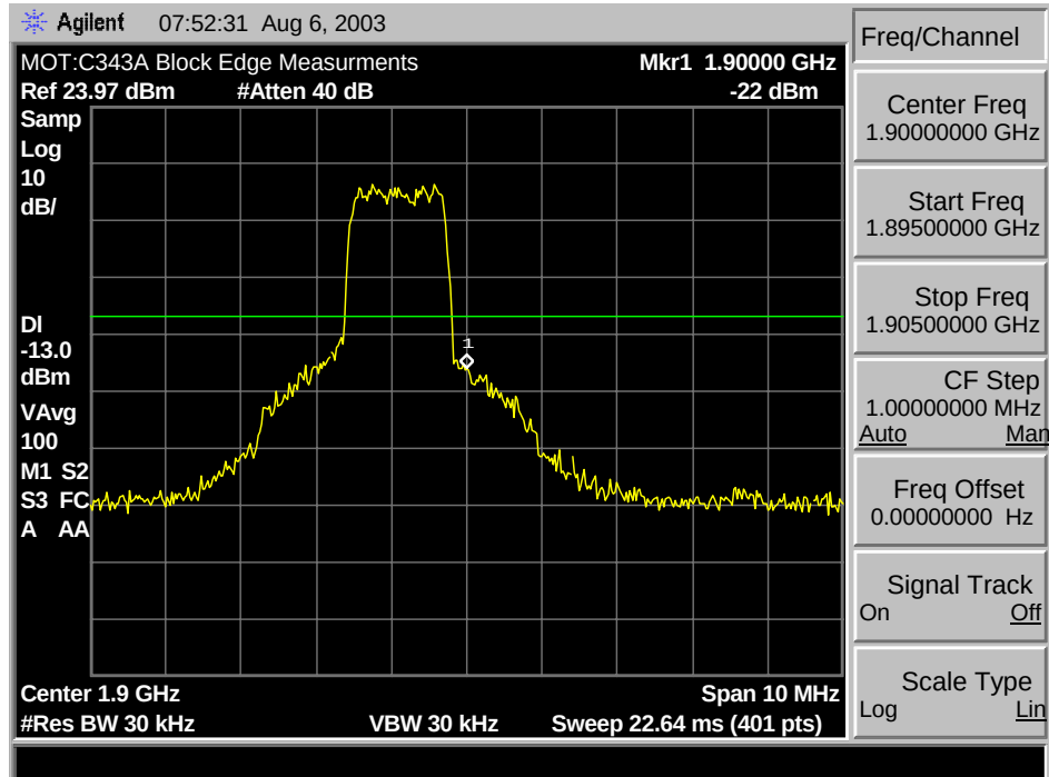
1900 CDMA C3 Max. Block Edge
