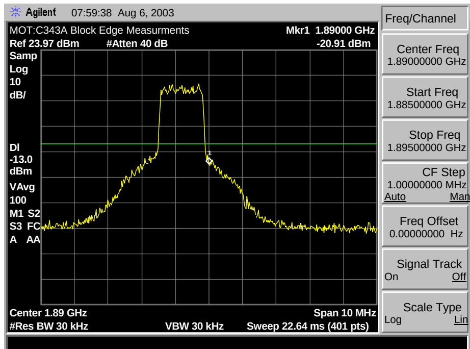
1900 CDMA E Max. Block Edge
