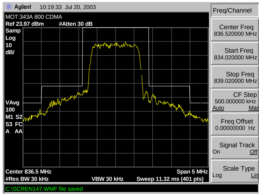
800 CDMA Bandwidth
