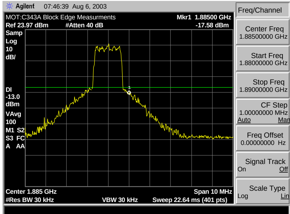
1900 CDMA B Max. Block Edge
