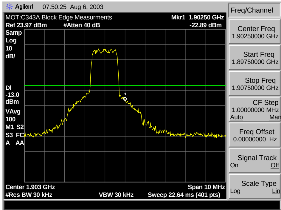
1900 CDMA C2 Max Block Edge
