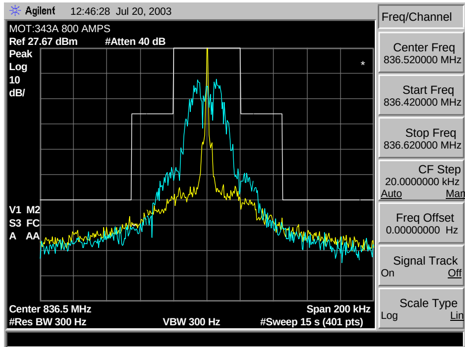
800 AMPS Voice
