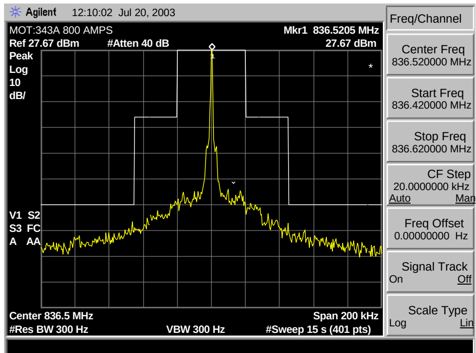
800 AMPS Unmodulated
