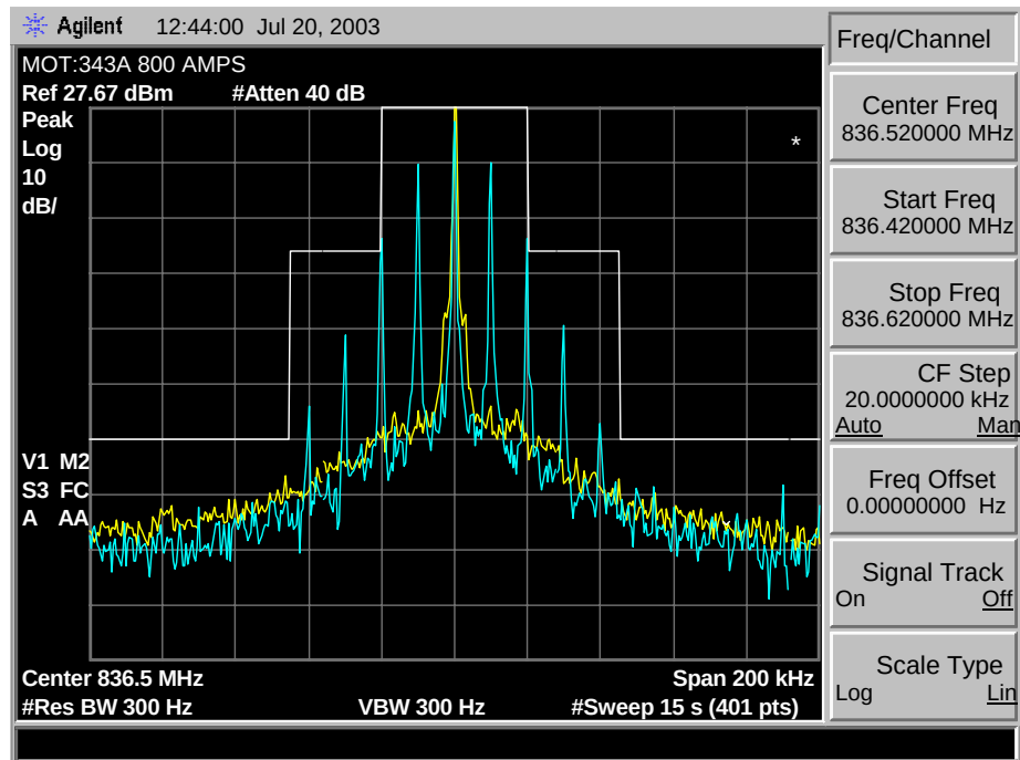
800 AMPS Signal
