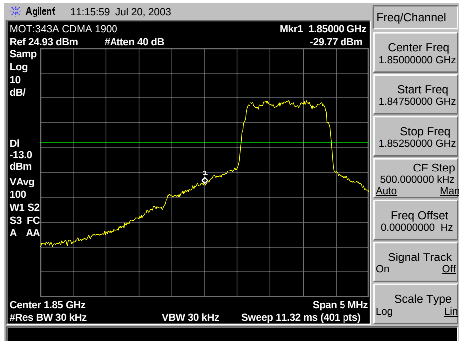
1900 CDMA Lower Band Edge
