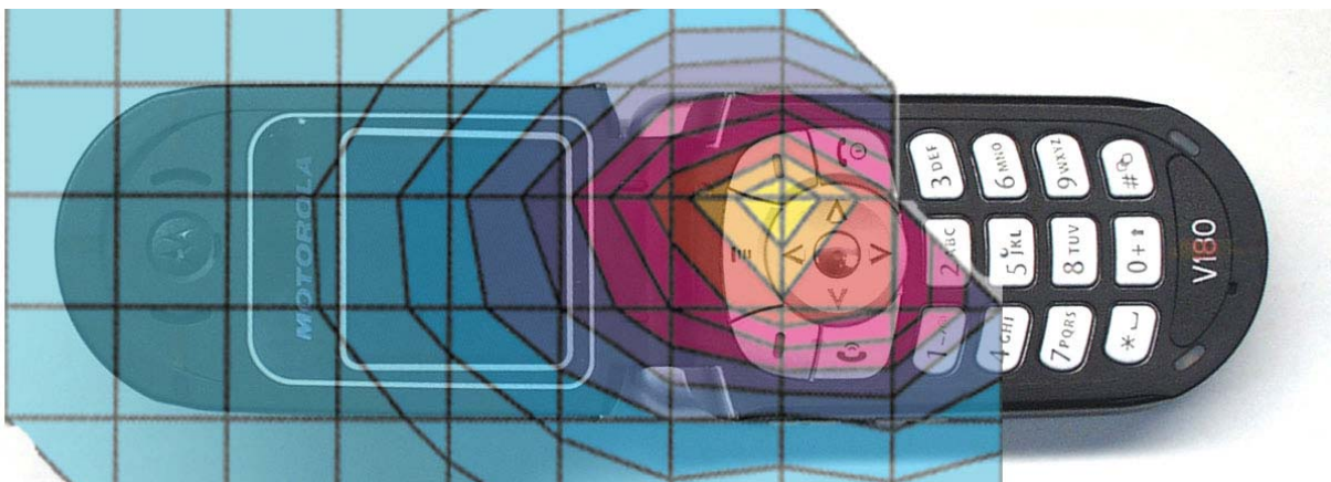
Figure 1. 800MHz Head Adjacent Contour Overlaid on Phone (Cheek Touch)
