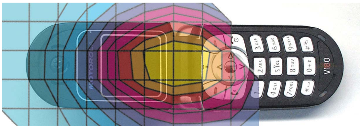
Figure 3. Typical 800MHz Head Adjacent Contour Overlaid on Phone (15 ° Tilt)
