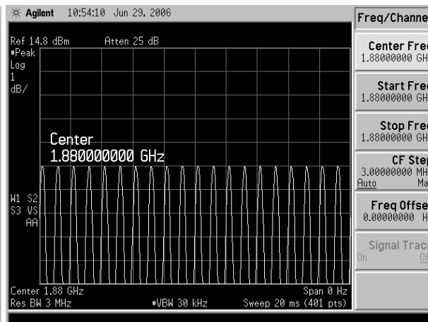
80% AM 1880 MHz
