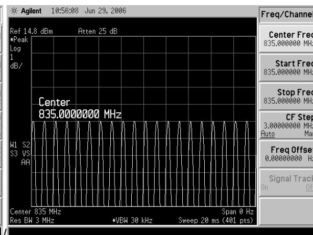
80% AM 835 MHz
