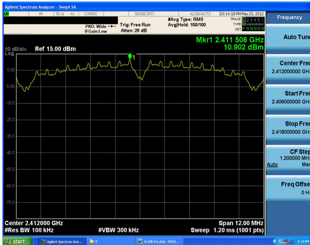
Plot 6-10. Power Spectral Density Plot (802.11b – Ch. 1)
