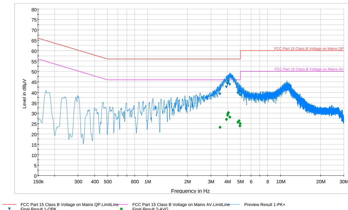
Plot 6-31. Line Conducted Plot with 802.11b (L1)
