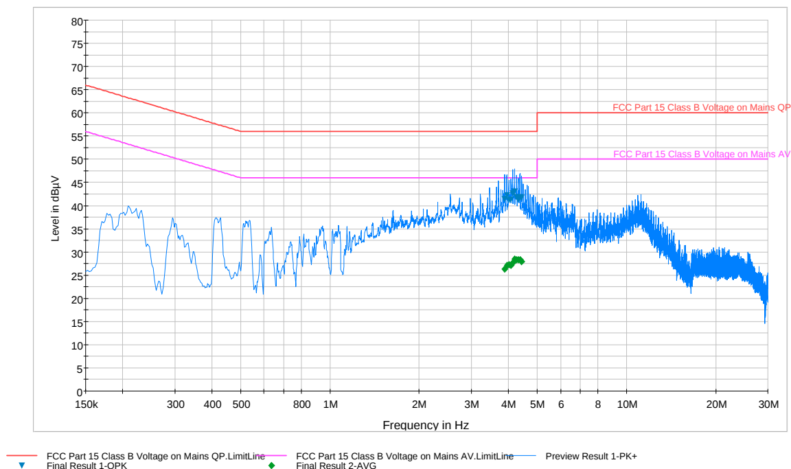
Plot 6-32. Line-Conducted Test Plot with 802.11b (N)
