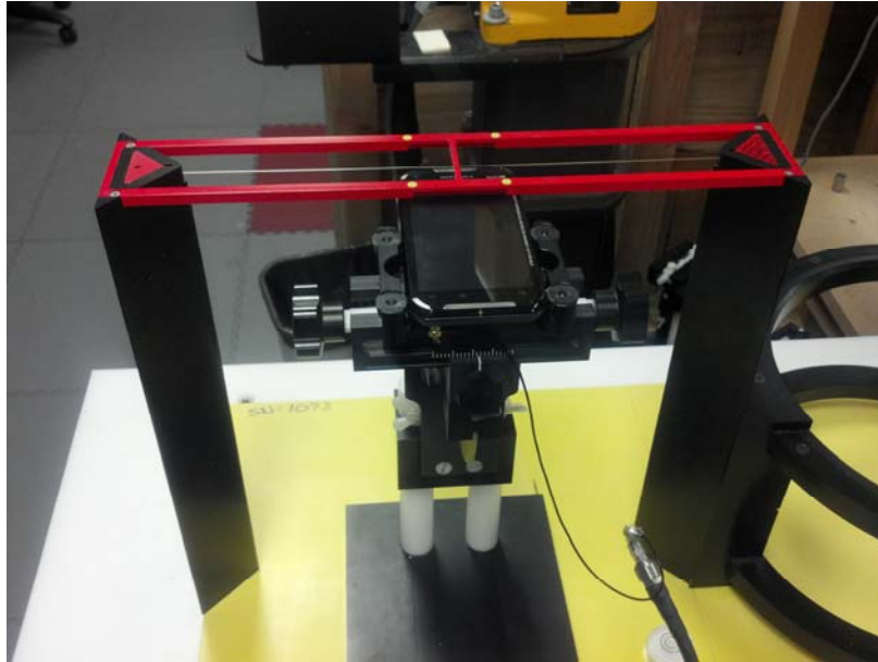
Figure 7. Positioning and Measurement for T-coil
