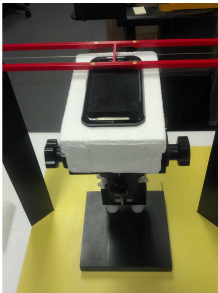
Figure 4. Positioning and Measurement for RF Emissions
