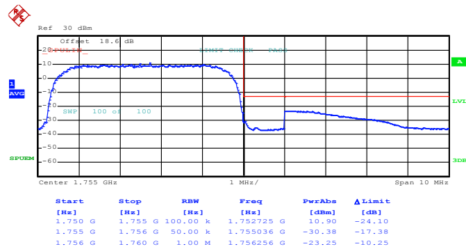
Higher Band Edge Plot on Channel 1513 (1752.6 MHz)
