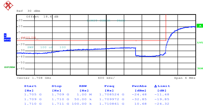
Lower Band Edge Plot on Channel 1312 (1712.4 MHz)
