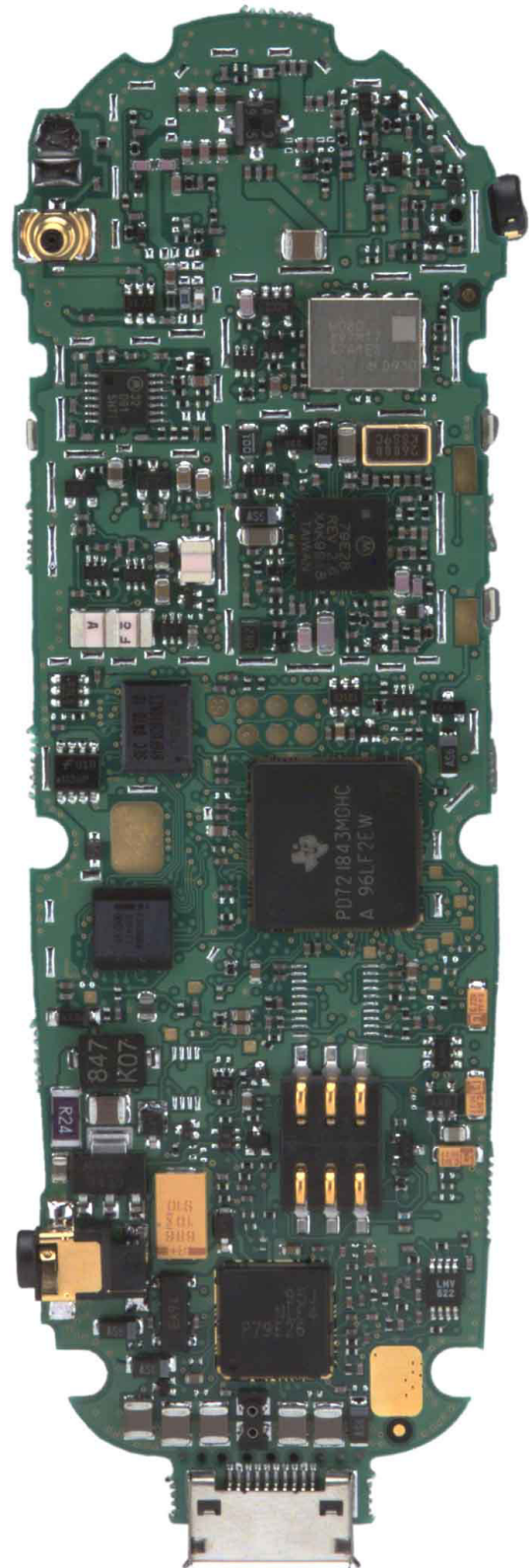
Rear View (Shields Removed)
