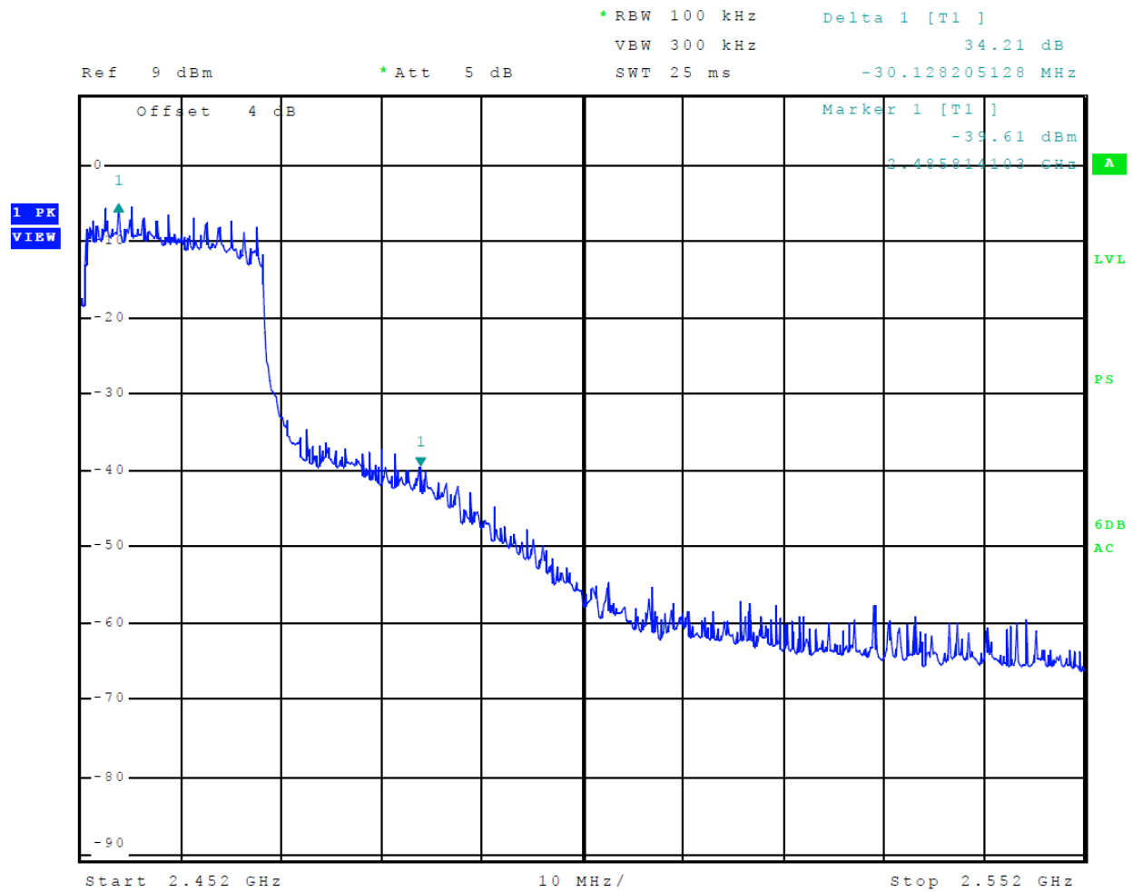
Figure 16 Plot of Transmitter Emissions High Band Edge Mode 8 802.11n
