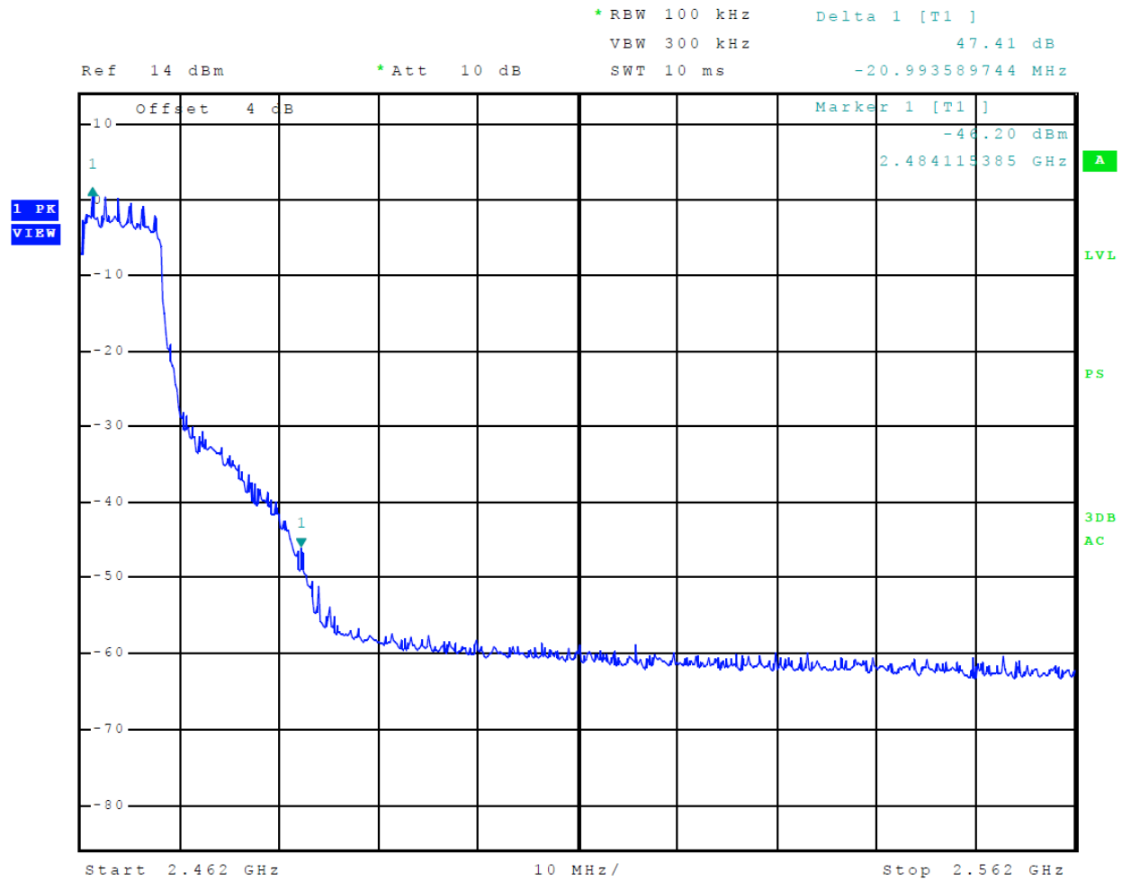
Figure 14 Plot of Transmitter Emissions High Band Edge Mode 7 802.11g
