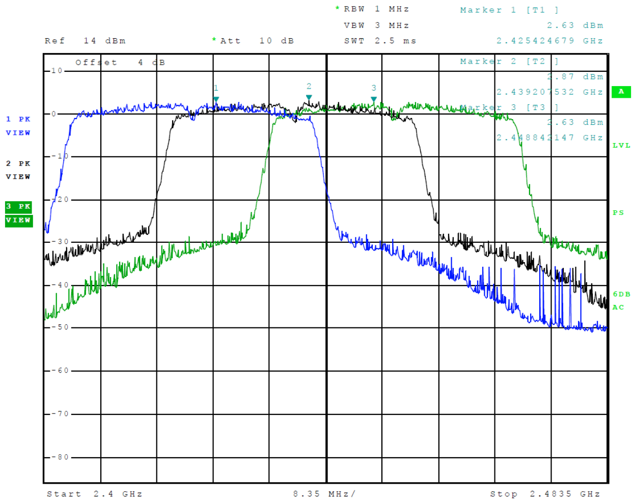
Figure 8 Plot of Transmitter Operation in 2412-2462 MHz Mode 8 802.11n40
