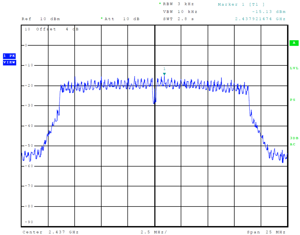
Figure 27 Plot of Transmitter Power Spectral Density Mode 8 802.11n
