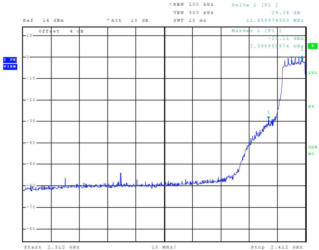
Figure 10 Plot of Transmitter Emissions Low Band Edge Mode 7 802.11g
