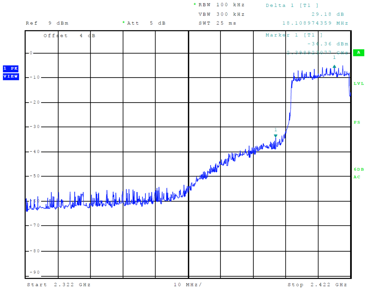
Figure 12 Plot of Transmitter Emissions Low Band Edge Mode 8 802.11n40
