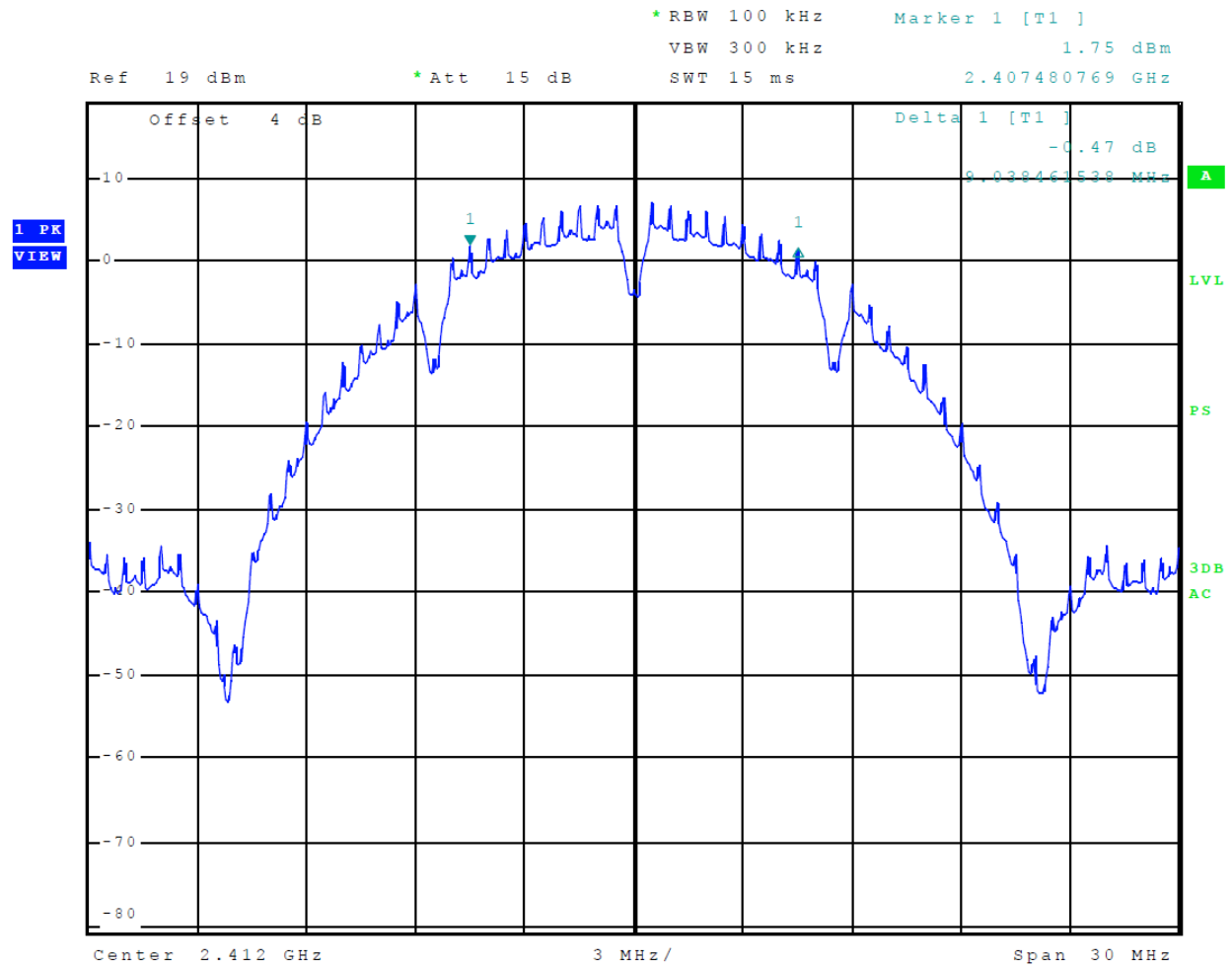
Figure 17 Plot of 6-dB Occupied Bandwidth Mode 6 802.11b
