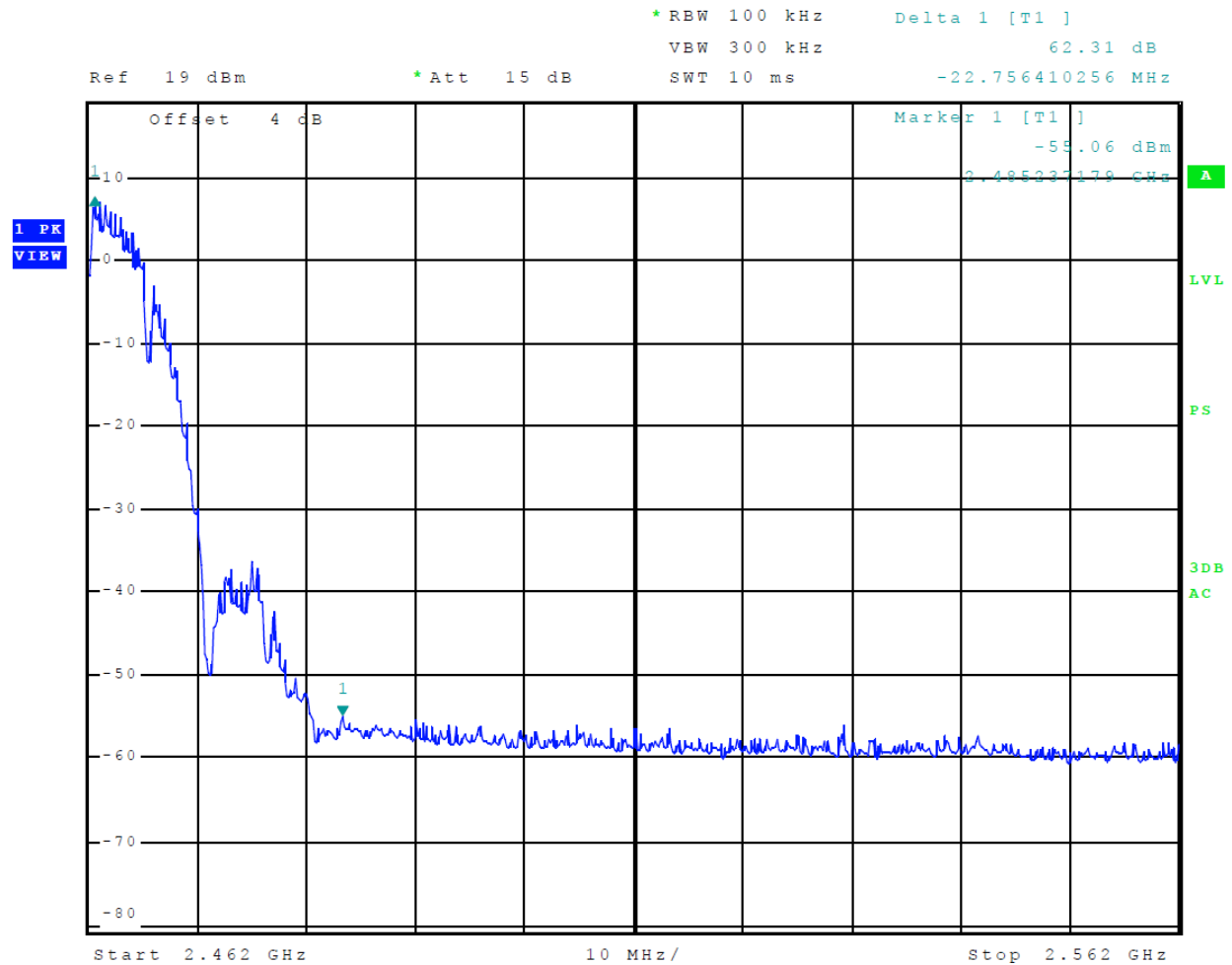
Figure 13 Plot of Transmitter Emissions High Band Edge Mode 6 802.11b
