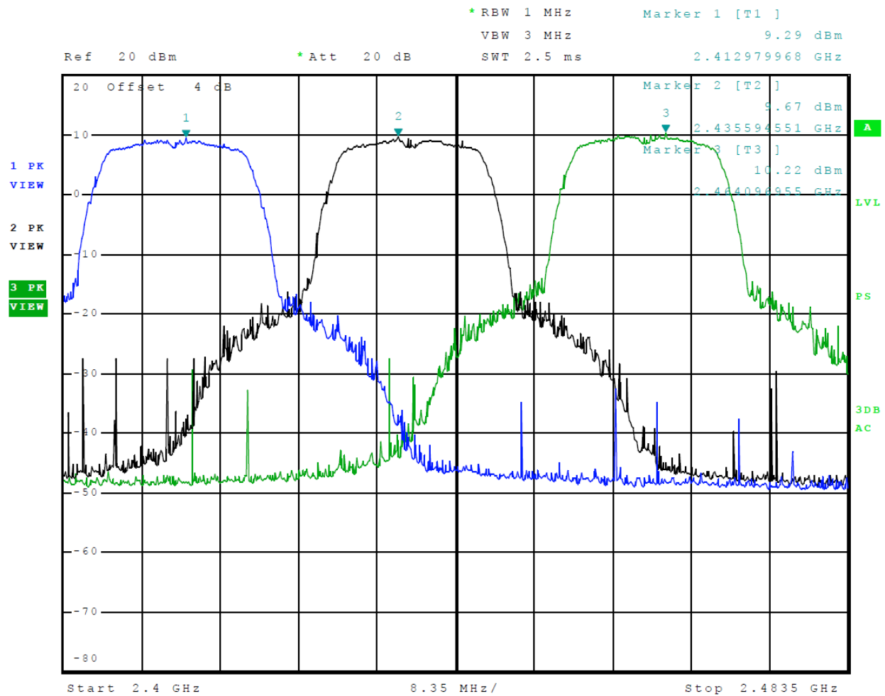
Figure 6 Plot of Transmitter Operation in 2412-2462 MHz Mode 7 802.11g
