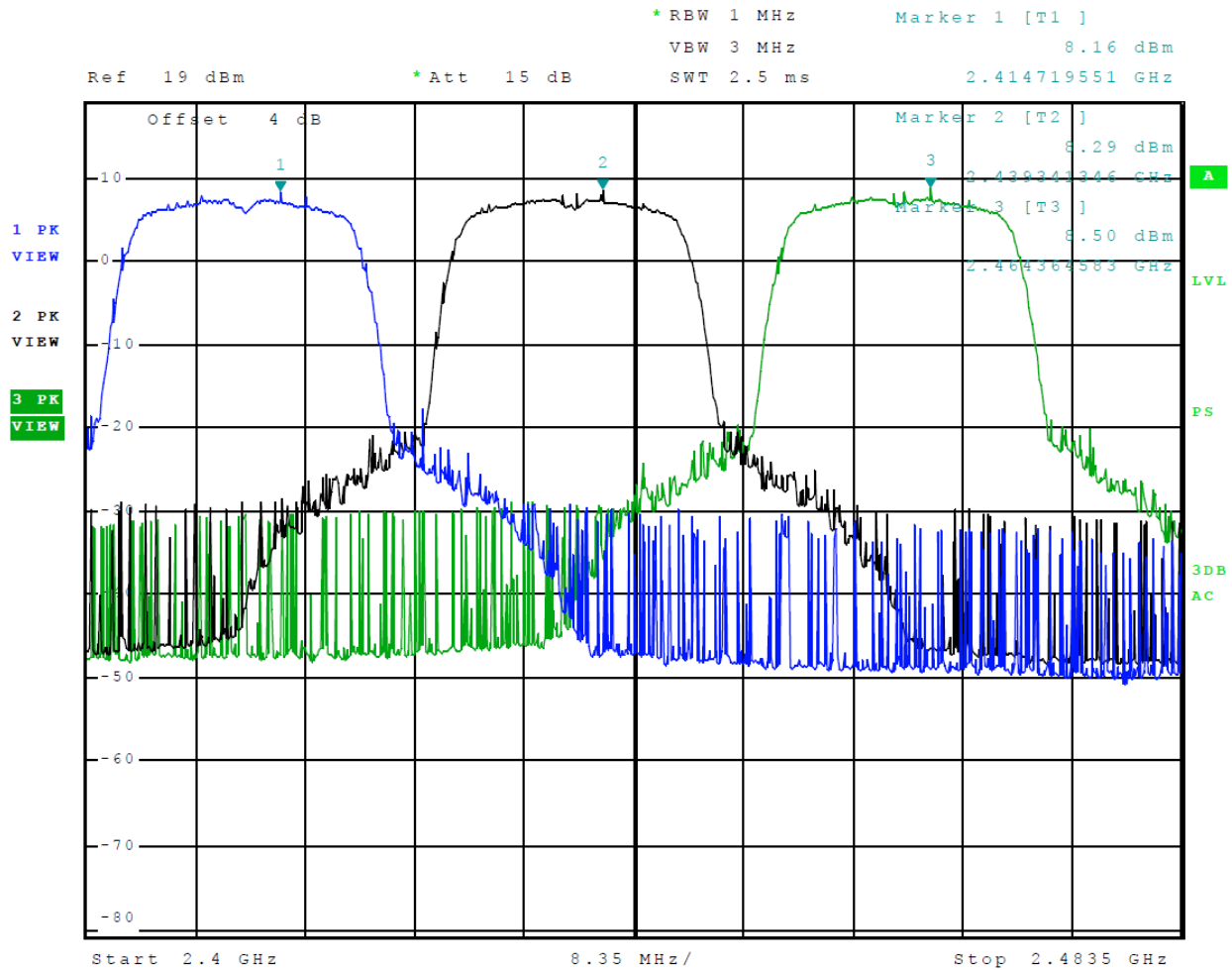
Figure 7 Plot of Transmitter Operation in 2412-2462 MHz Mode 8 802.11n
