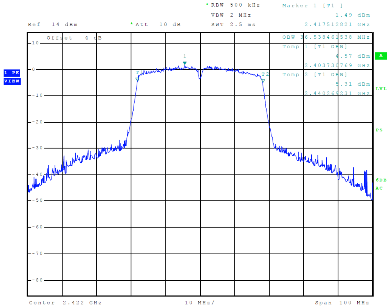
Figure 24 Plot of 99% Occupied Bandwidth Mode 8 802.11n40
