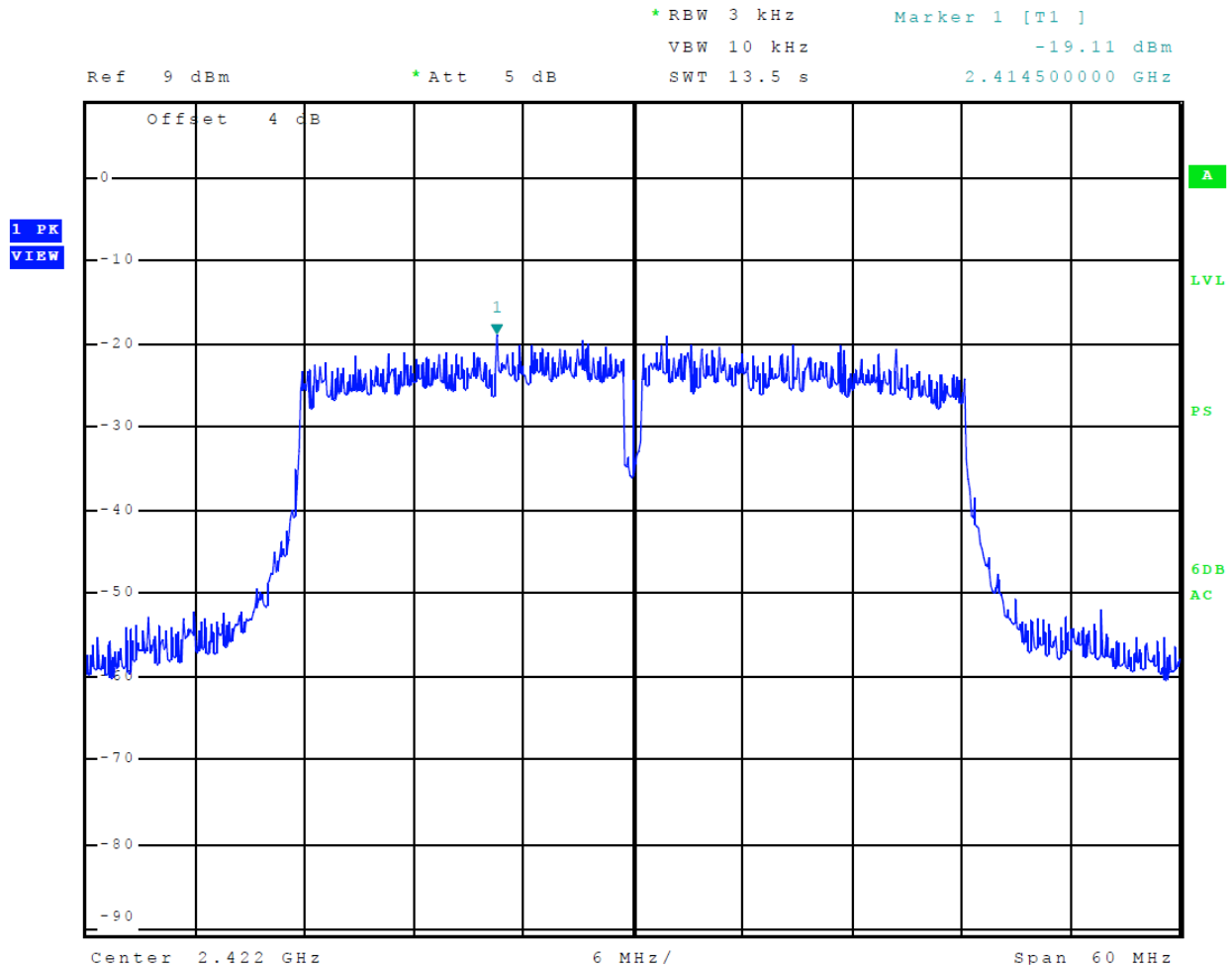
Figure 28 Plot of Transmitter Power Spectral Density Mode 8 802.11n40
