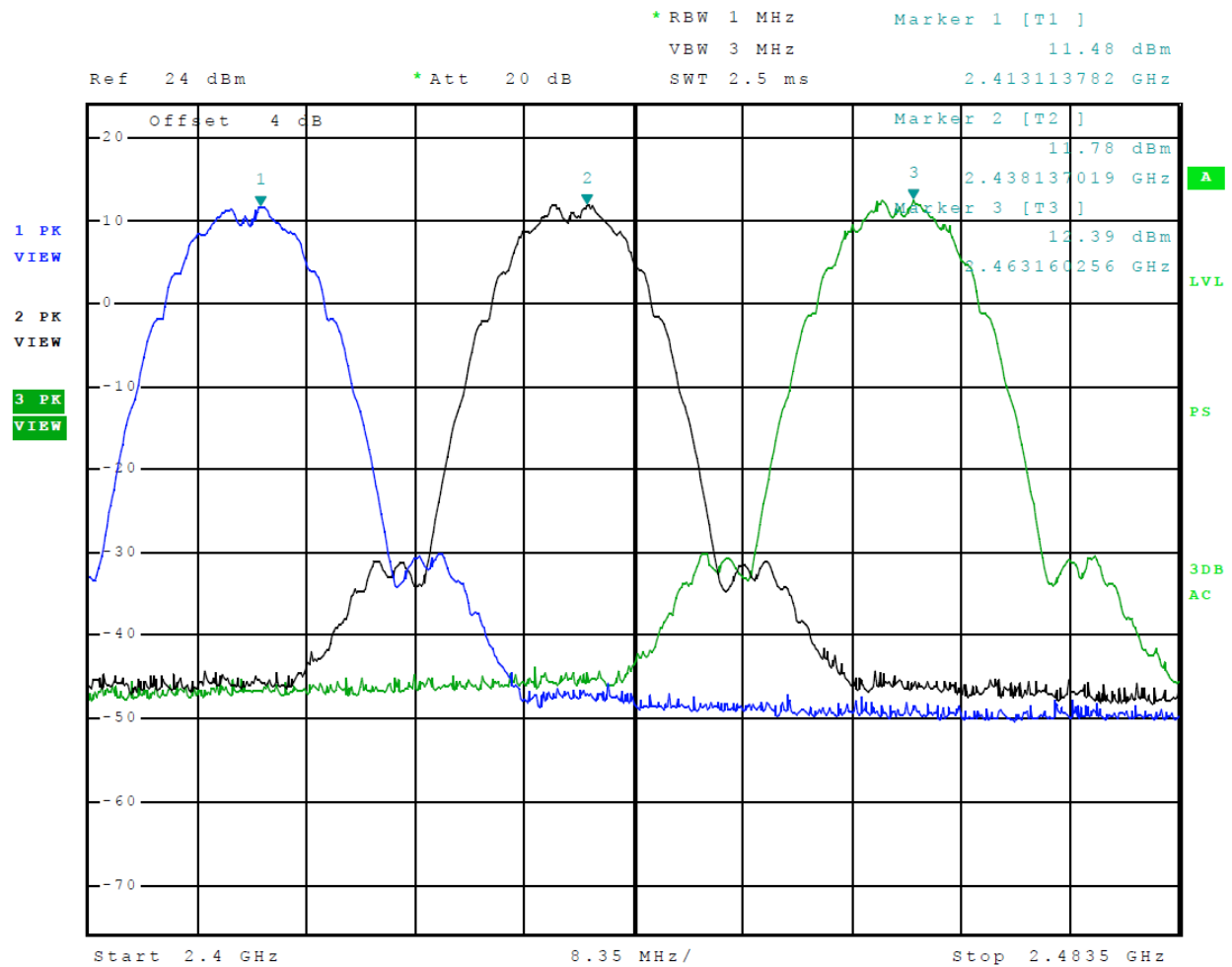
Figure 5 Plot of Transmitter Operation in 2412-2462 MHz Mode 6 802.11b
