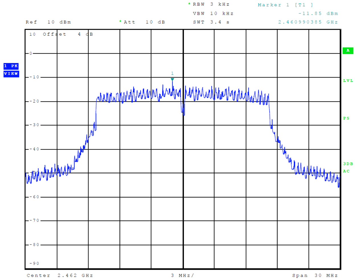
Figure 26 Plot of Transmitter Power Spectral Density Mode 7 802.11g
