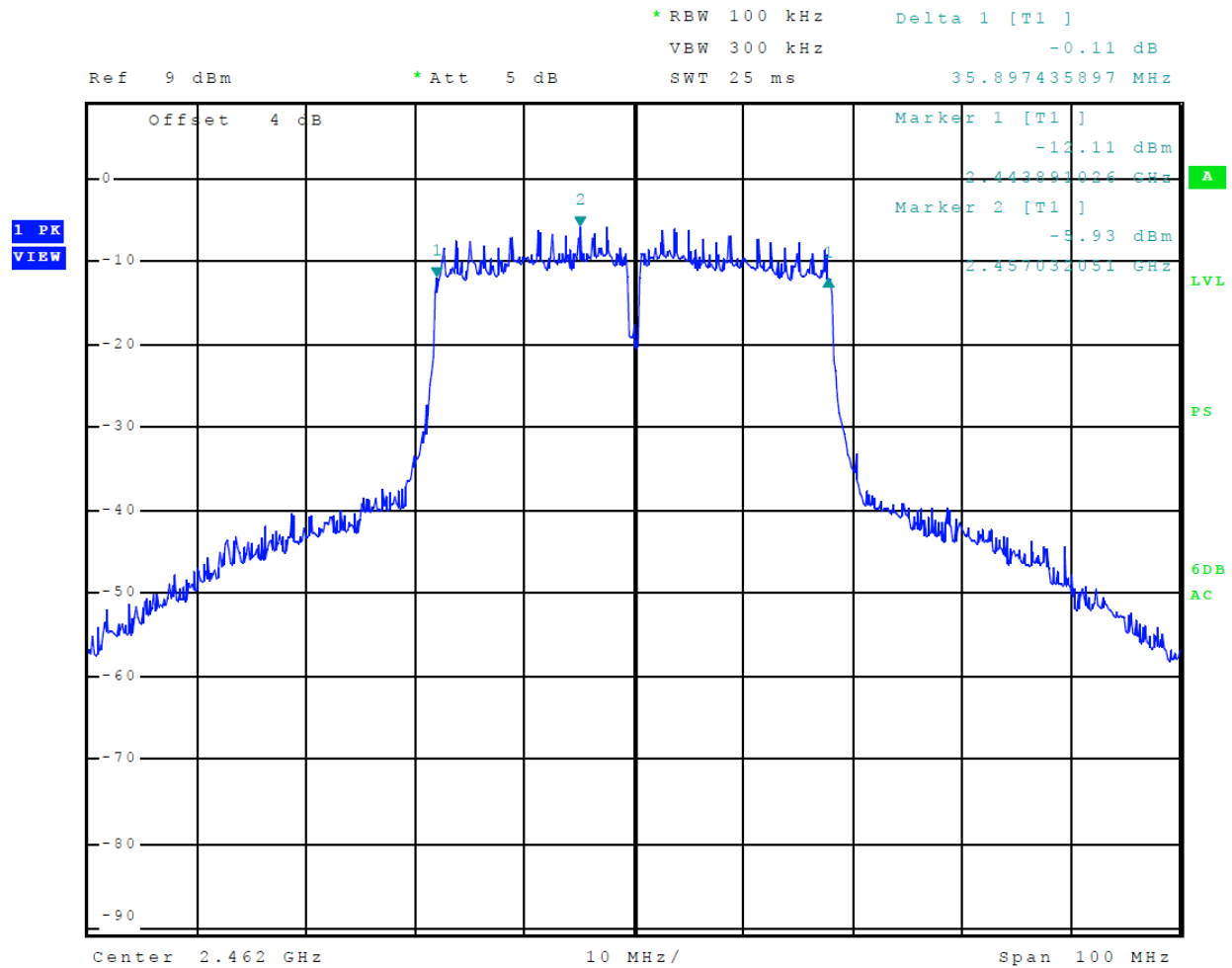
Figure 23 Plot of 6-dB Occupied Bandwidth Mode 8 802.11n40
