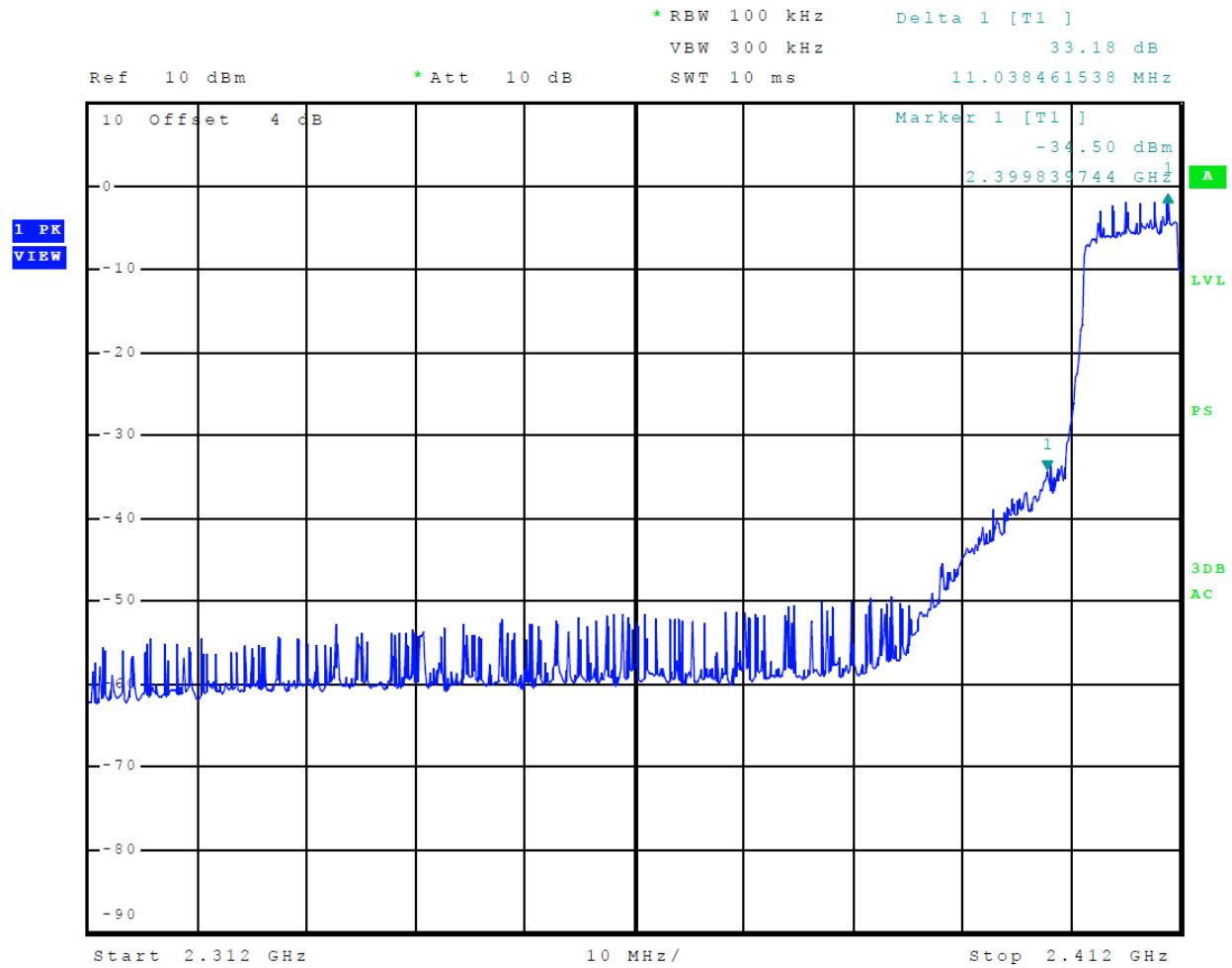
Figure 11 Plot of Transmitter Emissions Low Band Edge Mode 8 802.11n
