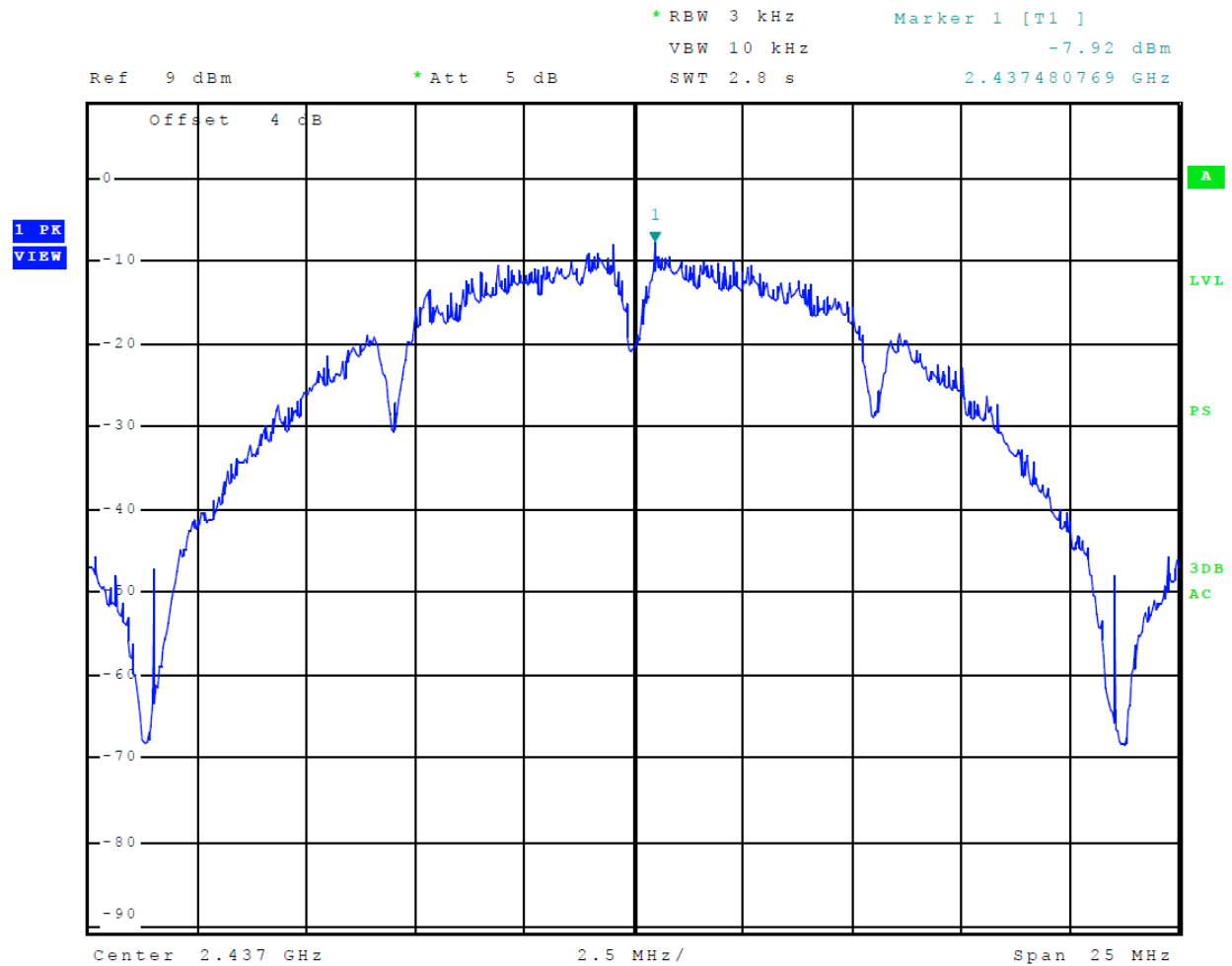
Figure 25 Plot of Transmitter Power Spectral Density Mode 6 802.11b
