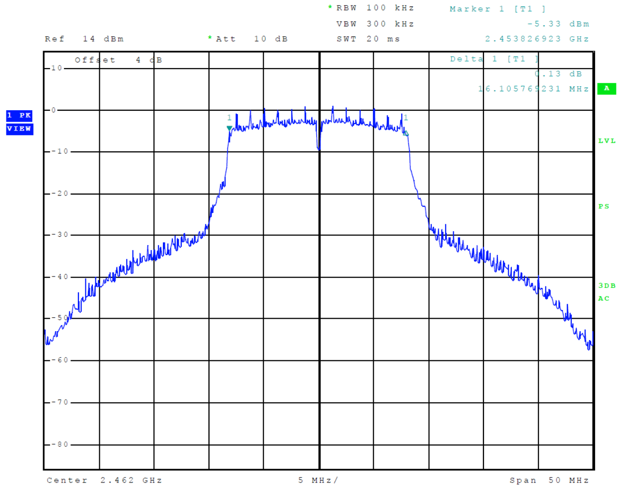
Figure 19 Plot of 6-dB Occupied Bandwidth Mode 7 802.11g
