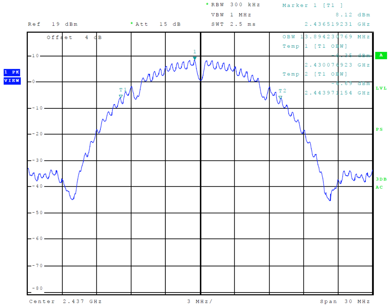
Figure 18 Plot of 99% Occupied Bandwidth Mode 6 802.11b
