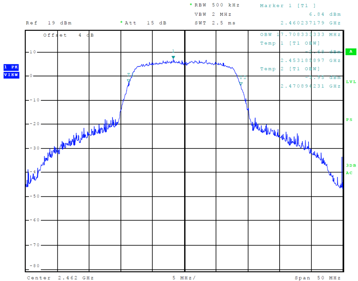
Figure 20 Plot of 99% Occupied Bandwidth Mode 7 802.11g
