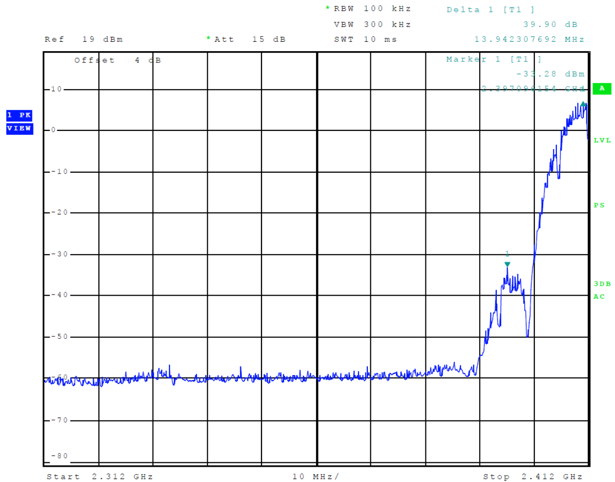
Figure 9 Plot of Transmitter Emissions Low Band Edge Mode 6 802.11b
