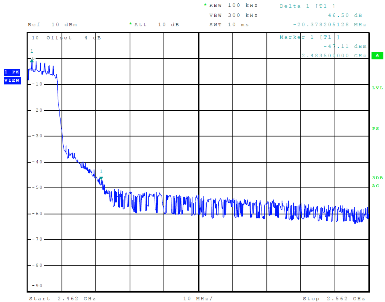
Figure 15 Plot of Transmitter Emissions High Band Edge Mode 8 802.11n
