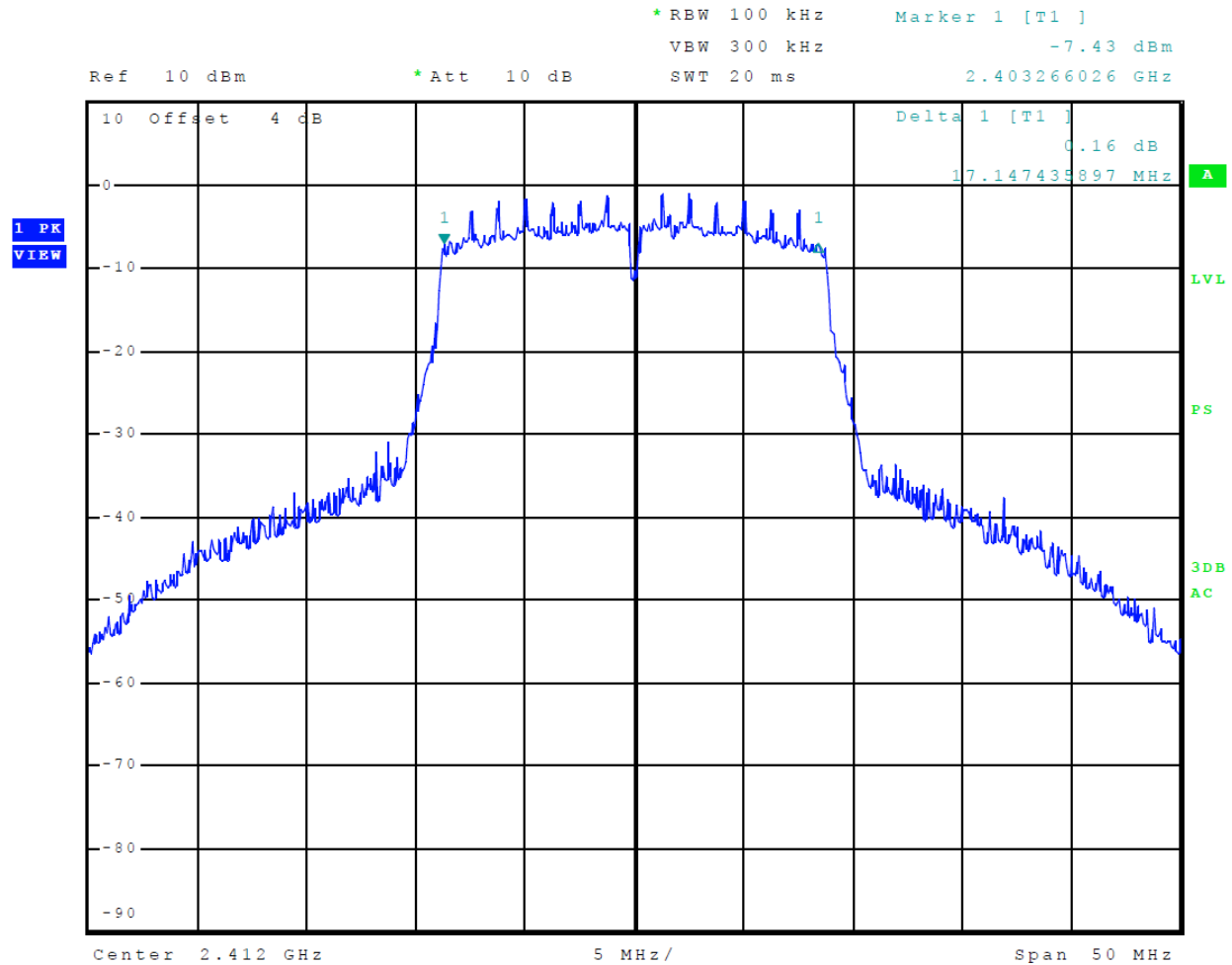
Figure 21 Plot of 6-dB Occupied Bandwidth Mode 8 802.11n
