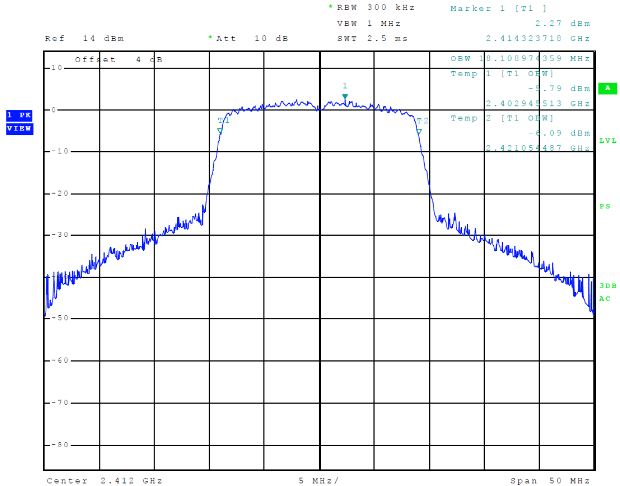
Figure 22 Plot of 99% Occupied Bandwidth Mode 8 802.11n
