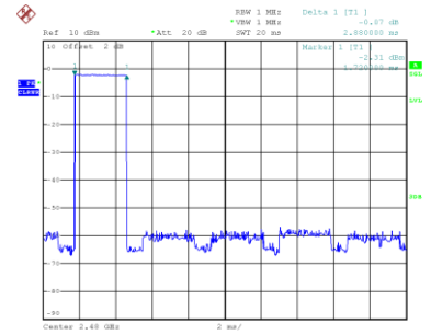
CH78-DH5
