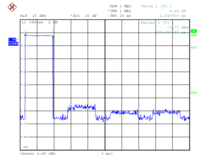
CH78-DH3
