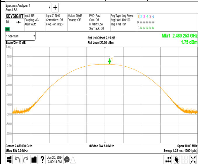
Channel 39 (2480MHz)
