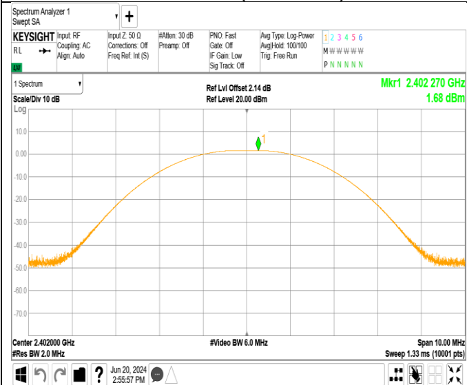
Channel 0 (2402MHz)
