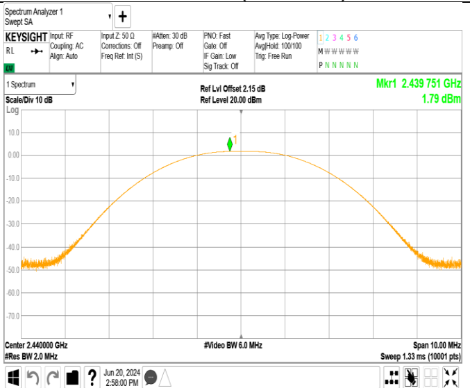
Channel 19 (2440MHz)
