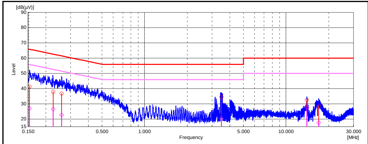
Neutral(N)
