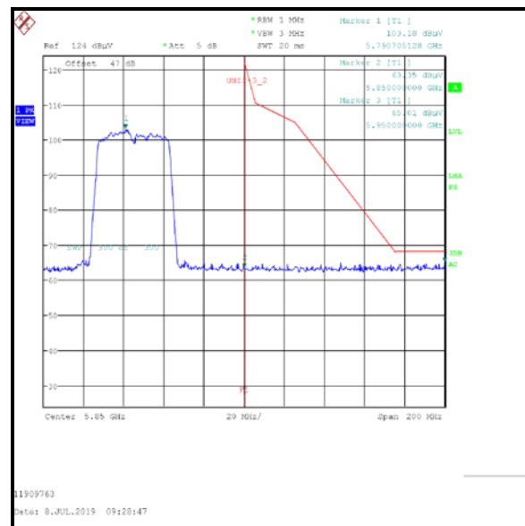
cUpper Band Edge Measurement
