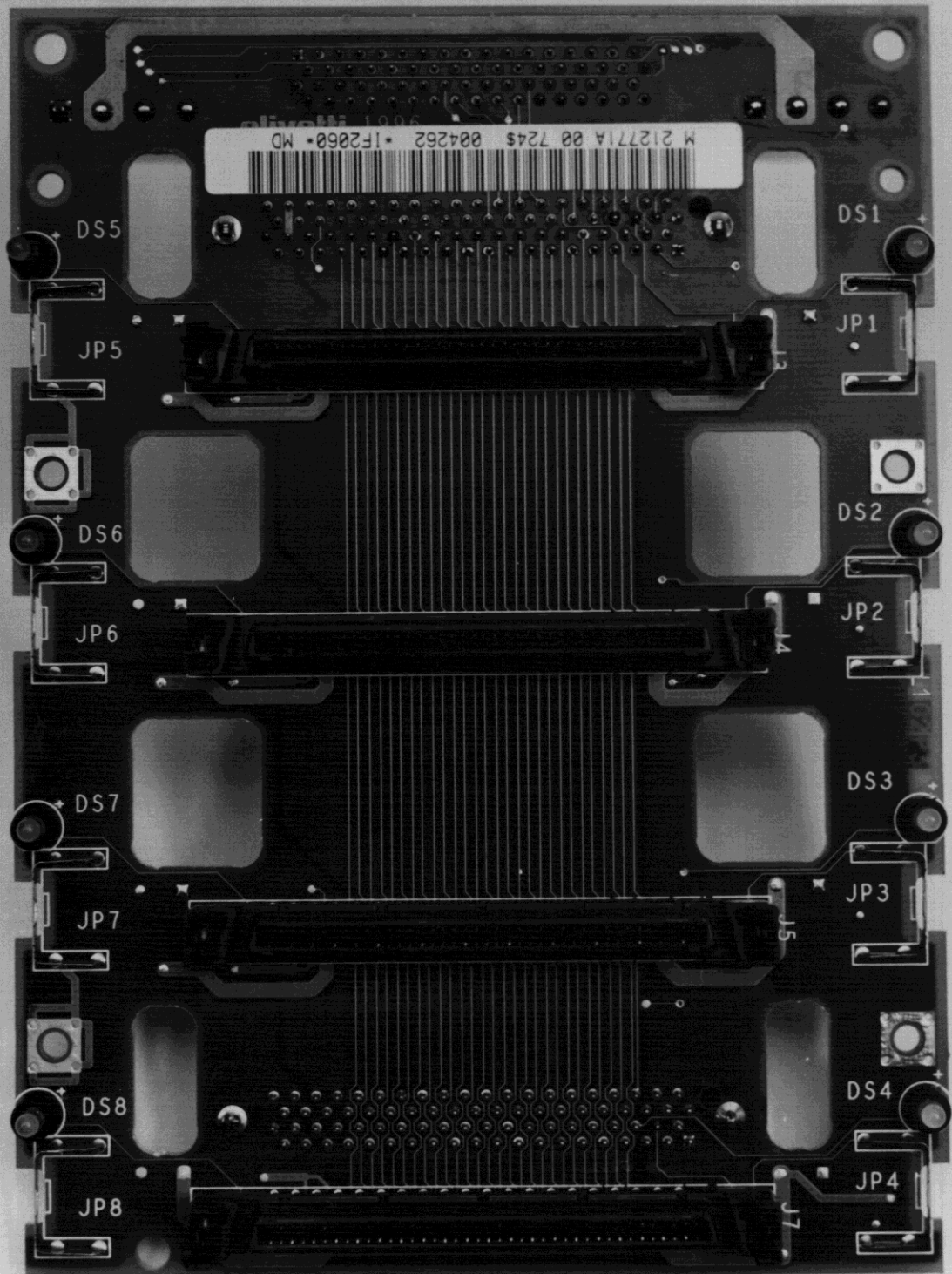
Fig. 8.7 IF 2060 interconnection board - Foil side
