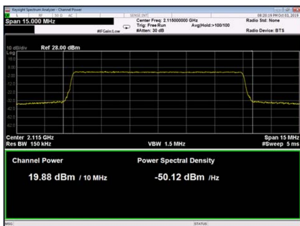
Figure 52 10MHz BW, 2115MHz
