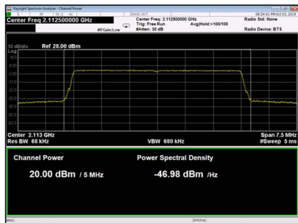
Figure 49 5MHz BW, 2112.5MHz
