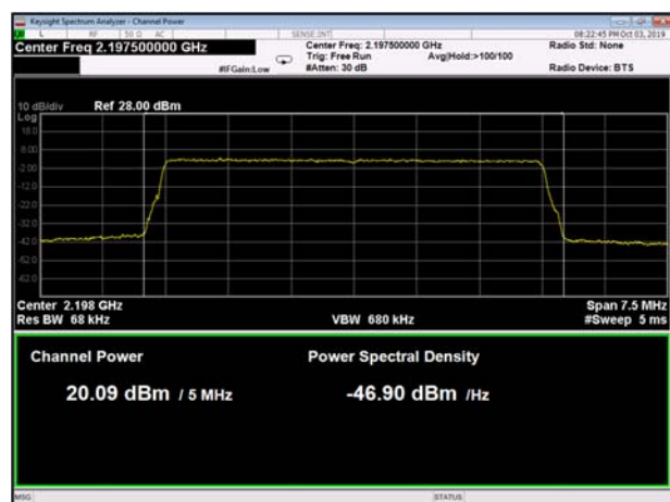
Figure 51 5MHz BW, 2197.5MHz
