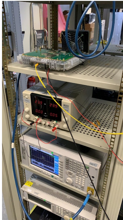
Conducted Test Set-Up
