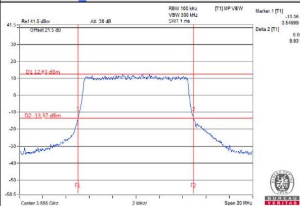
20MHz_Chain 2 / 16QAM / Low Channel
