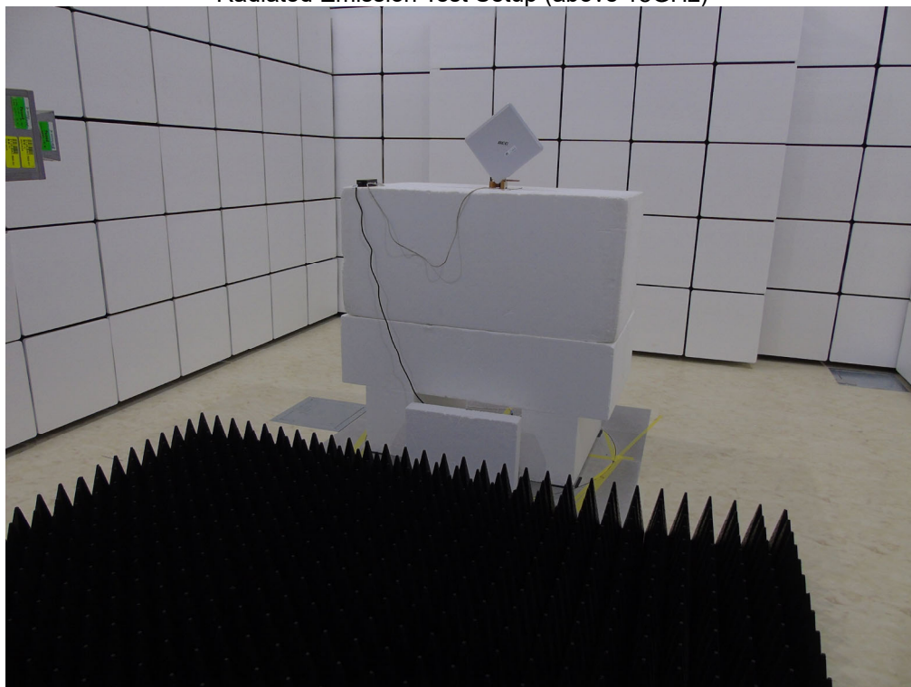
Radiated Emission Test Setup (above 18GHz)
