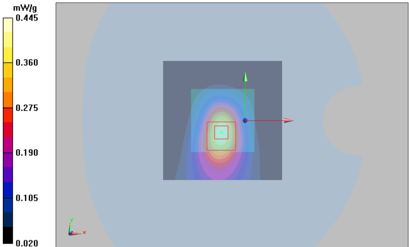
Figure 57 WCDMA Band V with Lenovo Y-450 Test Position 7 Channel 4183
