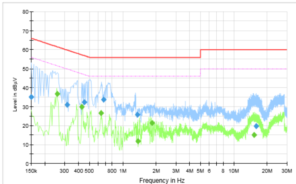
Fig.95 AC Power line Conducted Emission (Traffic), LE Coded
