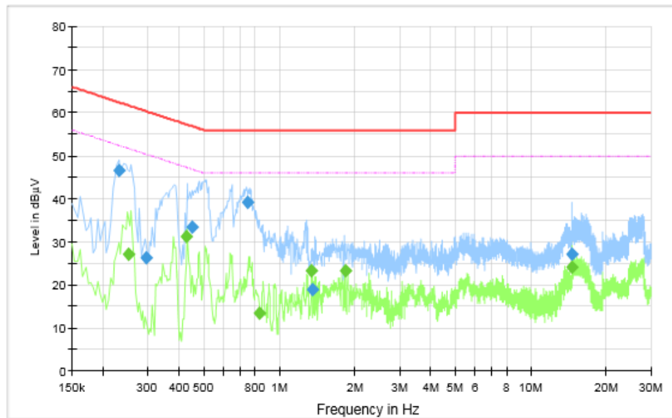
Fig.96 AC Power line Conducted Emission (Idle), LE Coded
