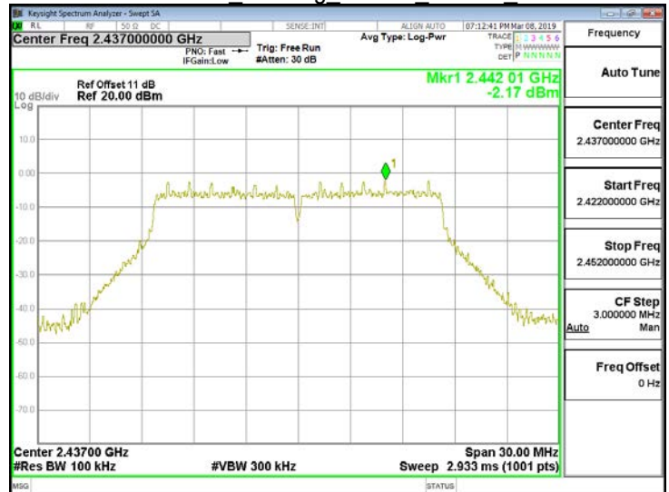
Reference Level 802.11g 20MHz Chain0 2437MHz
