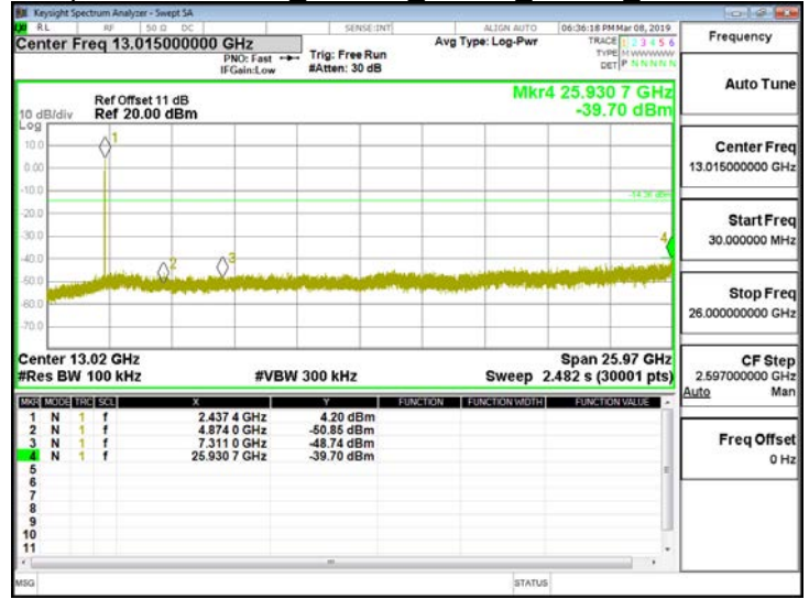
Spurious Emission 802.11b 20MHz Chain0 2437MHz
