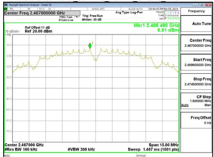
Reference Level 802.11b 20MHz Chain0 2467MHz
