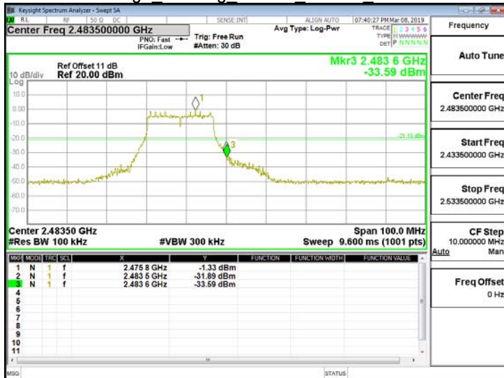
Band Edge 802.11g 20MHz Chain0 2472MHz
