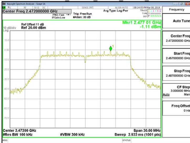
Reference Level 802.11n 20MHz Chain0 2472MHz
