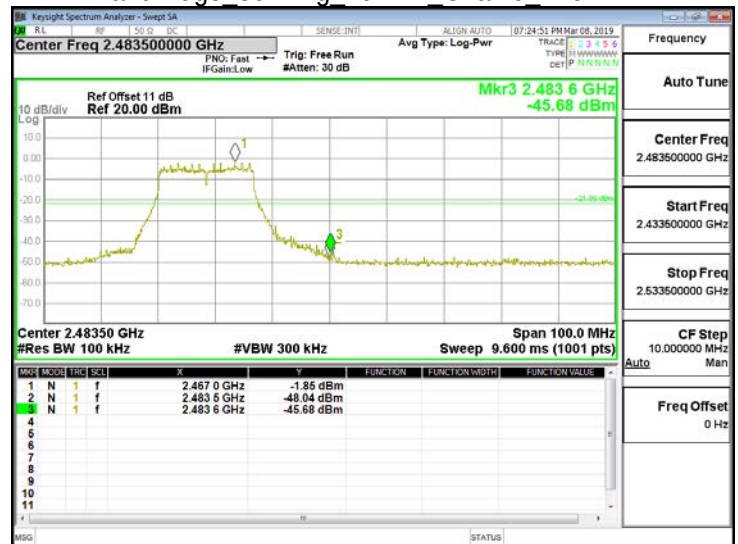
Band Edge 802.11g 20MHz Chain0 2462MHz
