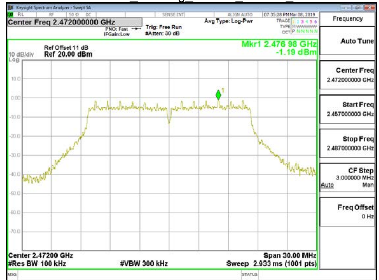
Reference Level 802.11g 20MHz Chain0 2472MHz
