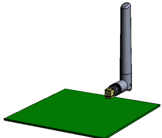
On edge of ground plane, bent 90 degrees
