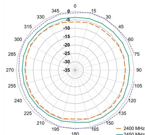
XY-Plane Gain
