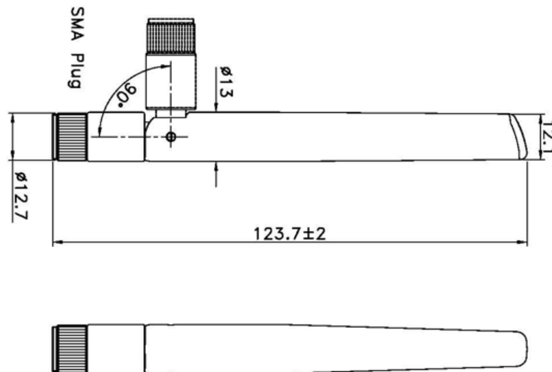
Figure 2. Antenna Dimensions
