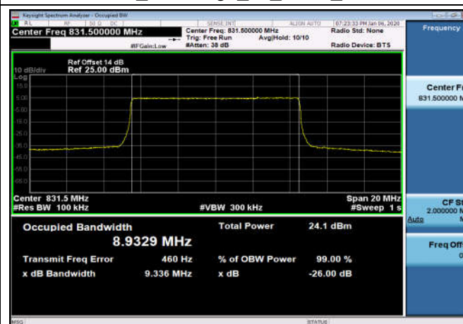
FDD26_MidRange_10_831.5_QPSK
