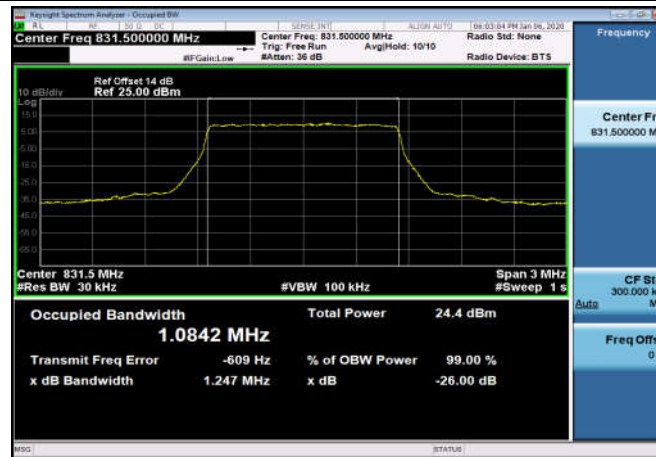
FDD26_MidRange_3MHz_831.5MHz_QPSK
