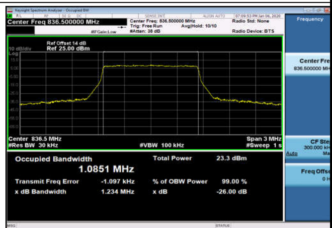
FDD05_MidRange_3_836.5_Q16
