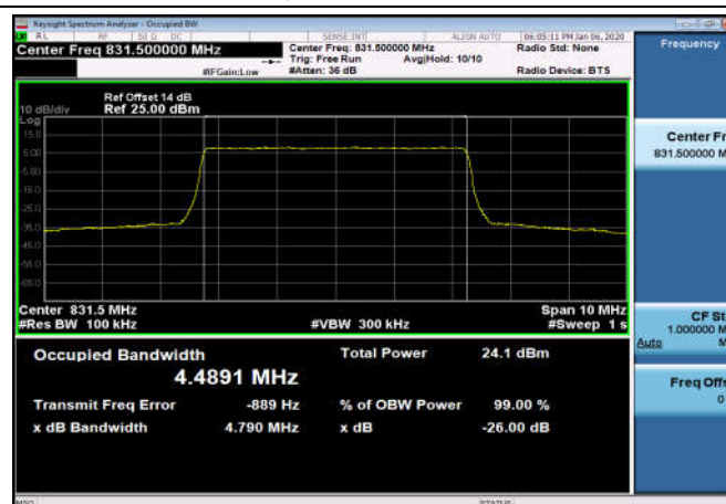
FDD26_MidRange_5MHz_831.5MHz_QPSK
