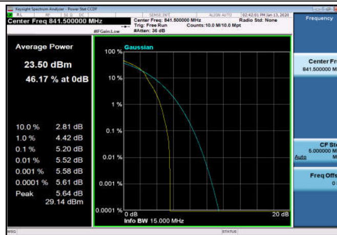
FDD26_HighRange_15MHz_841.5_OneRB _high_Q16
