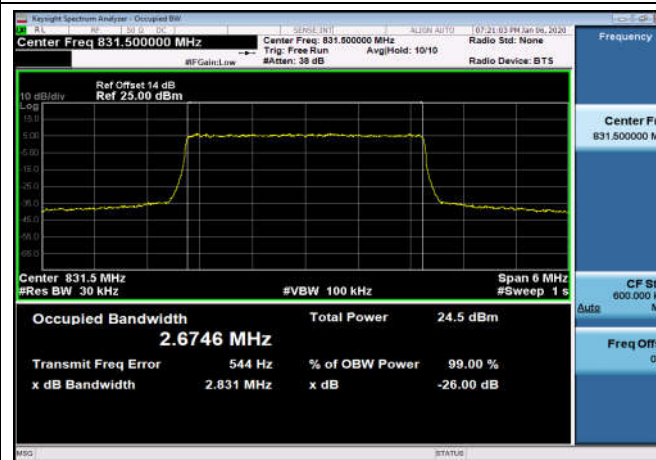
FDD26_MidRange_5_831.5_QPSK
