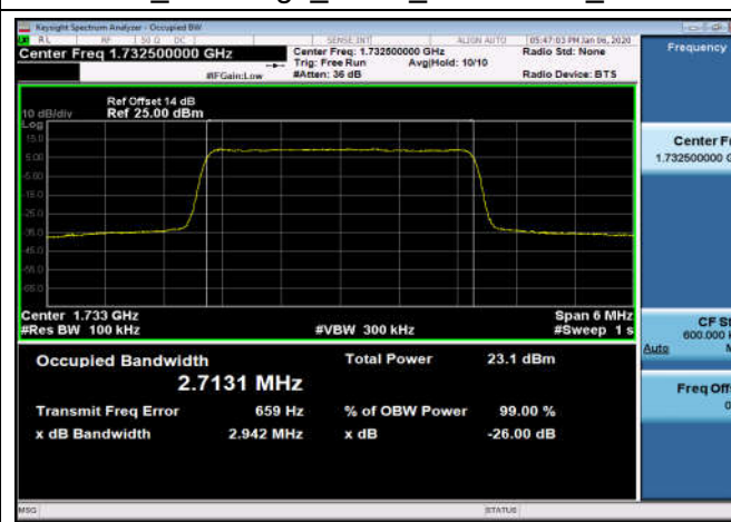
FDD04_MidRange_3MHz_1732.5MHz_QPSK
