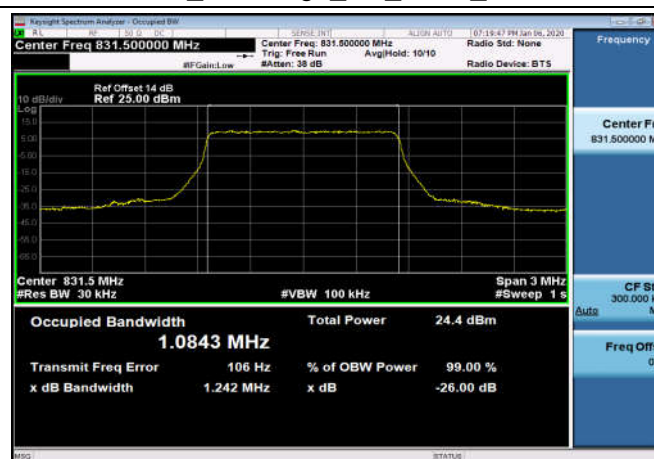
FDD26_MidRange_1.4_831.5_QPSK
