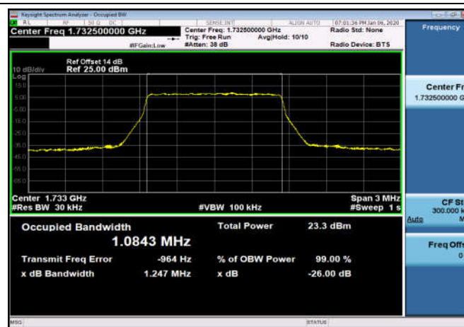
FDD04_MidRange_3_1732.5_QPSK
