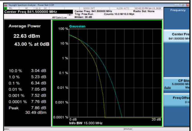
FDD26_HighRange_15MHz_841.5_fullRB _Q16
