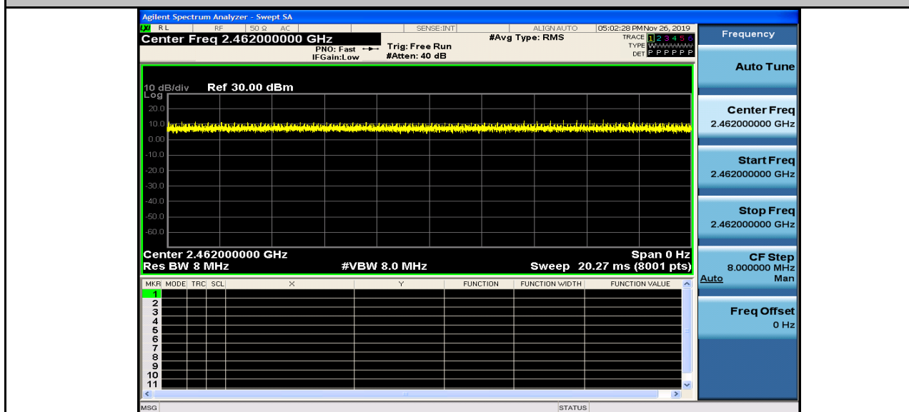
Duty Cycle_11G_2462_Ant1
