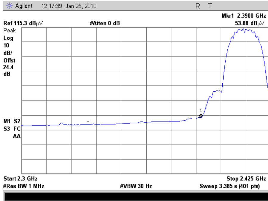
Plot 82. 802.11b Lower Band Edge, Channel 1, Average (24dBi Grid Antenna)
