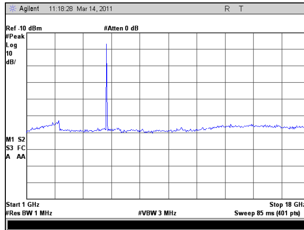
Plot 166. Radiated Spurious Emissions, Mid Channel, 1 GHz – 18 GHz, 802.11n HT10
