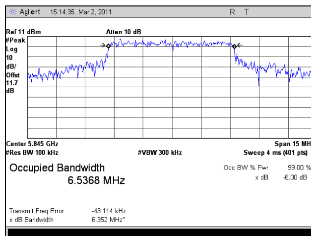
Plot 27. 6 dB Occupied Bandwidth, High Channel, 802.11n HT8, Port 1
