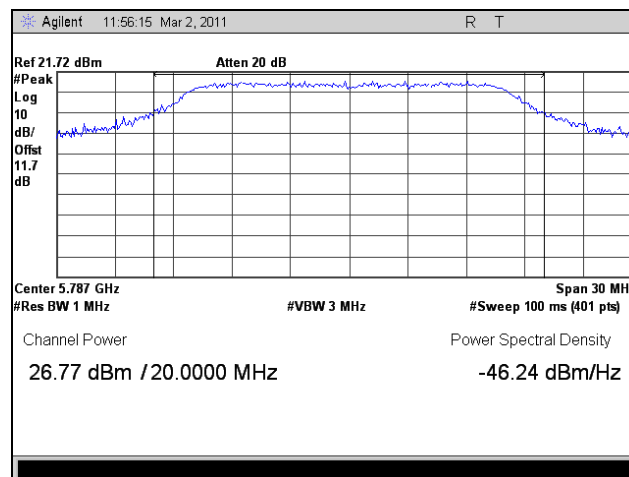
Plot 122. Peak Power Output, Mid Channel, 802.11n HT20, Port 1
