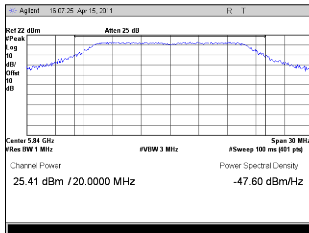
Plot 99. Peak Power Output, 802.11a 20 MHz, High Channel
