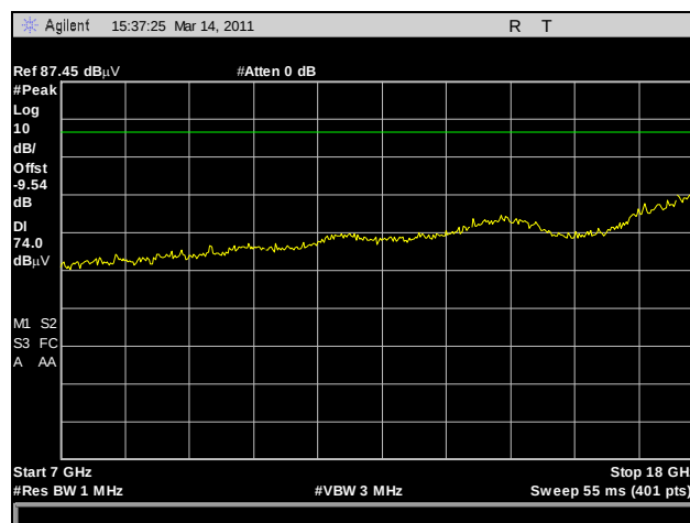
Plot 198. Radiated Harmonics, High Channel, 7 GHz – 18 GHz, Peak, 802.11n HT5
