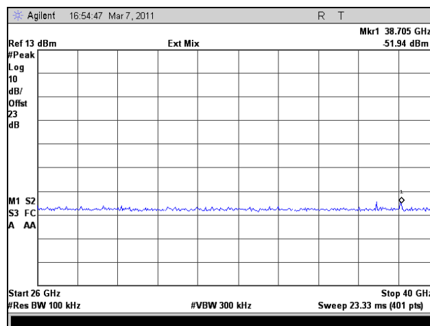
Plot 264. Conducted Spurious Emissions, Mid Channel, 26 GHz – 40 GHz, 802.11n HT8, Port 1
