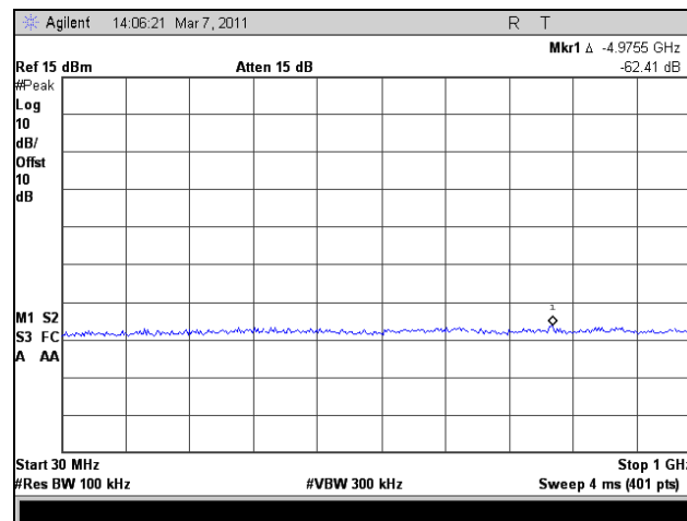
Plot 250. Conducted Spurious Emissions, Low Channel, 30 MHz – 1 GHz, 802.11n HT5, Port 2
