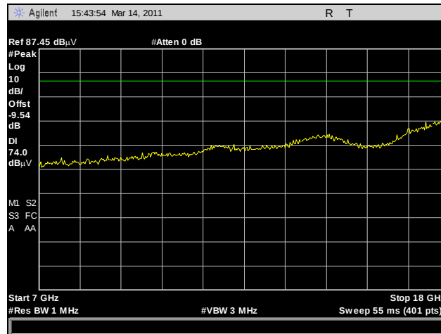
Plot 196. Radiated Harmonics, Mid Channel, 7 GHz – 18 GHz, Peak, 802.11n HT5
