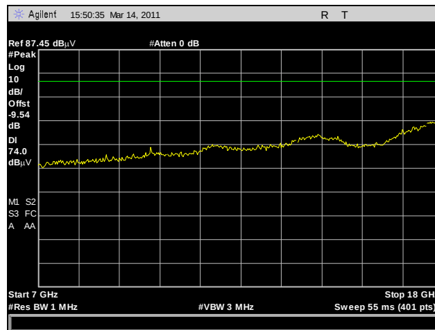
Plot 194. Radiated Harmonics, Low Channel, 7 GHz – 18 GHz, Peak, 802.11n HT5
