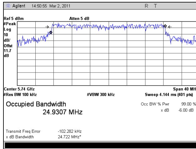
Plot 46. 6 dB Occupied Bandwidth, Low Channel, 802.11n HT30, Port 2
