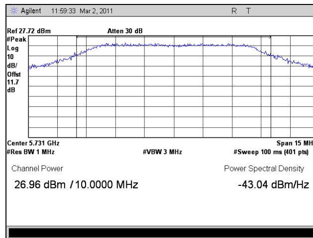
Plot 115. Peak Power Output, Low Channel, 802.11n HT10, Port 1
