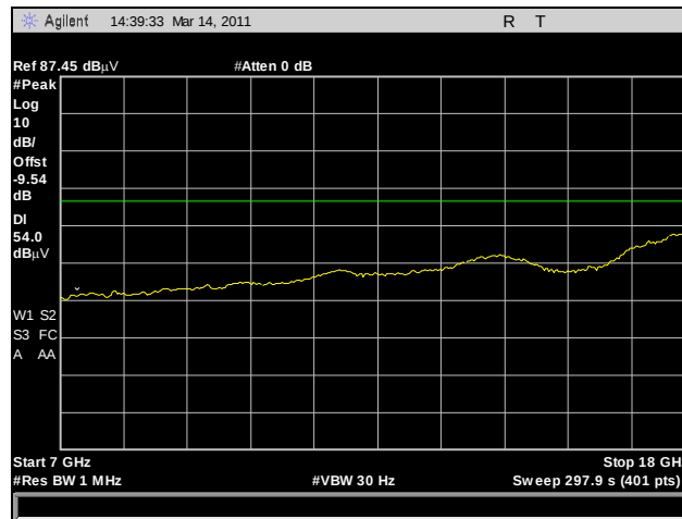
Plot 211. Radiated Harmonics, Low Channel, 7 GHz – 18 GHz, Average, 802.11n HT20
