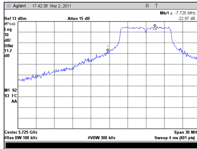
Plot 361. Conducted Band Edge, Low Channel, 802.11n HT10, Port 1
