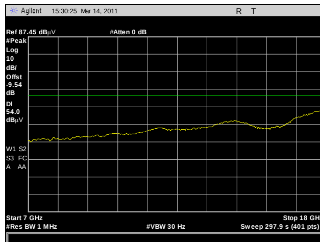
Plot 201. Radiated Harmonics, Mid Channel, 7 GHz – 18 GHz, Average, 802.11n HT8
