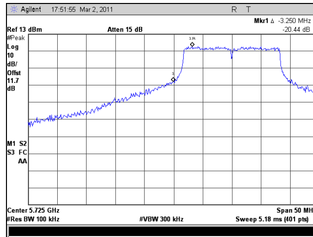
Plot 365. Conducted Band Edge, Low Channel, 802.11n HT20, Port 1
