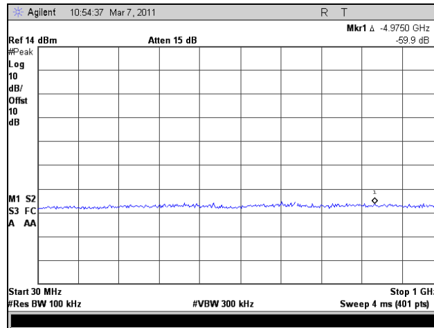
Plot 262. Conducted Spurious Emissions, Mid Channel, 30 MHz – 1 GHz, 802.11n HT8, Port 1
