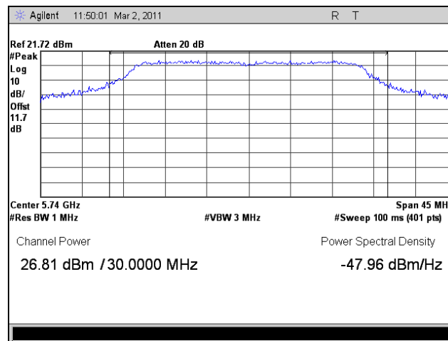
Plot 127. Peak Power Output, Low Channel, 802.11n HT30, Port 1
