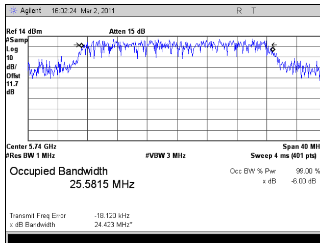
Plot 85. 99% Occupied Bandwidth, Low Channel, 802.11n HT30, Port 1
