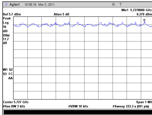
Plot 383. Peak Power Spectral Density, Low Channel, 802.11n HT5, Port 1
