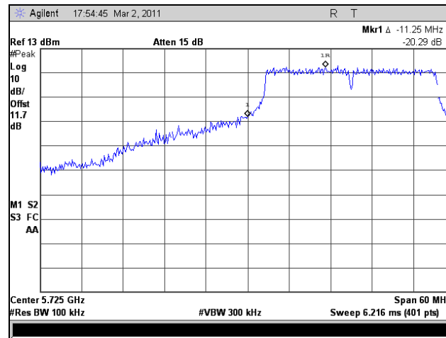
Plot 369. Conducted Band Edge, Low Channel, 802.11n HT30, Port 1
