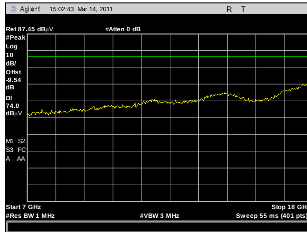
Plot 208. Radiated Harmonics, Mid Channel, 7 GHz – 18 GHz, Peak, 802.11n HT10
