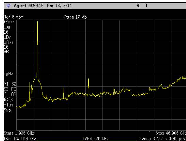
Plot 238. Conducted Spurious Emissions, Mid Channel, 802.11a 40 MHz, 1 GHz – 40 GHz
