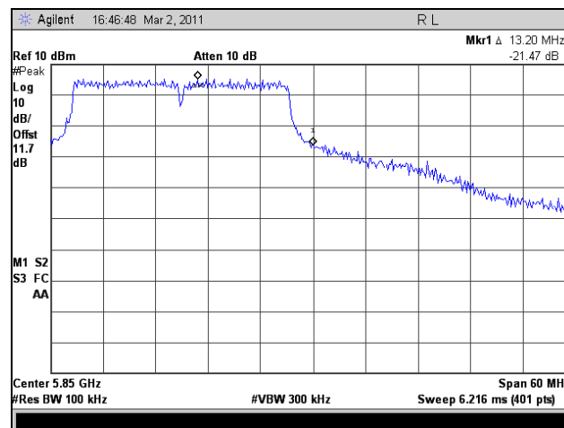
Plot 370. Conducted Band Edge, High Channel, 802.11n HT30, Port 1
