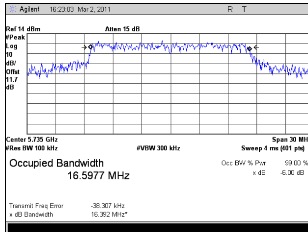
Plot 37. 6 dB Occupied Bandwidth, Low Channel, 802.11n HT20, Port 1
