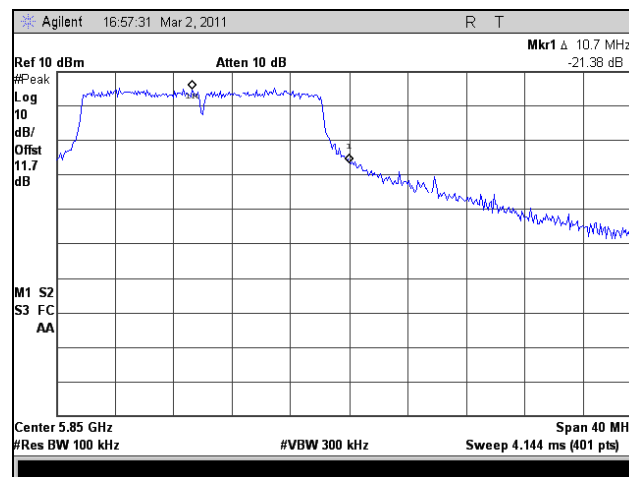
Plot 366. Conducted Band Edge, High Channel, 802.11n HT20, Port 1
