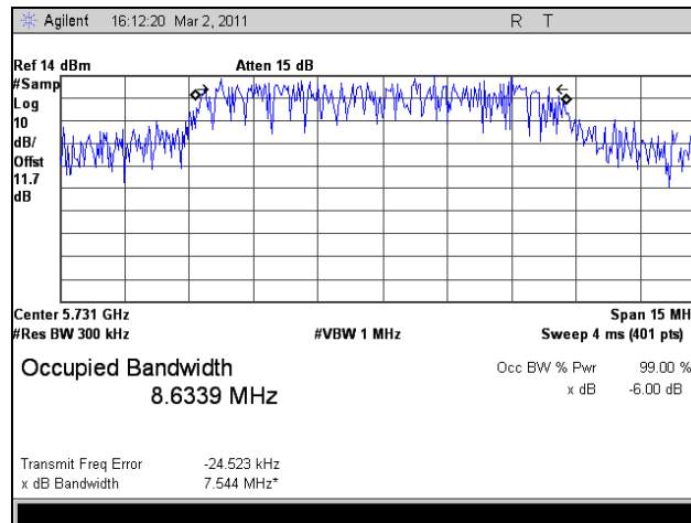
Plot 73. 99% Occupied Bandwidth, Low Channel, 802.11n HT10, Port 1
