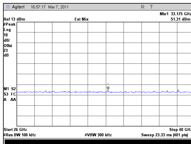
Plot 282. Conducted Spurious Emissions, Mid Channel, 26 GHz – 40 GHz, 802.11n HT10, Port 1
