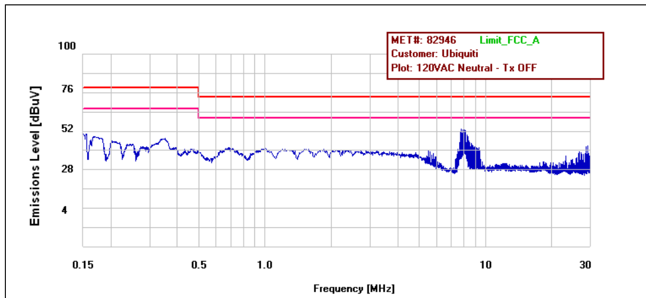
Plot 4. Conducted Emission, Neutral Line Plot, GME PSU
