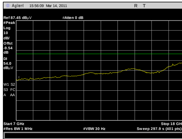
Plot 193. Radiated Harmonics, Low Channel, 7 GHz – 18 GHz, Average, 802.11n HT5
