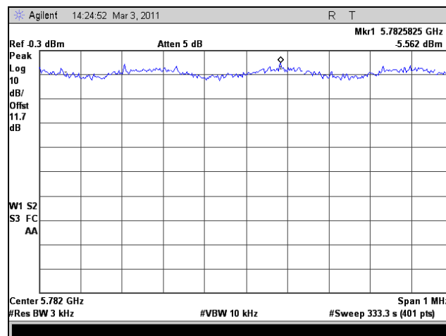
Plot 403. Peak Power Spectral Density, Mid Channel, 802.11n HT20, Port 1
