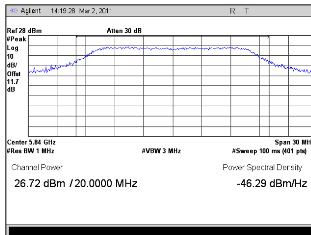
Plot 126. Peak Power Output, High Channel, 802.11n HT20, Port 2
