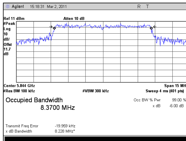
Plot 33. 6 dB Occupied Bandwidth, High Channel, 802.11n HT10, Port 1
