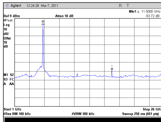
Plot 323. Conducted Spurious Emissions, Low Channel, 1 GHz – 26 GHz, 802.11n HT30, Port 2
