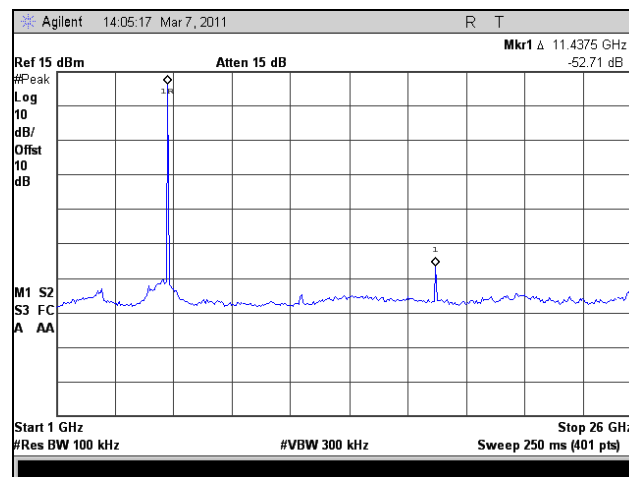
Plot 251. Conducted Spurious Emissions, Low Channel, 1 GHz – 26 GHz, 802.11n HT5, Port 2
