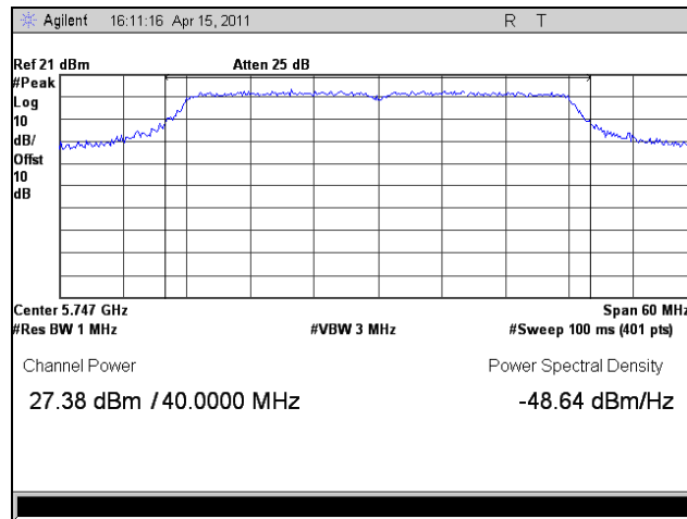
Plot 100. Peak Power Output, 802.11a 40 MHz, Low Channel
