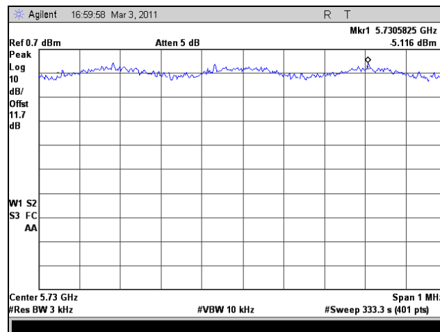
Plot 402. Peak Power Spectral Density, Low Channel, 802.11n HT20, Port 2
