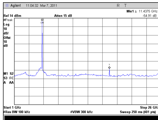
Plot 260. Conducted Spurious Emissions, Low Channel, 1 GHz – 26 GHz, 802.11n HT8, Port 1
