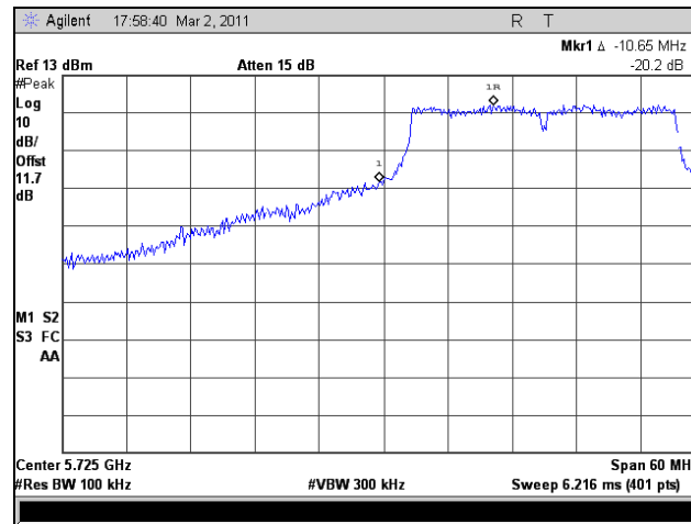
Plot 371. Conducted Band Edge, Low Channel, 802.11n HT30, Port 2
