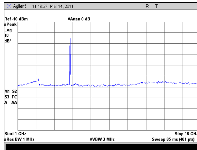
Plot 164. Radiated Spurious Emissions, Low Channel, 1 GHz – 18 GHz, 802.11n HT10
