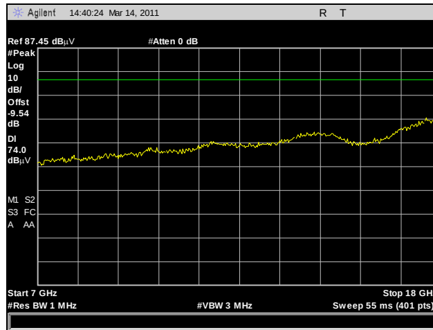
Plot 214. Radiated Harmonics, Mid Channel, 7 GHz – 18 GHz, Peak, 802.11n HT20
