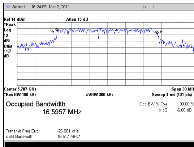
Plot 38. 6 dB Occupied Bandwidth, Mid Channel, 802.11n HT20, Port 1
