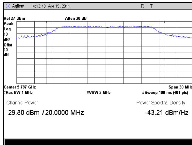
Plot 98. Peak Power Output, 802.11a 20 MHz, Mid Channel
