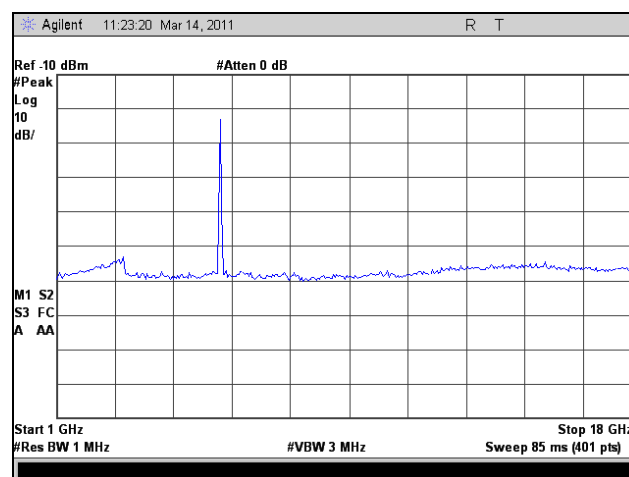
Plot 180. Radiated Spurious Emissions, High Channel, 1 GHz – 18 GHz, 802.11n HT30
