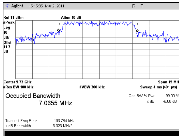
Plot 25. 6 dB Occupied Bandwidth, Low Channel, 802.11n HT8, Port 1
