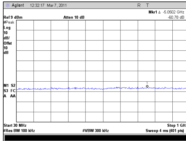
Plot 307. Conducted Spurious Emissions, Mid Channel, 30 MHz – 1 GHz, 802.11n HT20, Port 2
