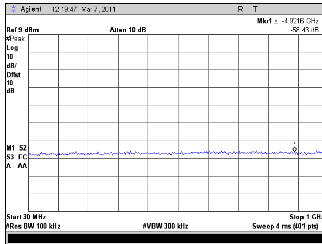
Plot 325. Conducted Spurious Emissions, Mid Channel, 30 MHz – 1 GHz, 802.11n HT30, Port 2
