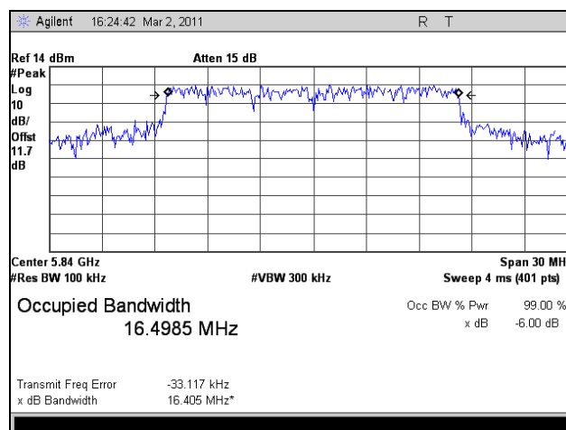
Plot 39. 6 dB Occupied Bandwidth, High Channel, 802.11n HT20, Port 1
