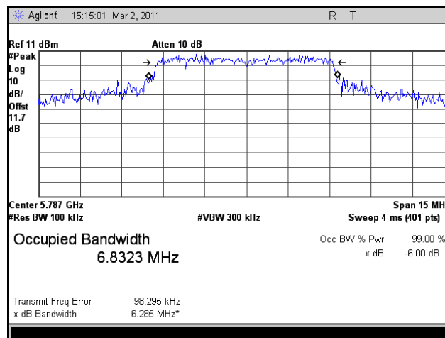
Plot 26. 6 dB Occupied Bandwidth, Mid Channel, 802.11n HT8, Port 1
