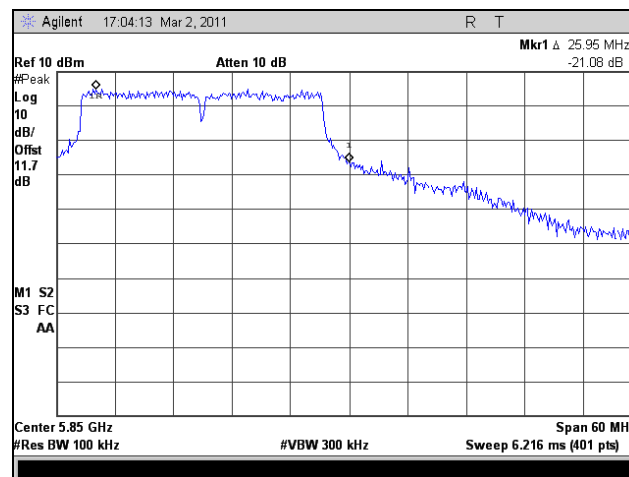
Plot 372. Conducted Band Edge, High Channel, 802.11n HT30, Port 2
