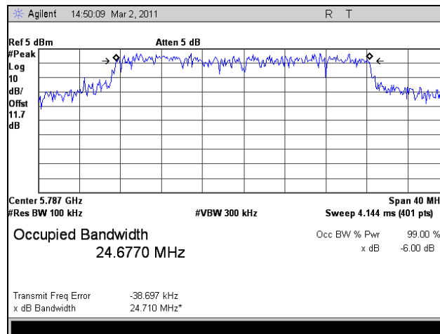
Plot 47. 6 dB Occupied Bandwidth, Mid Channel, 802.11n HT30, Port 2
