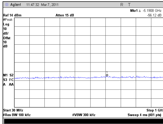
Plot 334. Conducted Spurious Emissions, Mid Channel, 30 MHz – 1 GHz, 802.11n HT40, Port 1
