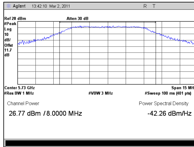
Plot 109. Peak Power Output, Low Channel, 802.11n HT8, Port 1
