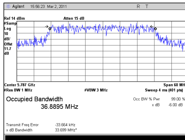
Plot 95. 99% Occupied Bandwidth, Mid Channel, 802.11n HT40, Port 2
