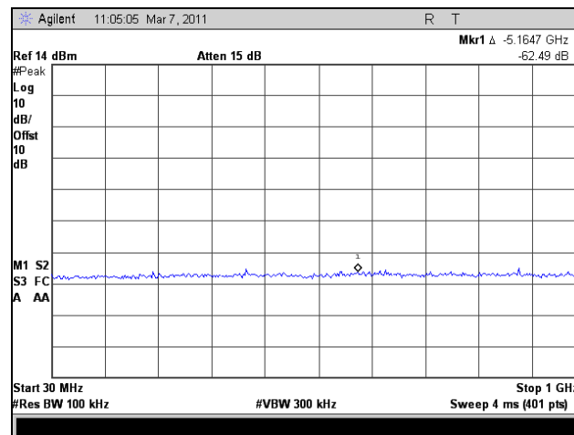
Plot 259. Conducted Spurious Emissions, Low Channel, 30 MHz – 1 GHz, 802.11n HT8, Port 1
