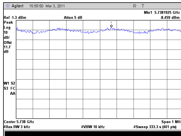
Plot 414. Peak Power Spectral Density, Low Channel, 802.11n HT40, Port 2
