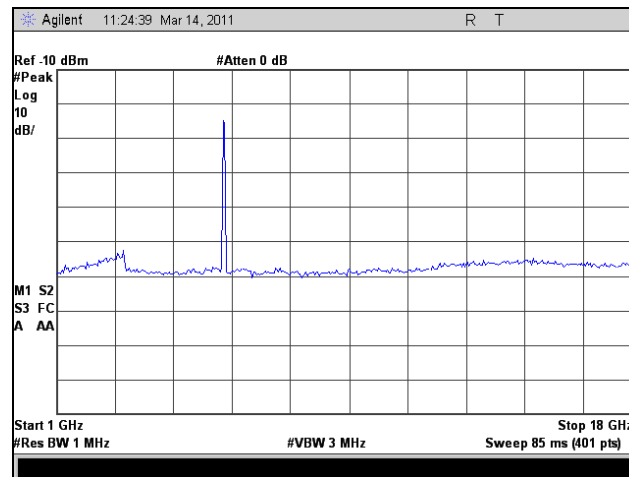
Plot 176. Radiated Spurious Emissions, Low Channel, 1 GHz – 18 GHz, 802.11n HT30
