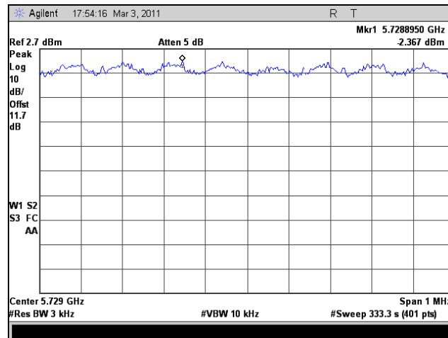
Plot 390. Peak Power Spectral Density, Low Channel, 802.11n HT8, Port 2
