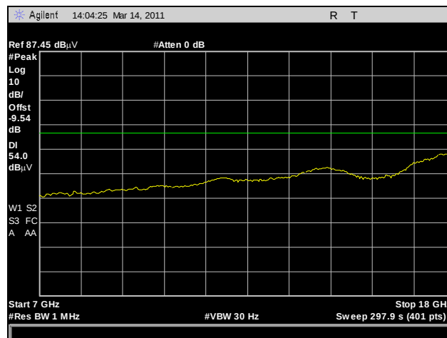
Plot 225. Radiated Harmonics, Mid Channel, 7 GHz – 18 GHz, Average, 802.11n HT40
