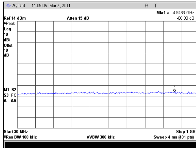
Plot 280. Conducted Spurious Emissions, Mid Channel, 30 MHz – 1 GHz, 802.11n HT10, Port 1
