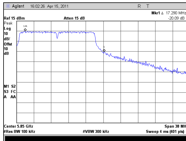
Plot 350. Conducted Band Edge, High Channel, 802.11a 20 MHz
