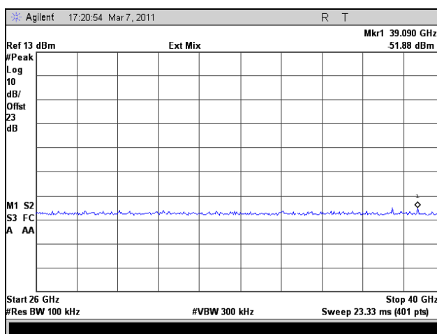
Plot 258. Conducted Spurious Emissions, High Channel, 26 GHz – 40 GHz, 802.11n HT5, Port 2
