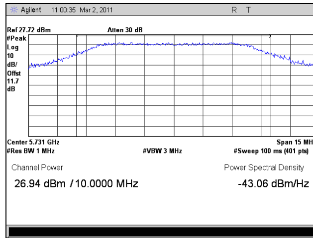
Plot 118. Peak Power Output, Low Channel, 802.11n HT10, Port 2
