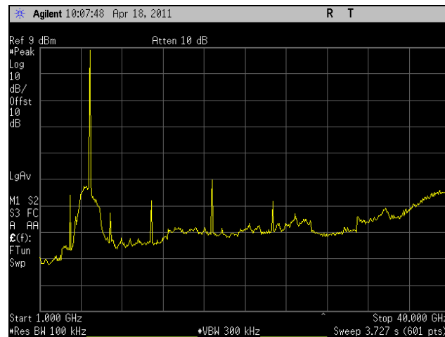
Plot 232. Conducted Spurious Emissions, Mid Channel, 802.11a 20 MHz, 1 GHz – 40 GHz
