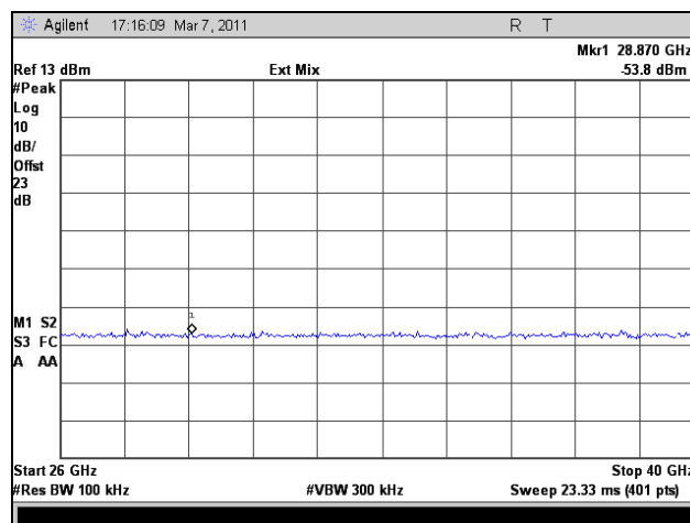
Plot 291. Conducted Spurious Emissions, Mid Channel, 26 GHz – 40 GHz, 802.11n HT10, Port 2
