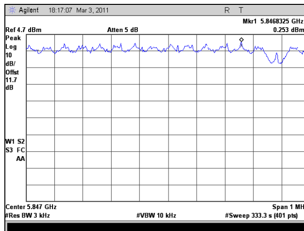
Plot 388. Peak Power Spectral Density, High Channel, 802.11n HT5, Port 2
