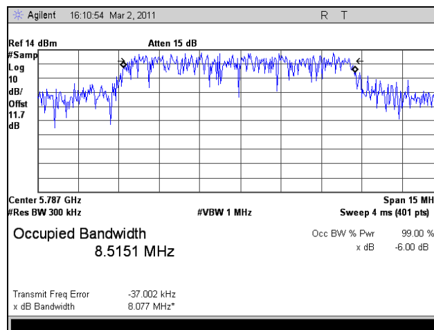
Plot 74. 99% Occupied Bandwidth, Mid Channel, 802.11n HT10, Port 1
