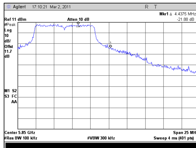
Plot 362. Conducted Band Edge, High Channel, 802.11n HT10, Port 1
