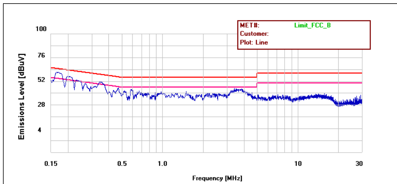
Plot 9. Conducted Emissions, 15.207(a), Phase Line, Cetus PSU
