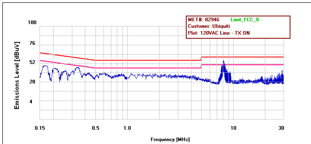
Plot 11. Conducted Emissions, 15.207(a), Phase Line, GME PSU
