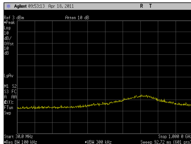
Plot 239. Conducted Spurious Emissions, High Channel, 802.11a 40 MHz, 30 MHz – 1 GHz
