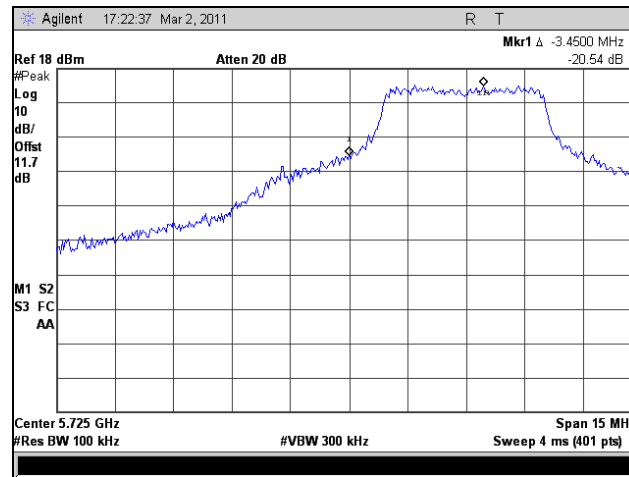
Plot 353. Conducted Band Edge, Low Channel, 802.11n HT5, Port 1
