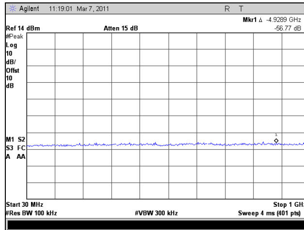
Plot 298. Conducted Spurious Emissions, Mid Channel, 30 MHz – 1 GHz, 802.11n HT20, Port 1
