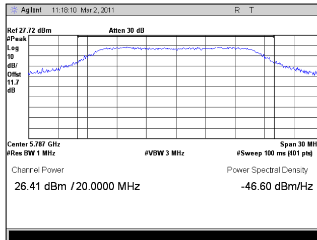
Plot 125. Peak Power Output, Mid Channel, 802.11n HT20, Port 2
