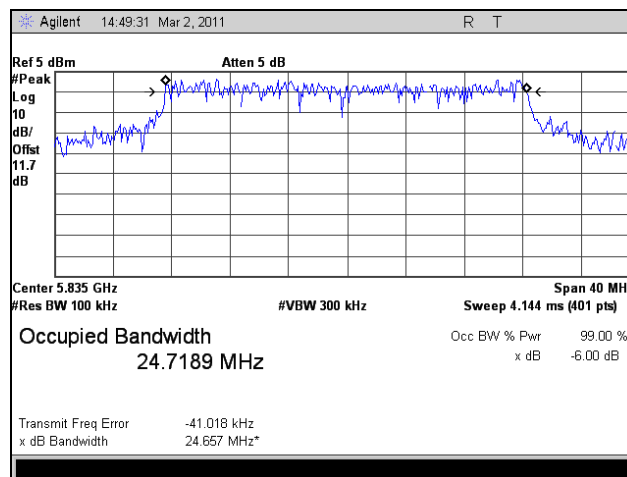
Plot 48. 6 dB Occupied Bandwidth, High Channel, 802.11n HT30, Port 2
