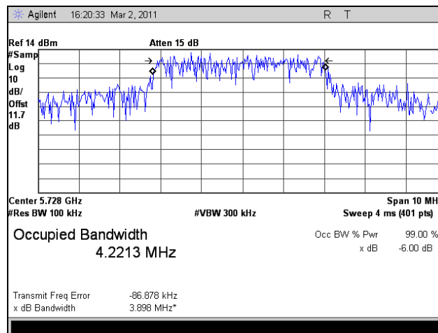
Plot 61. 99% Occupied Bandwidth, Low Channel, 802.11n HT5, Port 1
