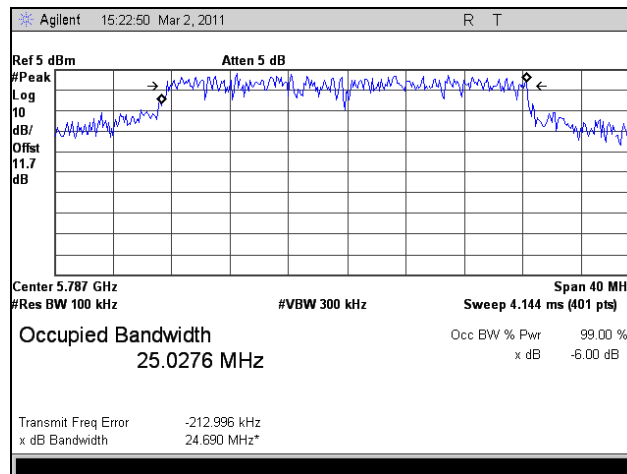
Plot 44. 6 dB Occupied Bandwidth, Mid Channel, 802.11n HT30, Port 1
