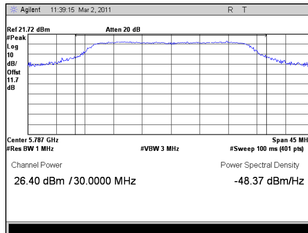
Plot 131. Peak Power Output, Mid Channel, 802.11n HT30, Port 2
