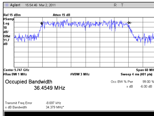
Plot 94. 99% Occupied Bandwidth, Low Channel, 802.11n HT40, Port 2
