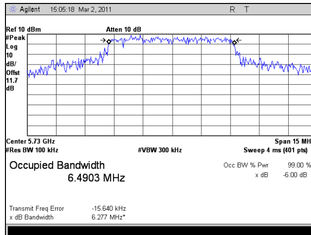
Plot 28. 6 dB Occupied Bandwidth, Low Channel, 802.11n HT8, Port 2
