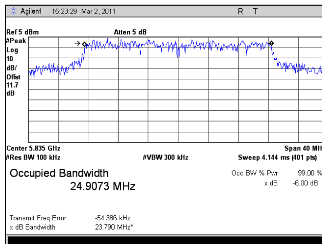
Plot 45. 6 dB Occupied Bandwidth, High Channel, 802.11n HT30, Port 1
