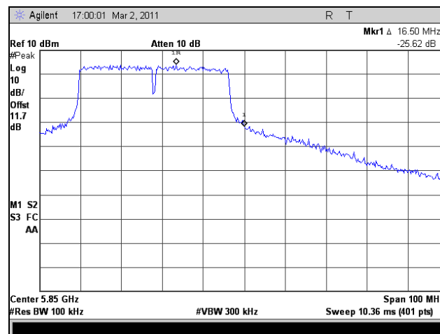
Plot 374. Conducted Band Edge, High Channel, 802.11n HT40, Port 1
