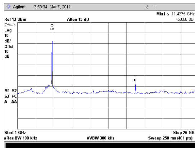
Plot 287. Conducted Spurious Emissions, Low Channel, 1 GHz – 26 GHz, 802.11n HT10, Port 2
