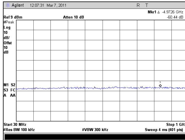
Plot 343. Conducted Spurious Emissions, Mid Channel, 30 MHz – 1 GHz, 802.11n HT40, Port 2
