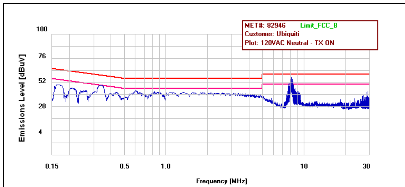
Plot 12. Conducted Emissions, 15.207(a), Neutral Line, GME PSU
