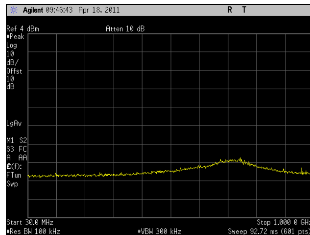
Plot 235. Conducted Spurious Emissions, Low Channel, 802.11a 40 MHz, 30 MHz – 1 GHz
