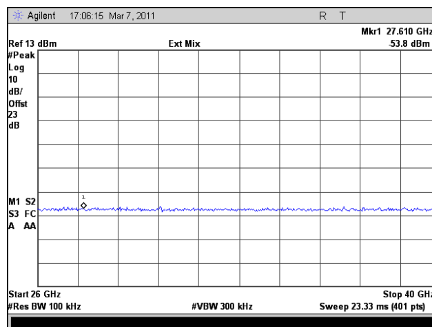
Plot 336. Conducted Spurious Emissions, Mid Channel, 26 GHz – 40 GHz, 802.11n HT40, Port 1
