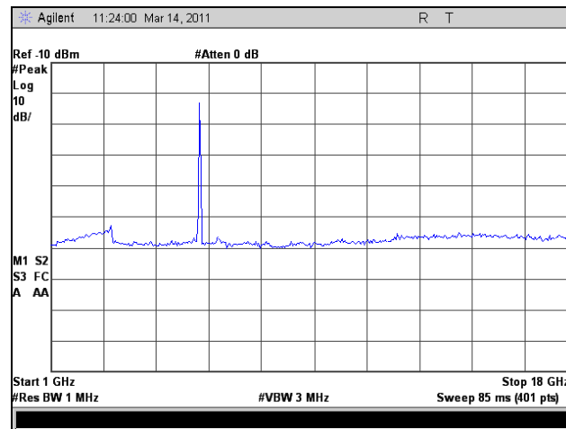
Plot 178. Radiated Spurious Emissions, Mid Channel, 1 GHz – 18 GHz, 802.11n HT30
