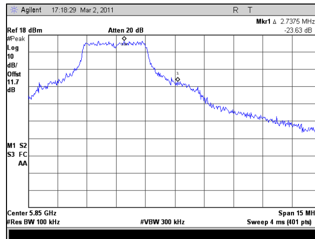
Plot 354. Conducted Band Edge, High Channel, 802.11n HT5, Port 1
