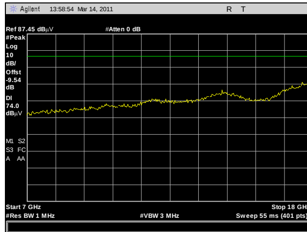
Plot 226. Radiated Harmonics, Mid Channel, 7 GHz – 18 GHz, Peak, 802.11n HT40
