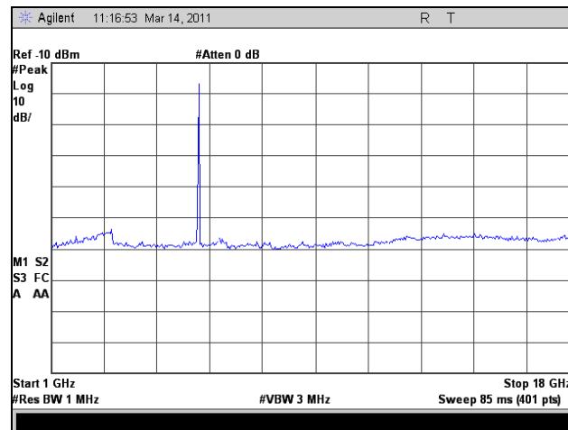
Plot 158. Radiated Spurious Emissions, Low Channel, 1 GHz – 18 GHz, 802.11n HT8
