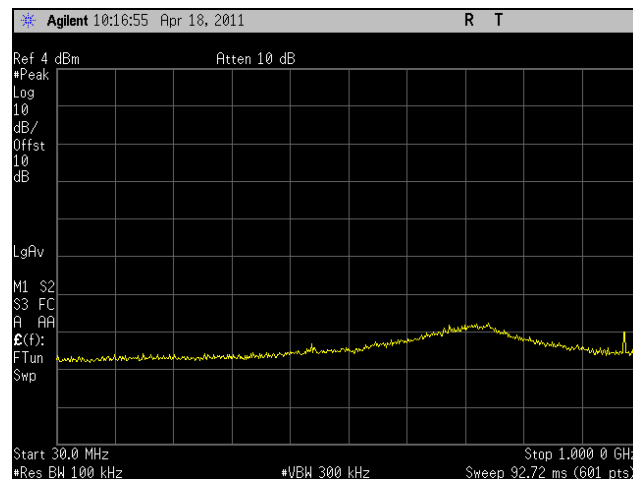
Plot 233. Conducted Spurious Emissions, High Channel, 802.11a 20 MHz, 30 MHz – 1 GHz
