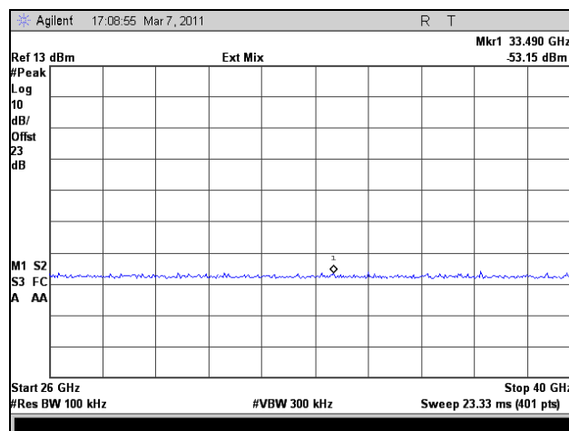
Plot 345. Conducted Spurious Emissions, Mid Channel, 26 GHz – 40 GHz, 802.11n HT40, Port 2
