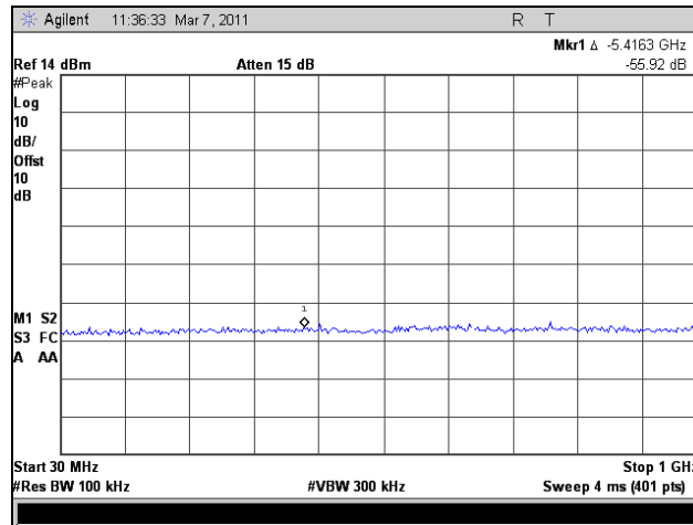
Plot 316. Conducted Spurious Emissions, Mid Channel, 30 MHz – 1 GHz, 802.11n HT30, Port 1
