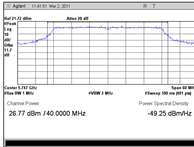
Plot 136. Peak Power Output, Low Channel, 802.11n HT40, Port 2
