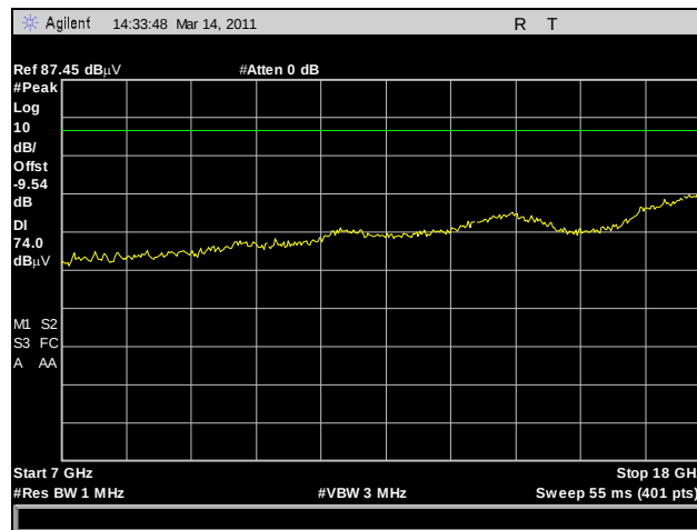
Plot 212. Radiated Harmonics, Low Channel, 7 GHz – 18 GHz, Peak, 802.11n HT20
