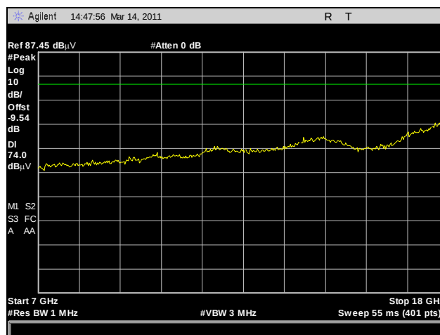
Plot 216. Radiated Harmonics, High Channel, 7 GHz – 18 GHz, Peak, 802.11n HT20
