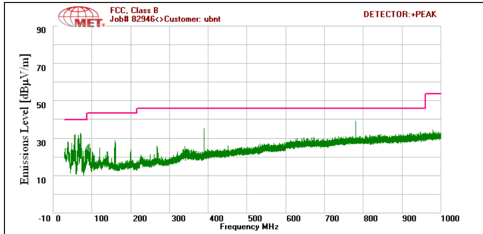
Plot 139. Radiated Spurious Emissions, 802.11a 20 MHz, Low Channel, 30 MHz – 1 GHz
