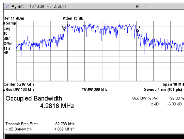
Plot 62. 99% Occupied Bandwidth, Mid Channel, 802.11n HT5, Port 1
