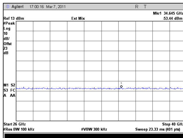
Plot 300. Conducted Spurious Emissions, Mid Channel, 26 GHz – 40 GHz, 802.11n HT20, Port 1
