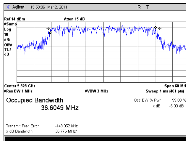
Plot 96. 99% Occupied Bandwidth, High Channel, 802.11n HT40, Port 2
