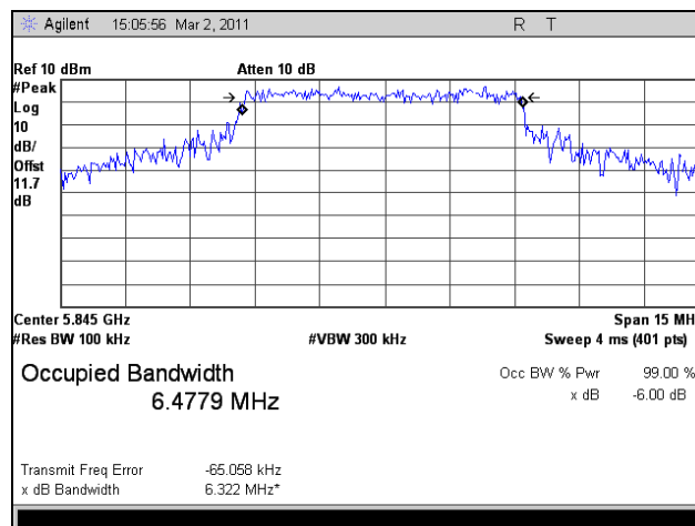
Plot 30. 6 dB Occupied Bandwidth, High Channel, 802.11n HT8, Port 2
