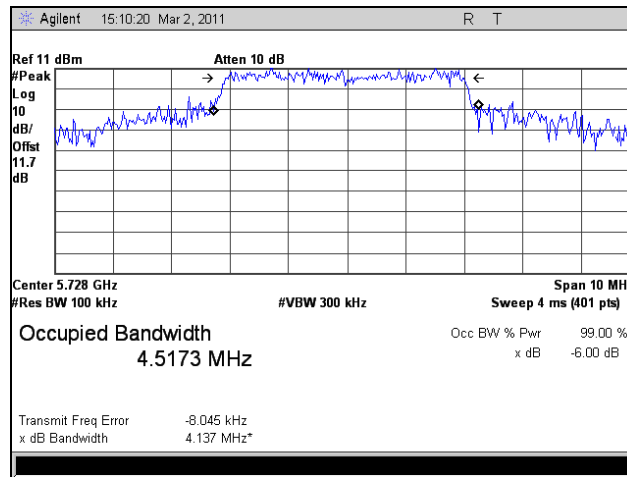
Plot 19. 6 dB Occupied Bandwidth, Low Channel, 802.11n HT5, Port 1
