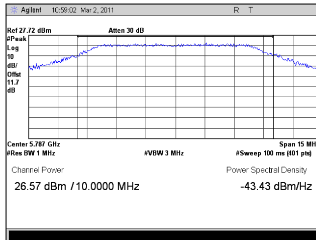
Plot 119. Peak Power Output, Mid Channel, 802.11n HT10, Port 2
