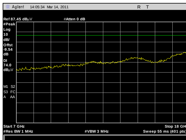
Plot 228. Radiated Harmonics, High Channel, 7 GHz – 18 GHz, Peak, 802.11n HT40
