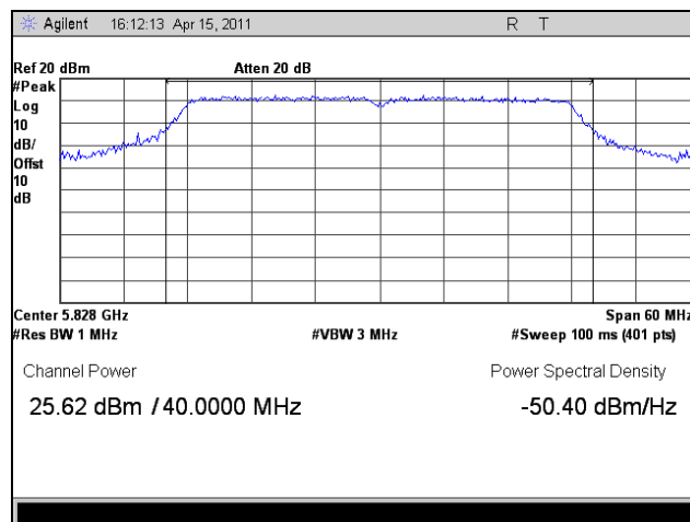
Plot 102. Peak Power Output, 802.11a 40 MHz, High Channel
