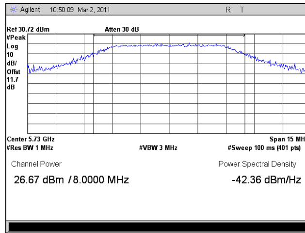
Plot 112. Peak Power Output, Low Channel, 802.11n HT8, Port 2
