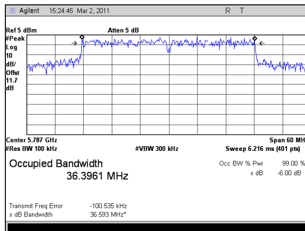
Plot 50. 6 dB Occupied Bandwidth, Mid Channel, 802.11n HT40, Port 1
