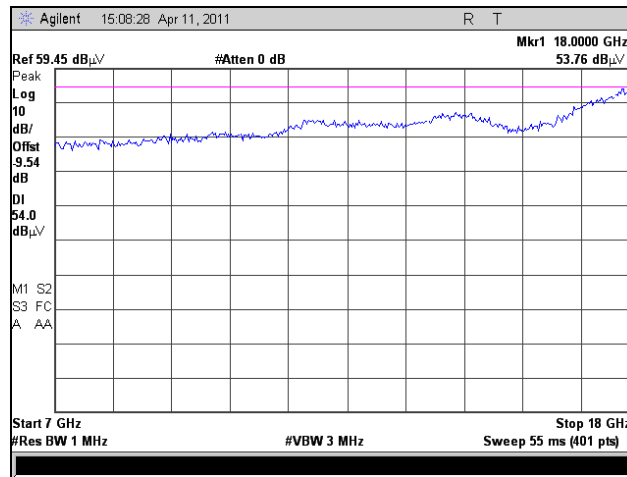
Plot 187. Radiated Harmonics, Low Channel, 802.11a 20 MHz, 7 GHz – 18 GHz
