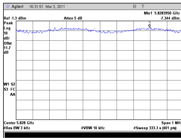
Plot 412. Peak Power Spectral Density, High Channel, 802.11n HT30, Port 2
