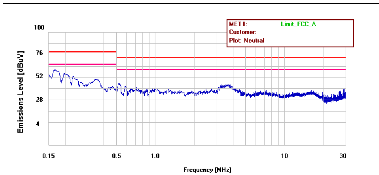
Plot 2. Conducted Emission, Neutral Line Plot, Cetus PSU
