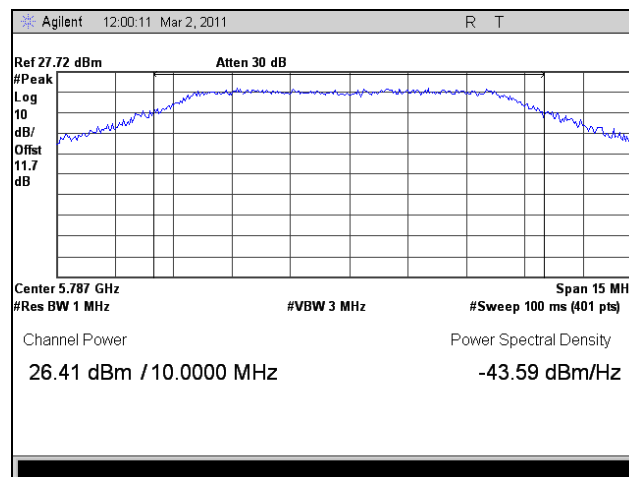
Plot 116. Peak Power Output, Mid Channel, 802.11n HT10, Port 1
