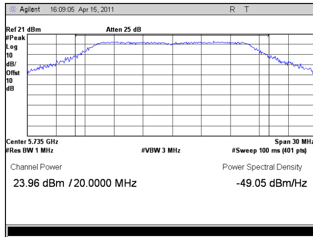
Plot 97. Peak Power Output, 802.11a 20 MHz, Low Channel
