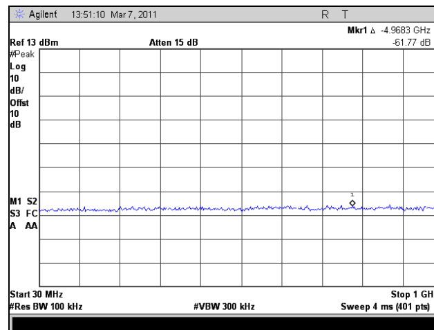
Plot 286. Conducted Spurious Emissions, Low Channel, 30 MHz – 1 GHz, 802.11n HT10, Port 2
