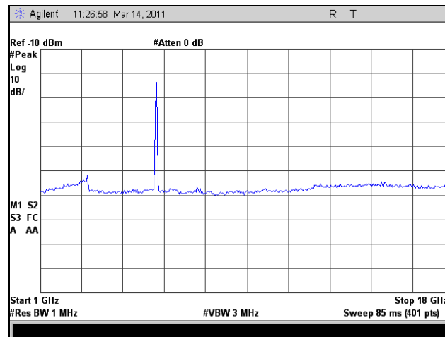
Plot 182. Radiated Spurious Emissions, Low Channel, 1 GHz – 18 GHz, 802.11n HT40
