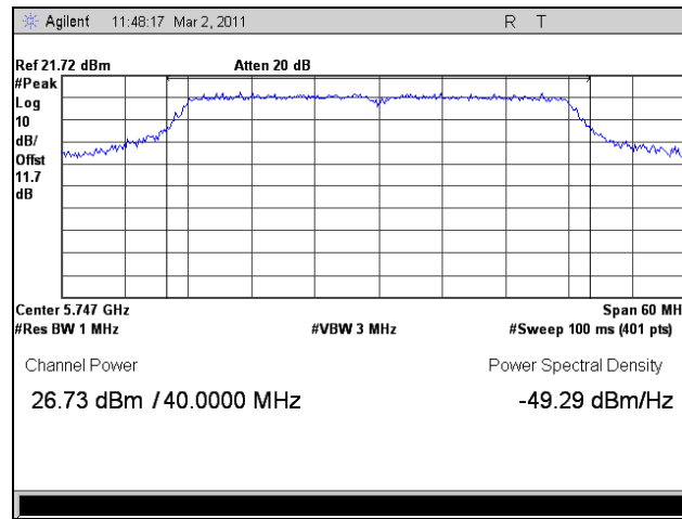
Plot 133. Peak Power Output, Low Channel, 802.11n HT40, Port 1
