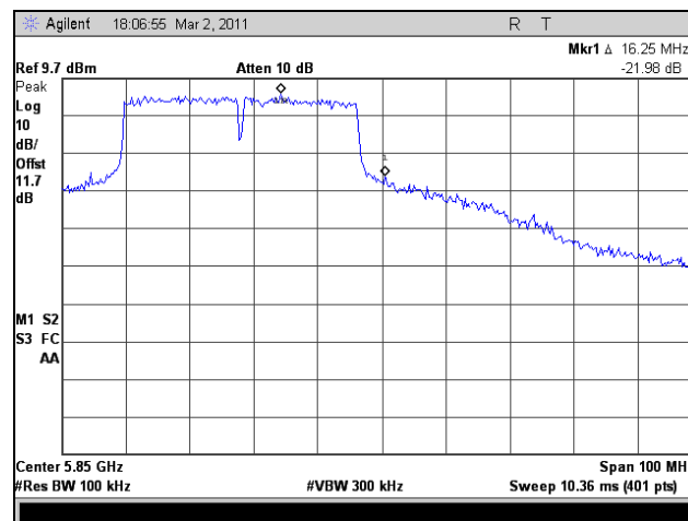
Plot 376. Conducted Band Edge, High Channel, 802.11n HT40, Port 2
