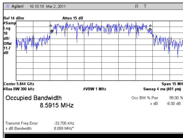
Plot 75. 99% Occupied Bandwidth, High Channel, 802.11n HT10, Port 1
