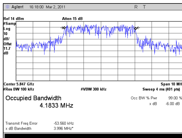
Plot 63. 99% Occupied Bandwidth, High Channel, 802.11n HT5, Port 1
