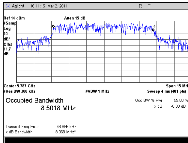
Plot 77. 99% Occupied Bandwidth, Mid Channel, 802.11n HT10, Port 2
