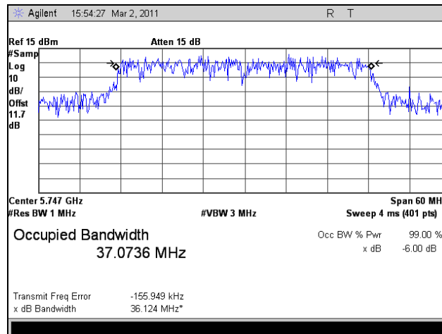
Plot 91. 99% Occupied Bandwidth, Low Channel, 802.11n HT40, Port 1
