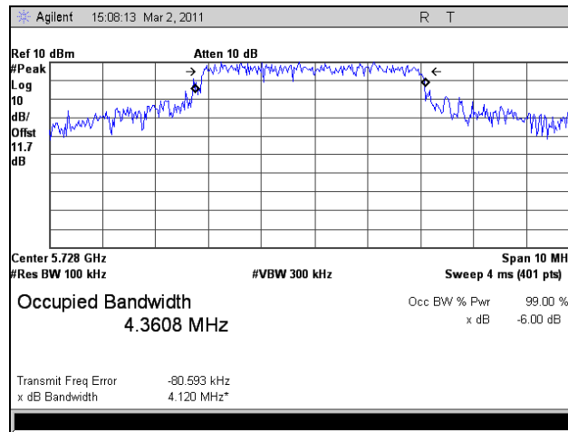
Plot 22. 6 dB Occupied Bandwidth, Low Channel, 802.11n HT5, Port 2
