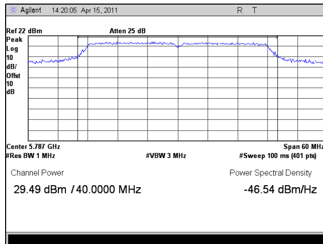
Plot 101. Peak Power Output, 802.11a 40 MHz, Mid Channel
