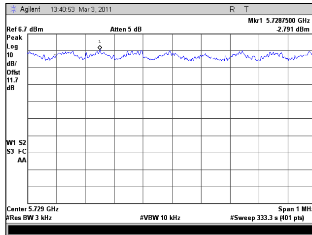
Plot 389. Peak Power Spectral Density, Low Channel, 802.11n HT8, Port 1
