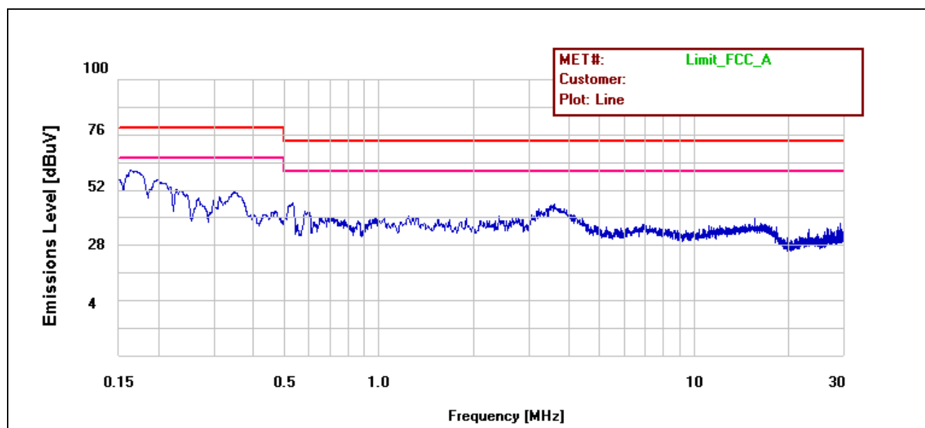
Plot 1. Conducted Emission, Phase Line Plot, Cetus PSU
