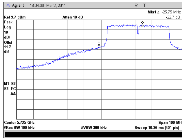
Plot 373. Conducted Band Edge, Low Channel, 802.11n HT40, Port 1
