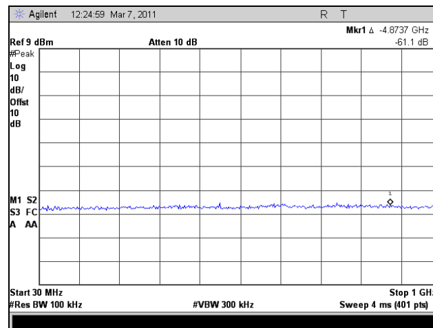
Plot 322. Conducted Spurious Emissions, Low Channel, 30 MHz – 1 GHz, 802.11n HT30, Port 2
