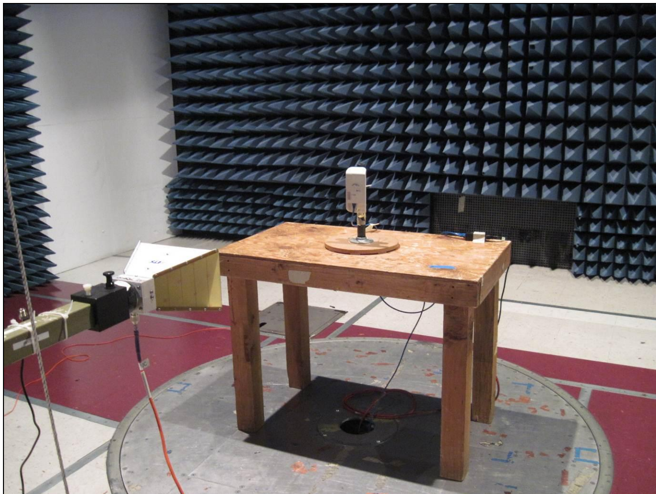
Photograph 6. Radiated Harmonics Emissions, Test Setup
