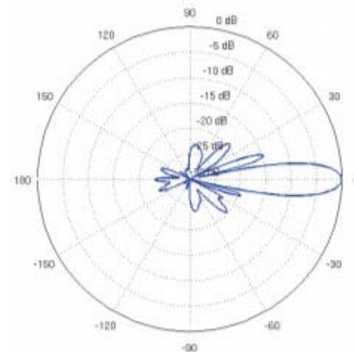
Horizontal Elevation
