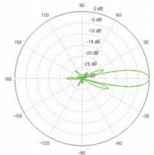
Horizontal Azimuth
