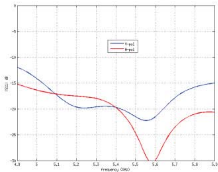
Return Loss
