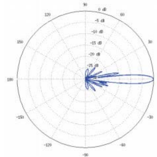
Horizontal Elevation
