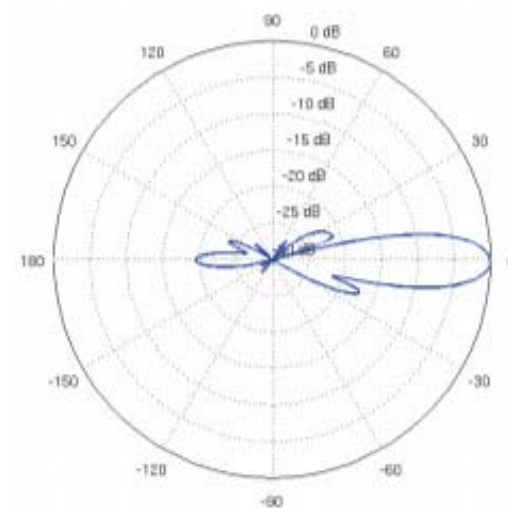
Vertical Elevation
