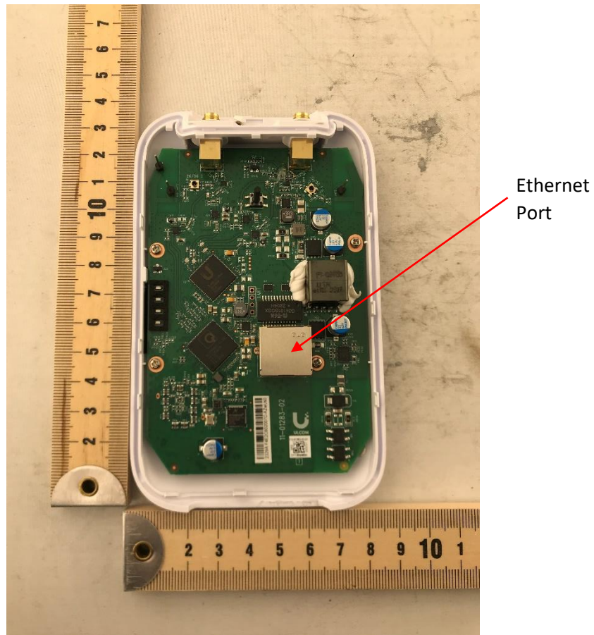
Photograph 1: Internal View of DUT With Front Cover Off
