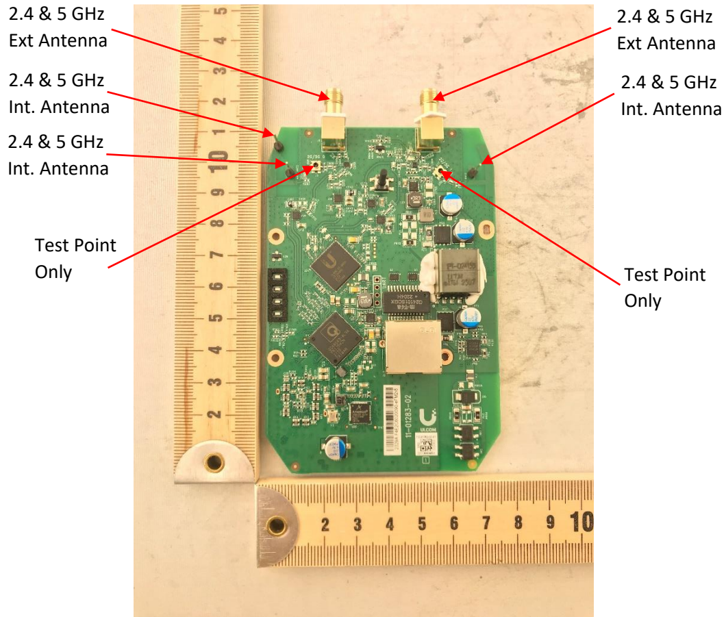
Photograph 2: Internal View of Top PCB
