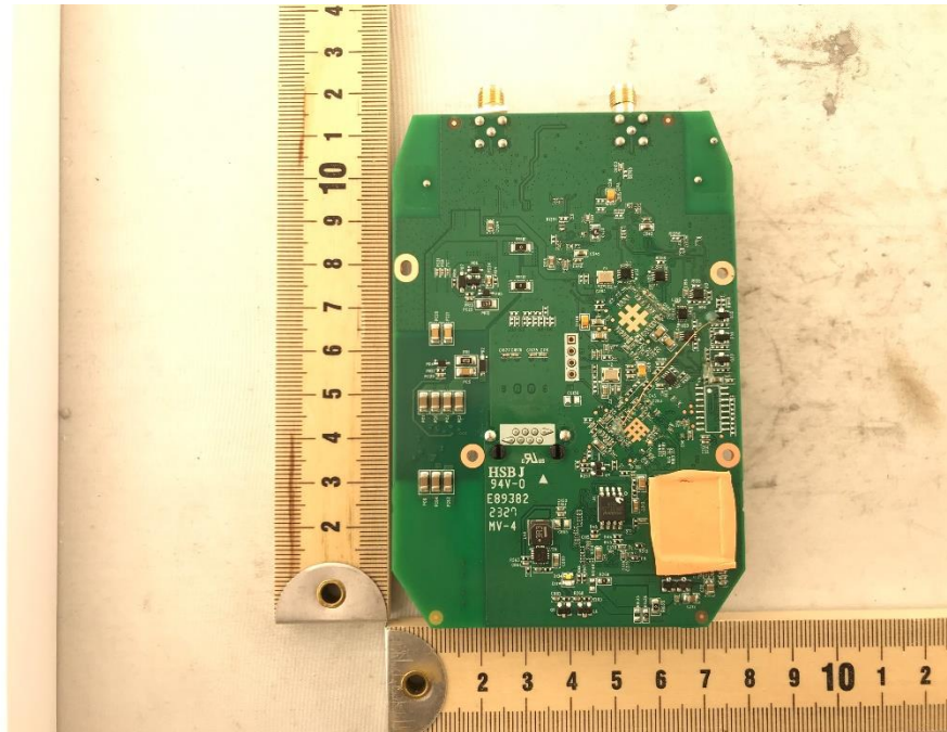
Photograph 3: Internal View of Bottom PCB
