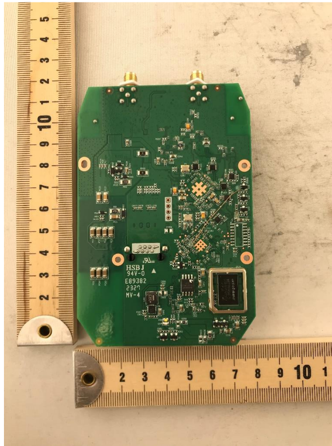
Photograph 4: Internal View of Bottom PCB With Can Off
