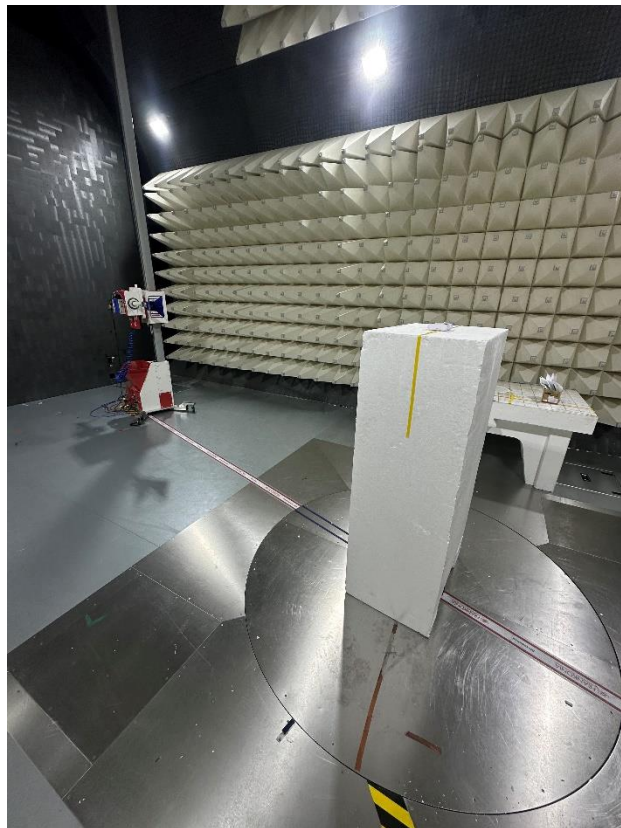
Photograph 2: View Test Set Up Radiated Emissions 1 – 17 GHz
