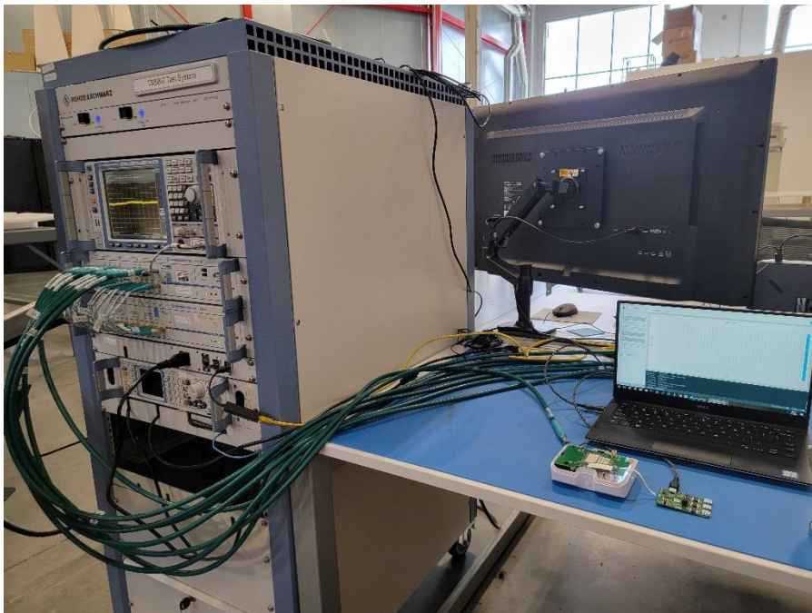
Photograph 4: View Test Set Up RF Conducted
