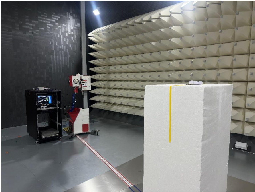
Photograph 3: View Test Set Up Radiated Emissions 17 – 26 GHz
