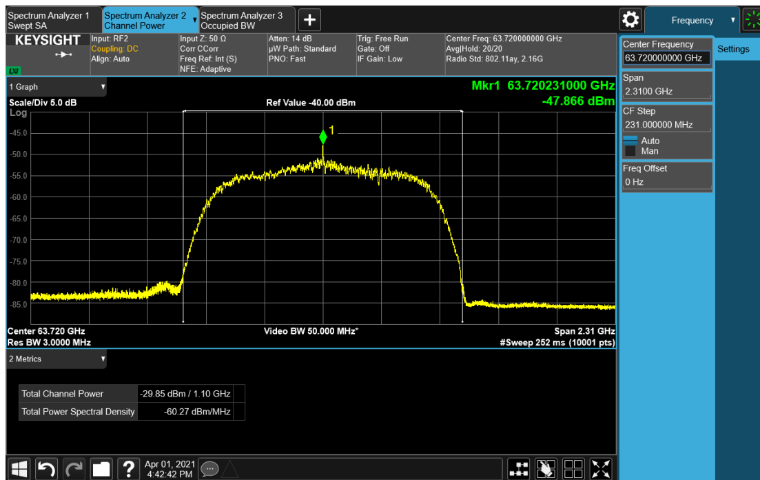
Wave-AP_1GHz_63.72GHz_AVG Power
