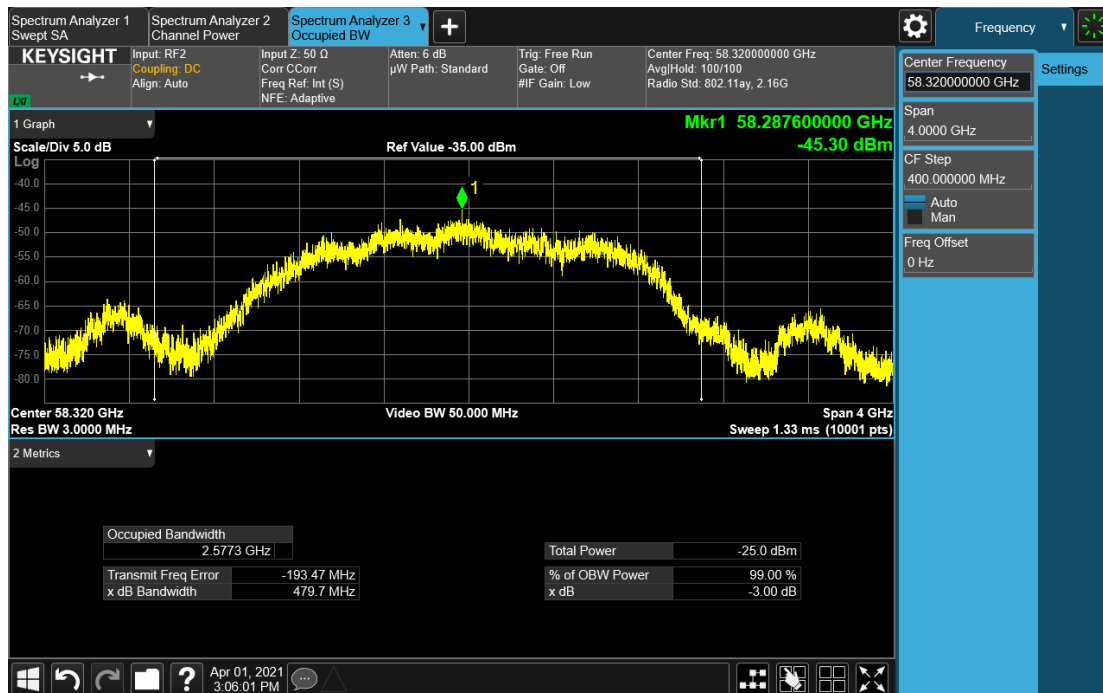
Wave-AP_2GHz_58.32GHz_Peak
