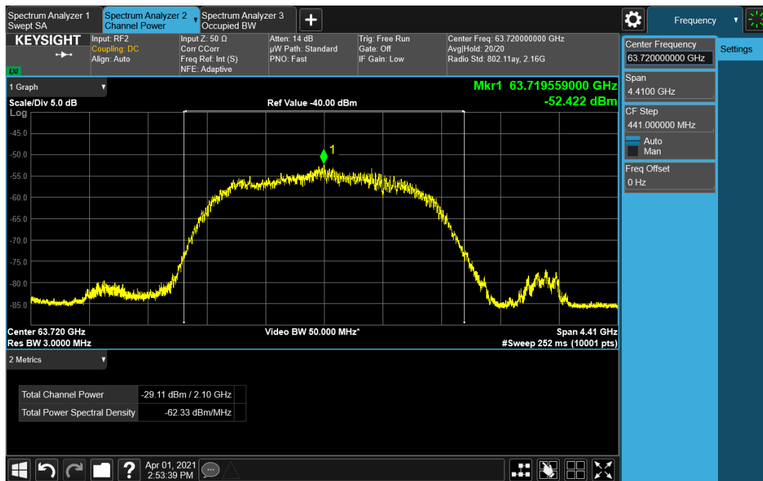
Wave-AP_2GHz_63.72GHz_Average Power
