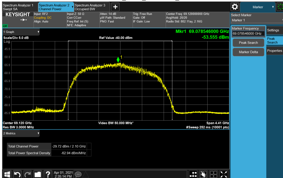
Wave-AP_2GHz_69.12GHz_Average Power
