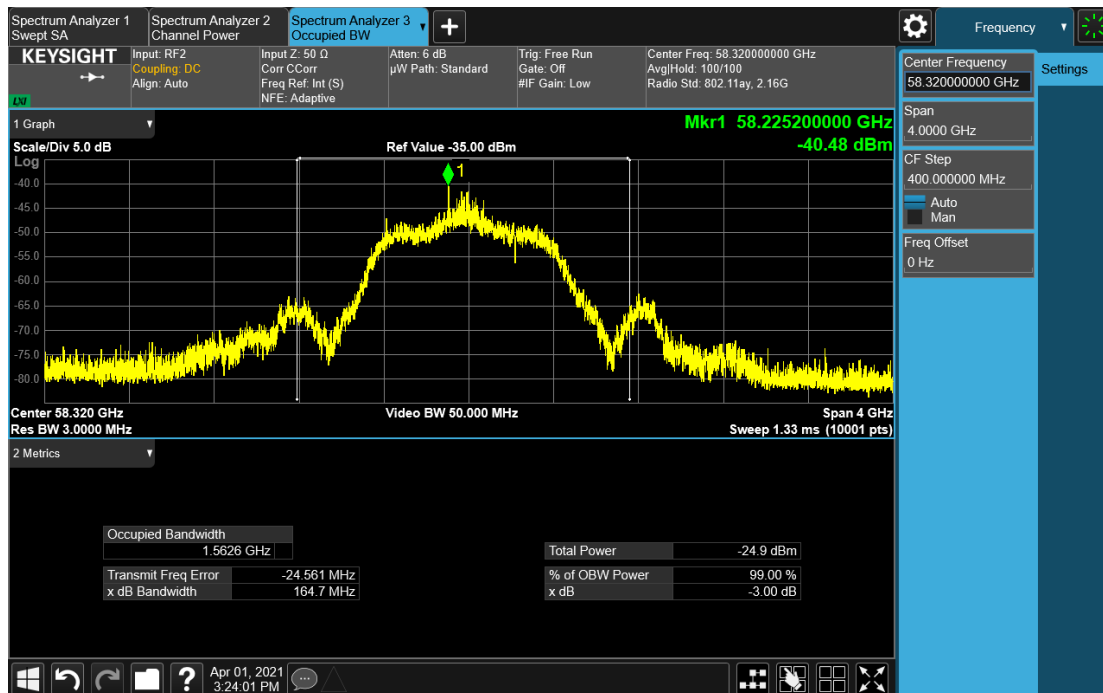
Wave-AP_1GHz_58.32GHz_Peak
