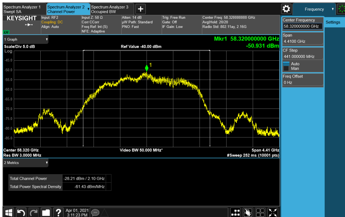
Wave-AP_2GHz_58.32GHz_AVG Power
