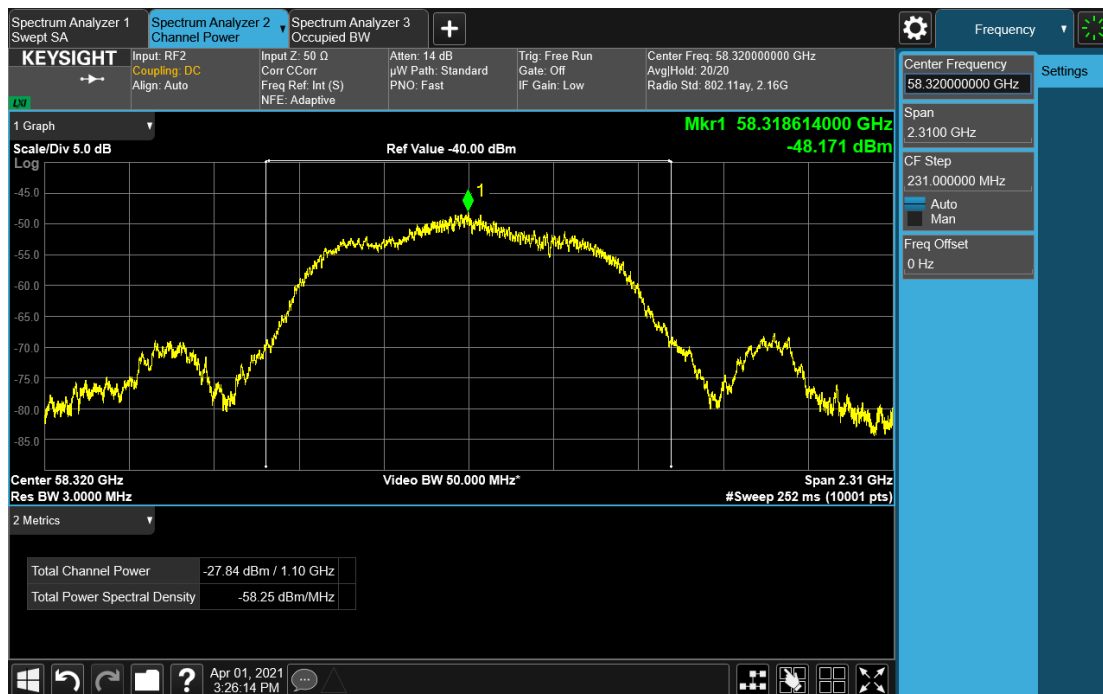
Wave-AP_1GHz_58.32GHz_AVG Power
