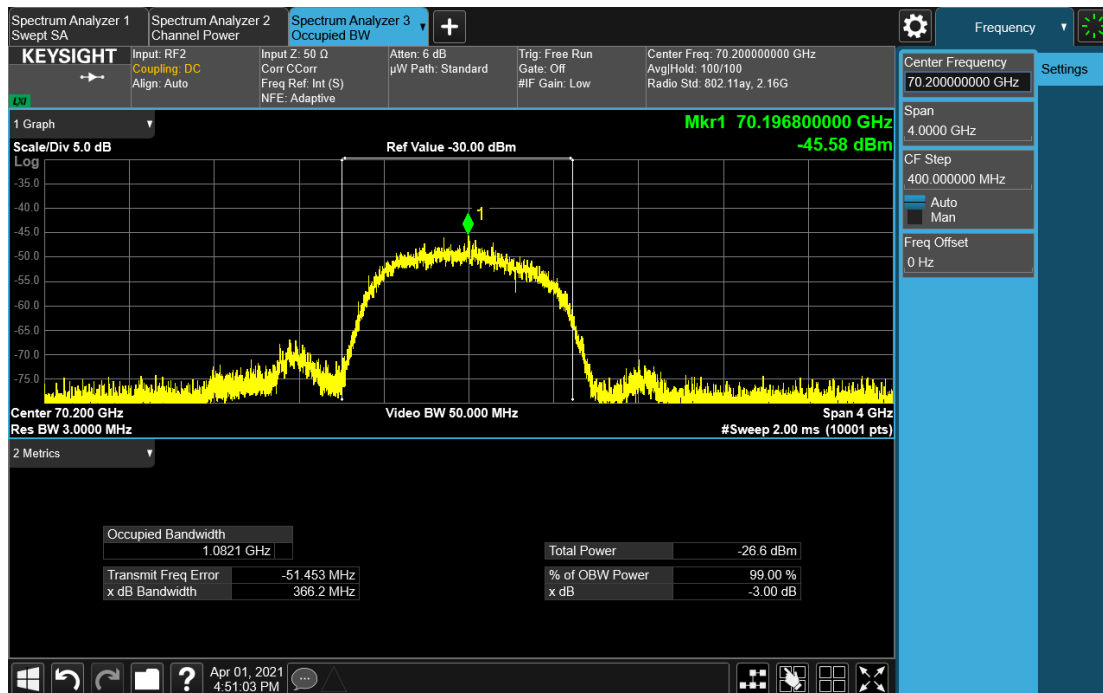
Wave-AP_1GHz_70.2GHz_Peak
