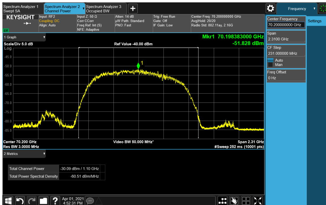
Wave-AP_1GHz_70.2GHz_AVG Power
