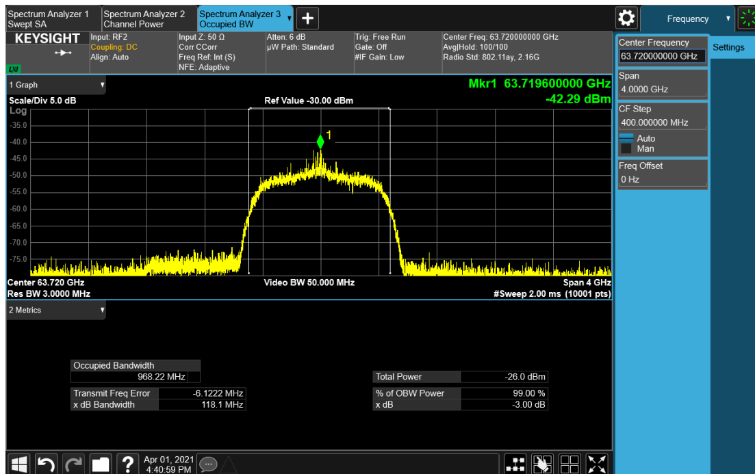
Wave-AP_1GHz_63.72GHz_Peak
