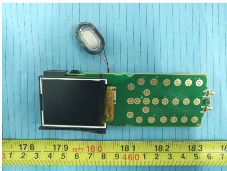
EUT – Main Board Top Cover off View 1
