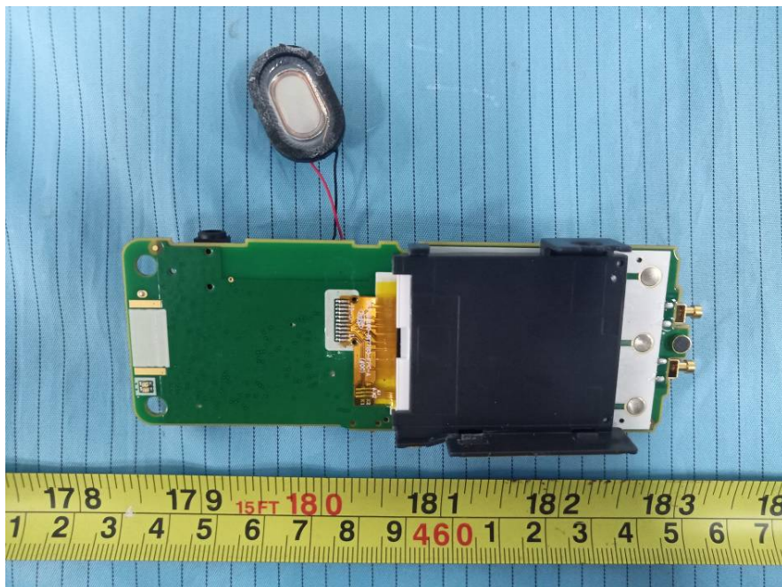
EUT – Main Board Top Cover off View 2
