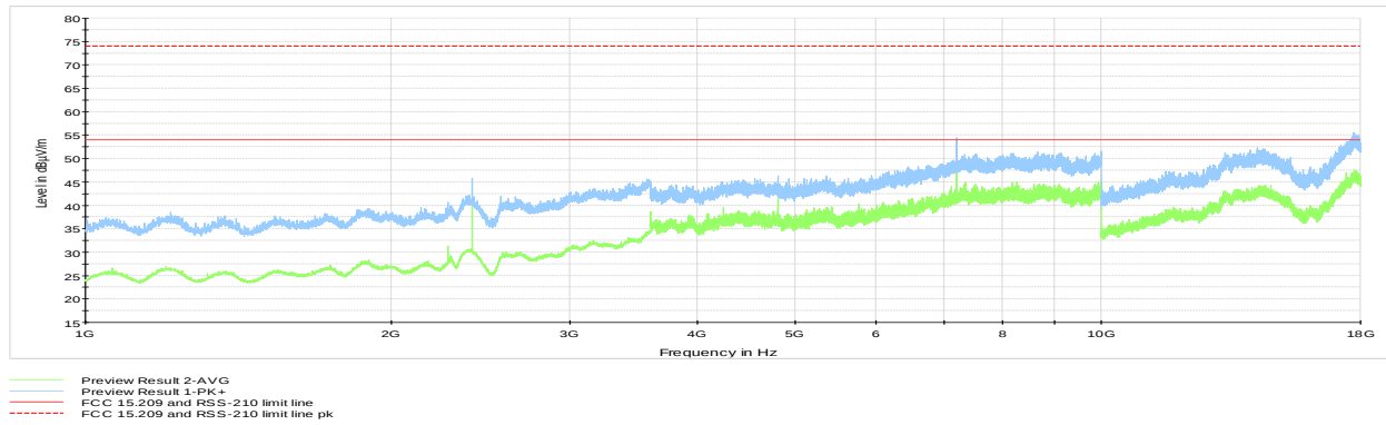
Figure 8.6-9: Radiated spurious emissions 1 to 18 GHz, Low channel
