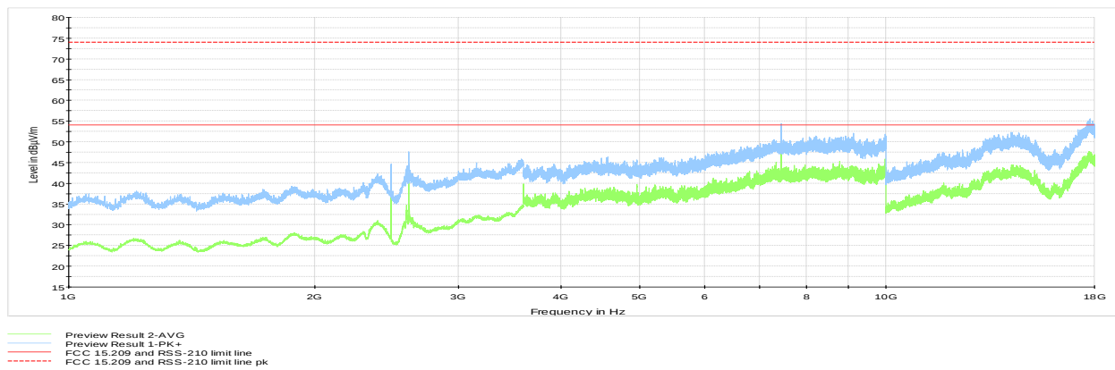
Figure 8.6-11: Radiated spurious emissions 1 to 18 GHz, High channel
