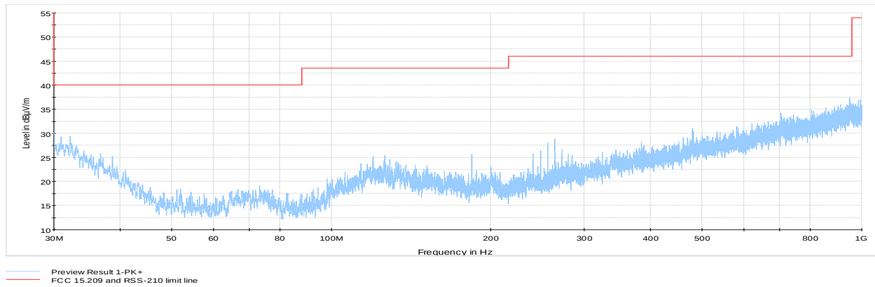
Figure 8.6-7: Radiated spurious emissions 30 MHz to 1 GHz, mid channel
