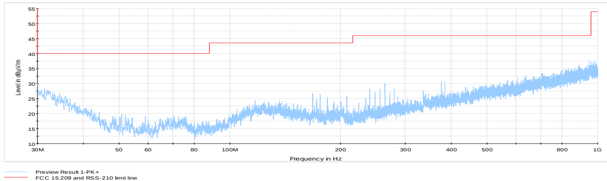
Figure 8.6-8: Radiated spurious emissions 30 MHz to 1 GHz, High channel
