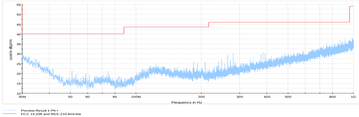
Figure 8.6-6: Radiated spurious emissions 30 MHz to 1 GHz, Low channel
