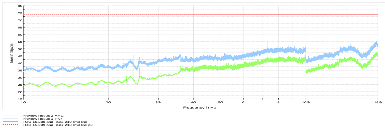
Figure 8.6-10: Radiated spurious emissions 1 to 18 GHz, mid channel
