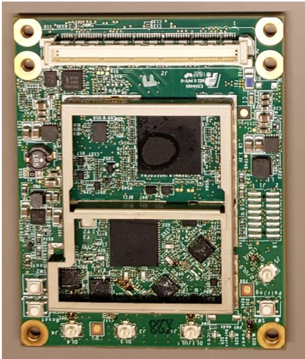
Figure 1- AMN41012 – Top View without shields
