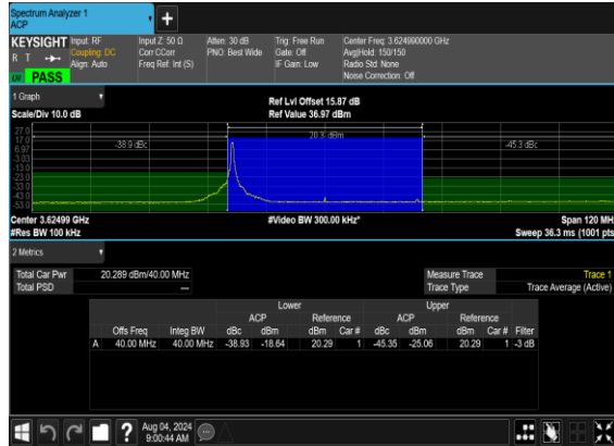
N48(40M)_DFT-s-OFDM_PI_2-BPSK_Edge_1RB_Left_Mid_CH
