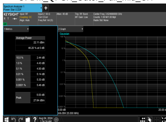
N48(20M)_DFT-s- OFDM_QPSK_Outer_Full_Mid_CH
