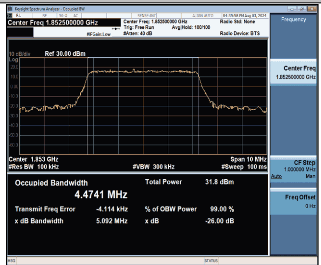
Band25-5MHz-16QAM-26065-25RB#0-PASS
