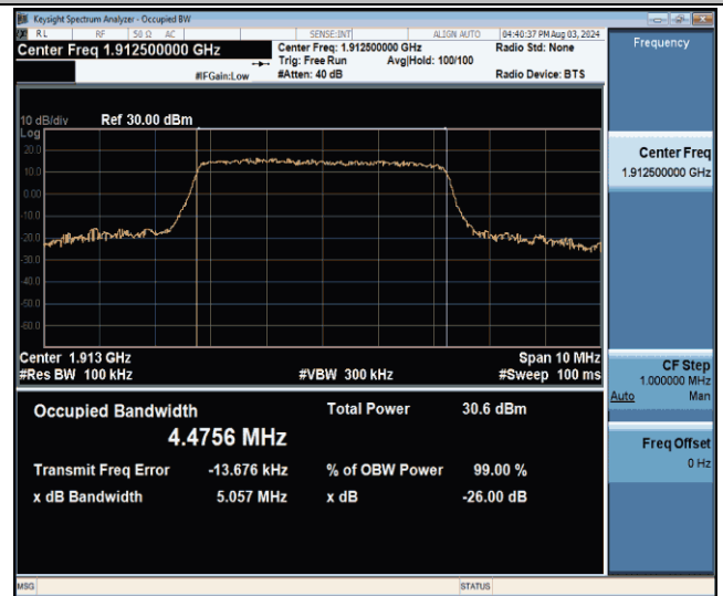
Band25-5MHz-16QAM-26665-25RB#0-PASS
