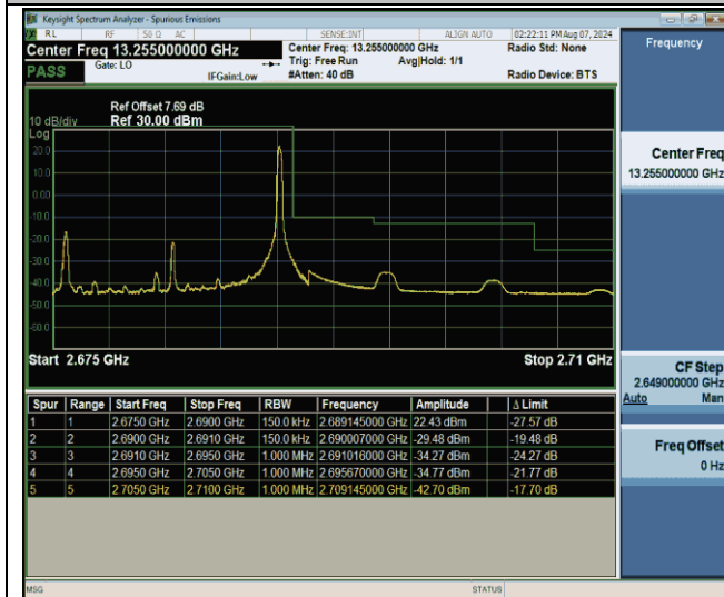
Band41_15MHz_QPSK_41515_1RB#74
