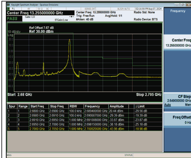
Band41_10MHz_QPSK_41540_1RB#49
