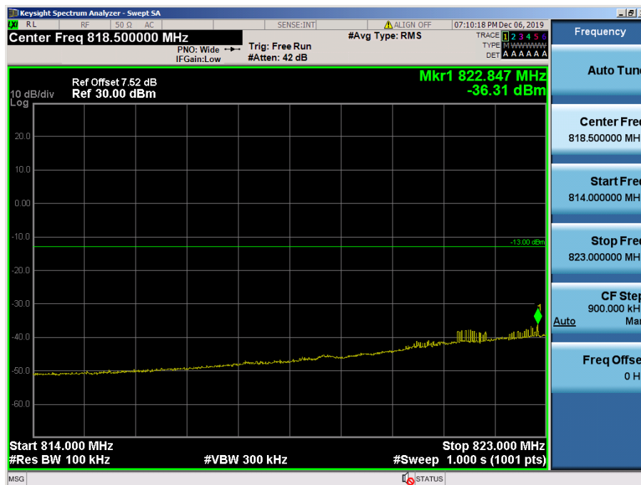
LTE Band 5 / 10MHz / 64QAM - RB Size/Offset (25/0)
