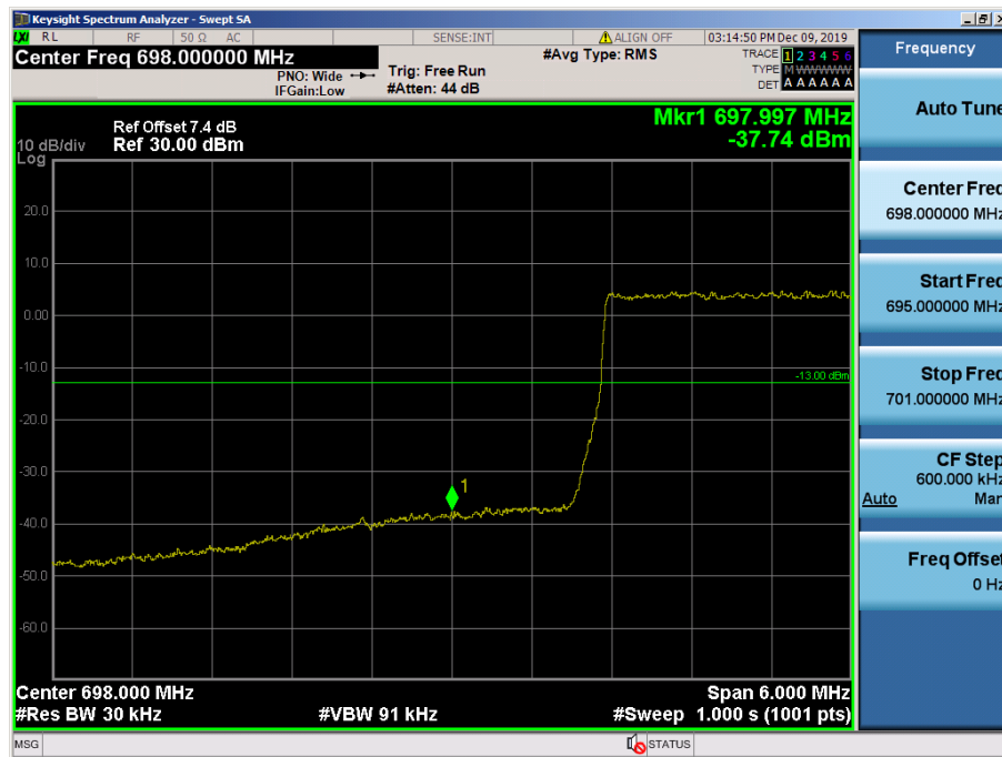
LTE Band 12 / 3MHz / 64QAM - RB Size/Offset (15/0)
