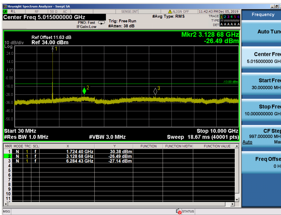
LTE Band 4 / 15MHz / 64QAM - RB Size/Offset (1/74)–Low Channel
